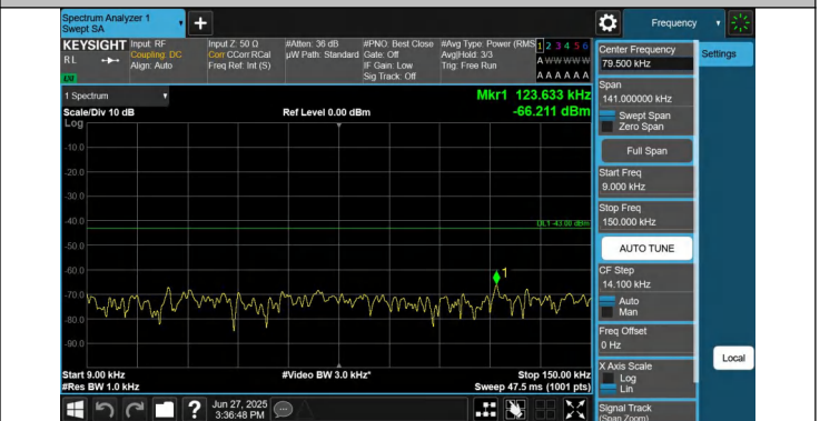
66-66-15MHz-15MHz-QPSK-QPSK-132347-132497-1RB#74-0RB#0-0.009~0.15MHz-PASS
