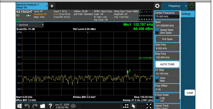
66-66-15MHz-20MHz-QPSK-QPSK-132325-132496-1RB#0-1RB #99-0.009~0.15MHz-PASS
