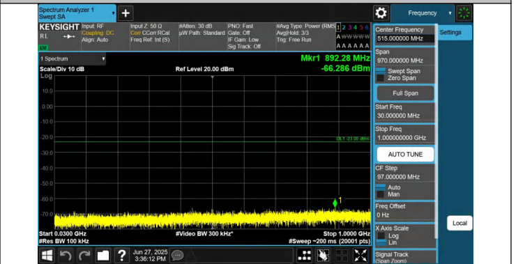
66-66-15MHz-15MHz-QPSK-QPSK-132347-132497-1RB#0-0RB #0-30~1000MHz-PASS
