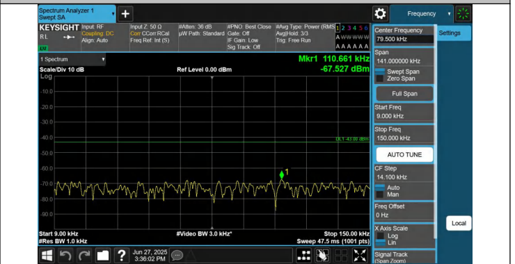
66-66-15MHz-15MHz-QPSK-QPSK-132347-132497-1RB#0-0RB #0-0.009~0.15MHz-PASS
