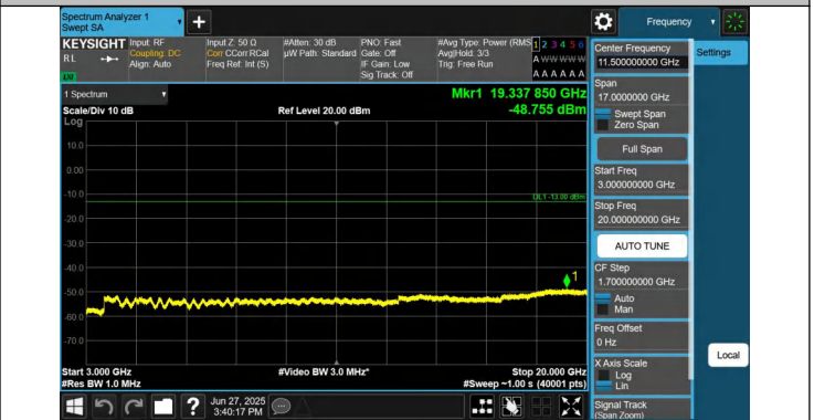
66-66-15MHz-15MHz-QPSK-QPSK-132447-132597-1RB#0-1RB #74-3000~20000MHz-PASS
