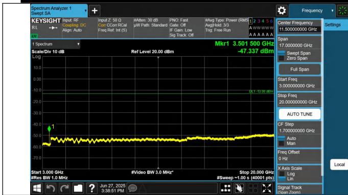
66-66-15MHz-15MHz-QPSK-QPSK-132447-132597-1RB#0-0RB #0-3000~20000MHz-PASS
