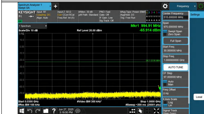
66-66-15MHz-10MHz-QPSK-QPSK-132499-132619-1RB#0-1RB #49-30~1000MHz-PASS
