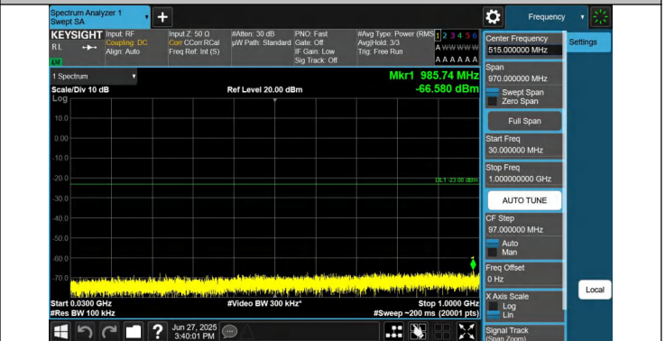
66-66-15MHz-15MHz-QPSK-QPSK-132447-132597-1RB#0-1RB #74-30~1000MHz-PASS
