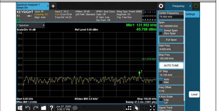
66-66-15MHz-15MHz-QPSK-QPSK-132047-132197-1RB#0-0RB #74-0.009~0.15MHz-PASS
