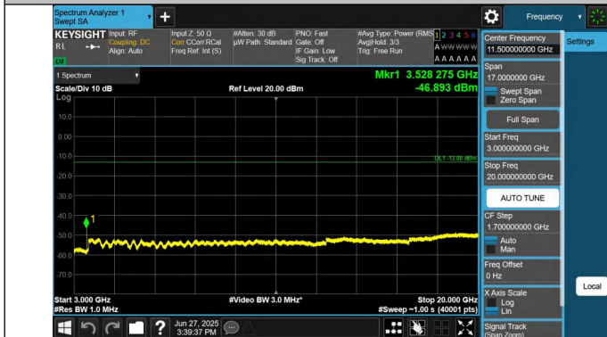
66-66-15MHz-15MHz-QPSK-QPSK-132447-132597-1RB#74-0R B#0-3000~20000MHz-PASS
