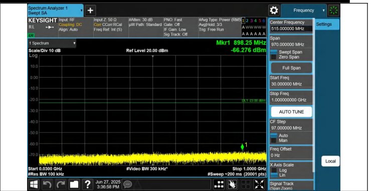
66-66-15MHz-15MHz-QPSK-QPSK-132347-132497-1RB#74-0R B#0-30~1000MHz-PASS
