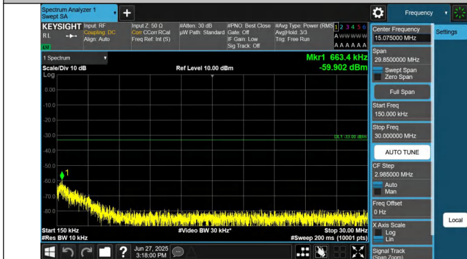
66-66-15MHz-10MHz-QPSK-QPSK-132499-132619-1RB#74-0R B#0-0.15~30MHz-PASS
