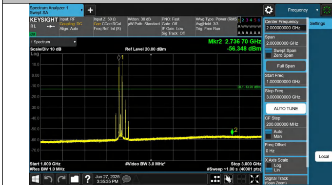
66-66-15MHz-15MHz-QPSK-QPSK-132047-132197-1RB#0-0RB #74-1000~3000MHz-PASS
