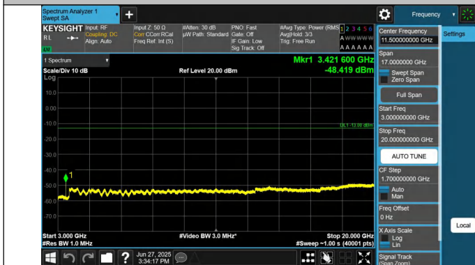
66-66-15MHz-15MHz-QPSK-QPSK-132047-132197-1RB#0-0RB #0-3000~20000MHz-PASS
