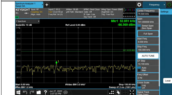
66-66-15MHz-15MHz-QPSK-QPSK-132347-132497-1RB#0-1RB #74-0.009~0.15MHz-PASS
