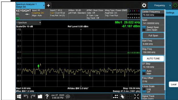
66-66-15MHz-20MHz-QPSK-QPSK-132050-132221-1RB#0-1RB #99-0.009~0.15MHz-PASS
