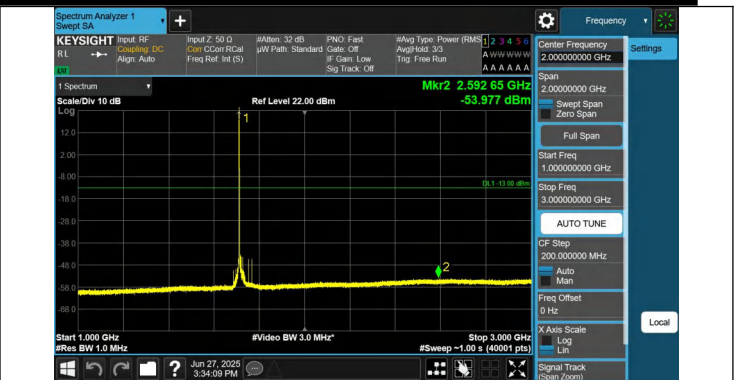
66-66-15MHz-15MHz-QPSK-QPSK-132047-132197-1RB#0-0RB #0-1000~3000MHz-PASS
