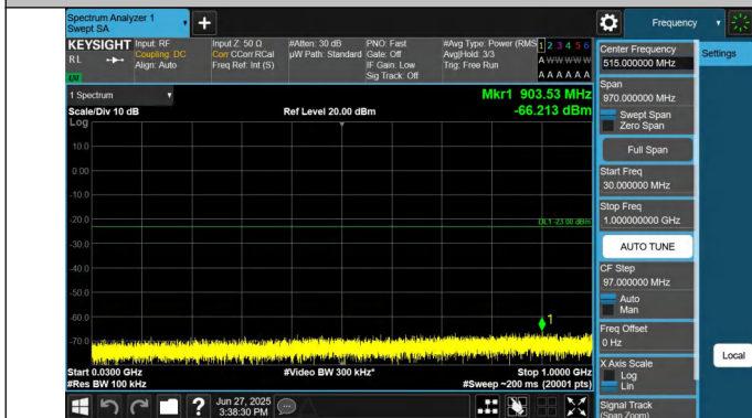
66-66-15MHz-15MHz-QPSK-QPSK-132447-132597-1RB#0-0RB #0-30~1000MHz-PASS
