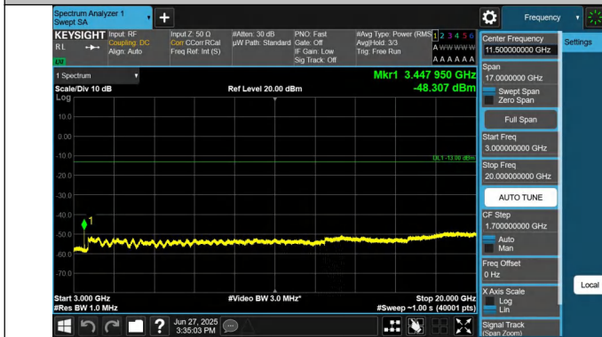
66-66-15MHz-15MHz-QPSK-QPSK-132047-132197-1RB#74-0R B#0-3000~20000MHz-PASS
