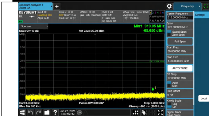
66-66-15MHz-15MHz-QPSK-QPSK-132447-132597-1RB#74-0R B#0-30~1000MHz-PASS
