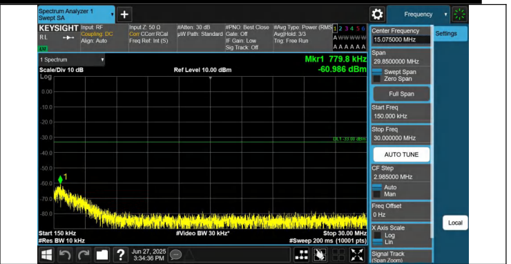
66-66-15MHz-15MHz-QPSK-QPSK-132047-132197-1RB#74-0R B#0-0.15~30MHz-PASS
