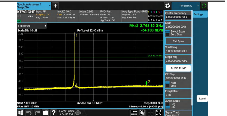
66-66-15MHz-15MHz-QPSK-QPSK-132047-132197-1RB#74-0R B#0-1000~3000MHz-PASS
