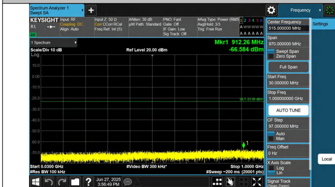
66-66-15MHz-20MHz-QPSK-QPSK-132050-132221-1RB#0-1RB #99-30~1000MHz-PASS
