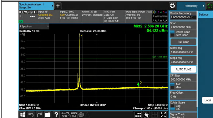
66-66-15MHz-15MHz-QPSK-QPSK-132347-132497-1RB#74-0R B#0-1000~3000MHz-PASS
