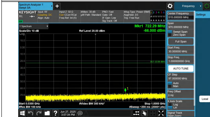
66-66-15MHz-20MHz-QPSK-QPSK-132325-132496-1RB#0-0RB #0-30~1000MHz-PASS
