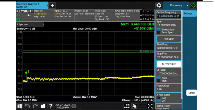
66-66-15MHz-20MHz-QPSK-QPSK-132050-132221-1RB#74-0R B#0-3000~20000MHz-PASS
