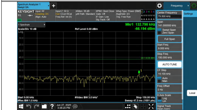
66-66-15MHz-15MHz-QPSK-QPSK-132447-132597-1RB#0-0RB #0-0.009~0.15MHz-PASS
