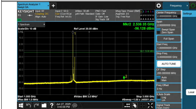
66-66-15MHz-15MHz-QPSK-QPSK-132447-132597-1RB#0-1RB #74-1000~3000MHz-PASS
