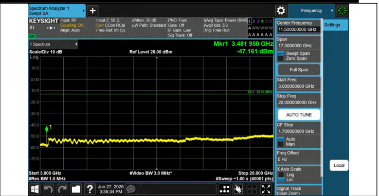
66-66-15MHz-15MHz-QPSK-QPSK-132347-132497-1RB#0-0RB #0-3000~20000MHz-PASS
