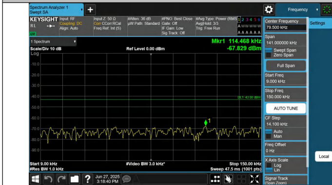
66-66-15MHz-10MHz-QPSK-QPSK-132499-132619-1RB#0-1RB #49-0.009~0.15MHz-PASS
