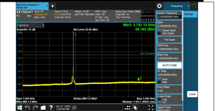
66-66-15MHz-15MHz-QPSK-QPSK-132447-132597-1RB#74-0R B#0-1000~3000MHz-PASS
