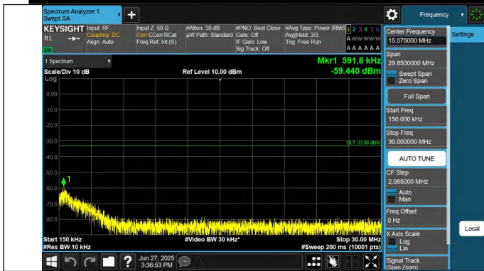
66-66-15MHz-15MHz-QPSK-QPSK-132347-132497-1RB#74-0R B#0-0.15~30MHz-PASS
