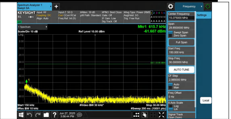
66-66-15MHz-20MHz-QPSK-QPSK-132050-132221-1RB#0-1RB #99-0.15~30MHz-PASS
