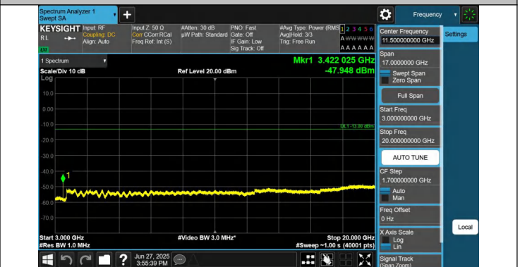
66-66-15MHz-20MHz-QPSK-QPSK-132050-132221-1RB#0-0RB #0-3000~20000MHz-PASS
