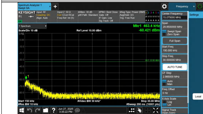
66-66-15MHz-15MHz-QPSK-QPSK-132047-132197-1RB#0-0RB #74-0.15~30MHz-PASS
