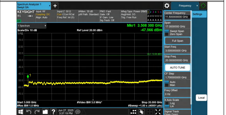
66-66-15MHz-15MHz-QPSK-QPSK-132347-132497-1RB#74-0R B#0-3000~20000MHz-PASS
