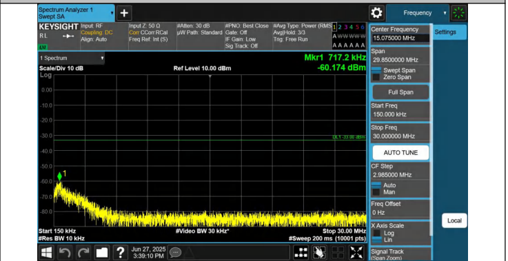
66-66-15MHz-15MHz-QPSK-QPSK-132447-132597-1RB#74-0R B#0-0.15~30MHz-PASS
