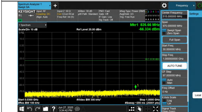
66-66-15MHz-15MHz-QPSK-QPSK-132047-132197-1RB#74-0R B#0-30~1000MHz-PASS
