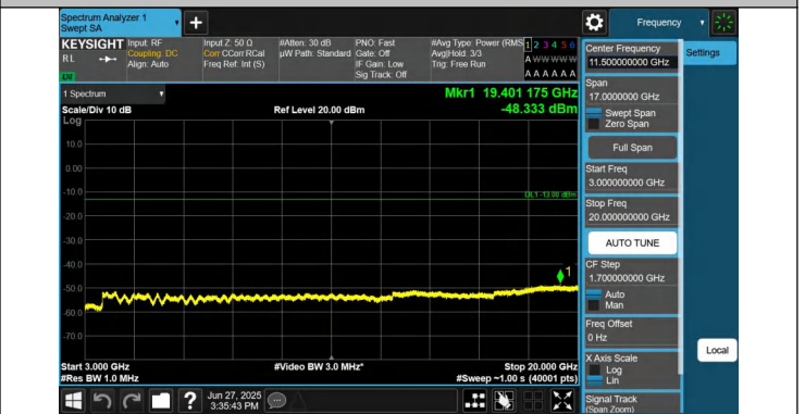
66-66-15MHz-15MHz-QPSK-QPSK-132047-132197-1RB#0-0RB #74-3000~20000MHz-PASS
