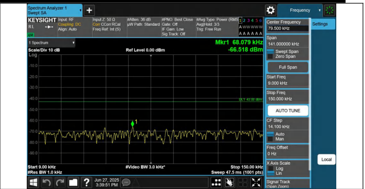
66-66-15MHz-15MHz-QPSK-QPSK-132447-132597-1RB#0-1RB #74-0.009~0.15MHz-PASS
