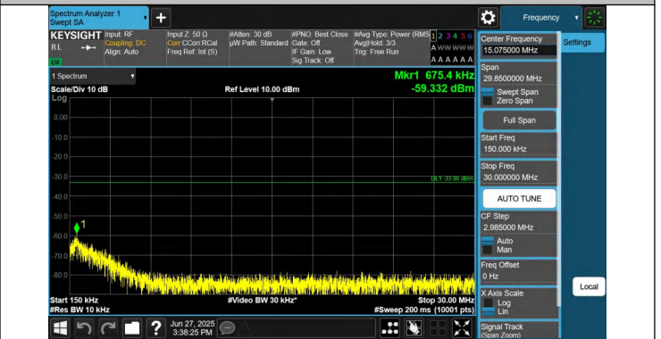
66-66-15MHz-15MHz-QPSK-QPSK-132447-132597-1RB#0-0RB #0-0.15~30MHz-PASS
