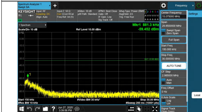
66-66-15MHz-15MHz-QPSK-QPSK-132447-132597-1RB#0-1RB #74-0.15~30MHz-PASS
