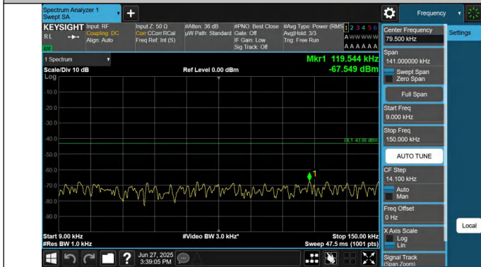
66-66-15MHz-15MHz-QPSK-QPSK-132447-132597-1RB#74-0R B#0-0.009~0.15MHz-PASS
