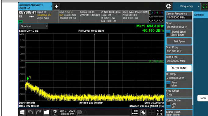
66-66-15MHz-20MHz-QPSK-QPSK-132050-132221-1RB#74-0R B#0-0.15~30MHz-PASS
