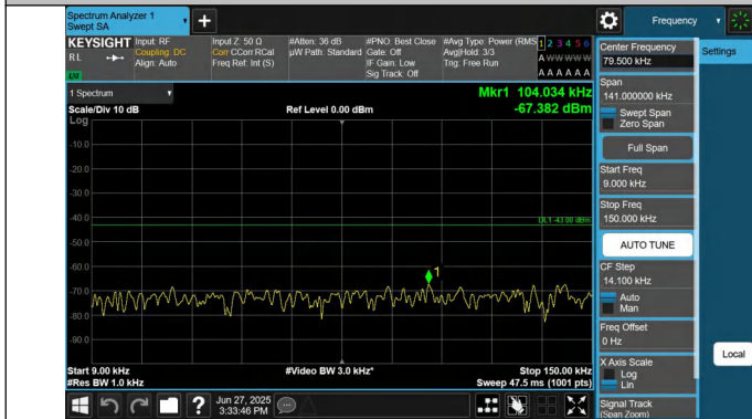
66-66-15MHz-15MHz-QPSK-QPSK-132047-132197-1RB#0-0RB #0-0.009~0.15MHz-PASS
