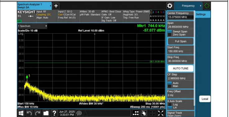
66-66-15MHz-15MHz-QPSK-QPSK-132047-132197-1RB#0-0RB #0-0.15~30MHz-PASS
