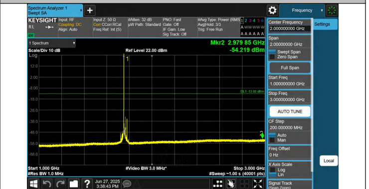
66-66-15MHz-15MHz-QPSK-QPSK-132447-132597-1RB#0-0RB #0-1000~3000MHz-PASS
