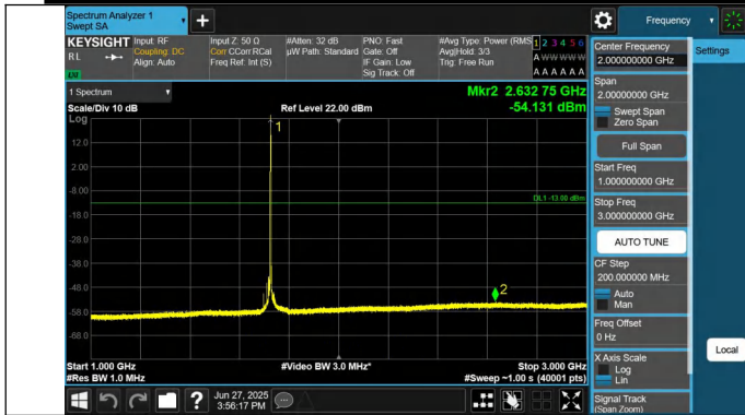
66-66-15MHz-20MHz-QPSK-QPSK-132050-132221-1RB#74-0R B#0-1000~3000MHz-PASS
