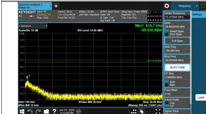
66-66-15MHz-10MHz-QPSK-QPSK-132047-132167-1RB#74-0R B#0-0.15~30MHz-PASS
