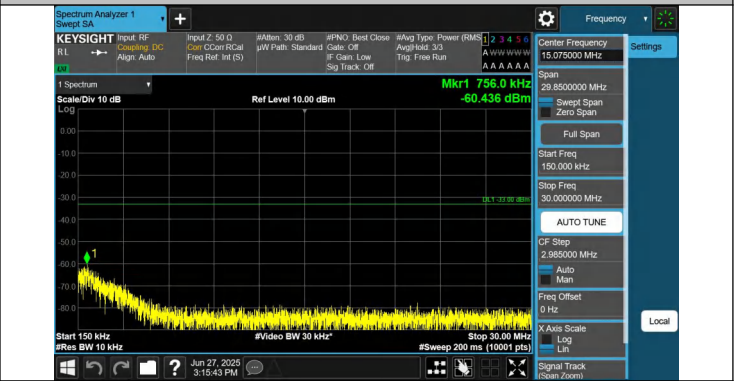
66-66-15MHz-10MHz-QPSK-QPSK-132373-132493-1RB#74-0R B#0-0.15~30MHz-PASS
