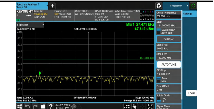
66-66-15MHz-10MHz-QPSK-QPSK-132373-132493-1RB#0-1RB #49-0.009~0.15MHz-PASS
