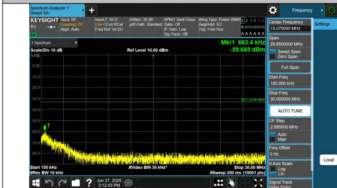
66-66-15MHz-10MHz-QPSK-QPSK-132047-132167-1RB#0-0RB #0-0.15~30MHz-PASS
