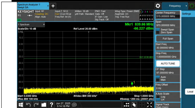
66-66-15MHz-10MHz-QPSK-QPSK-132047-132167-1RB#0-1RB #49-30~1000MHz-PASS
