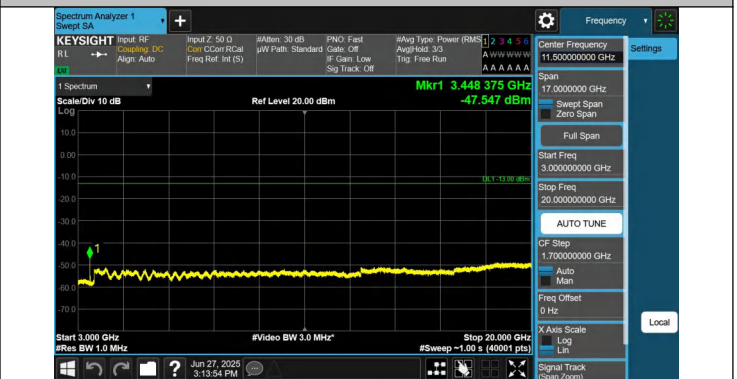
66-66-15MHz-10MHz-QPSK-QPSK-132047-132167-1RB#74-0R B#0-3000~20000MHz-PASS
