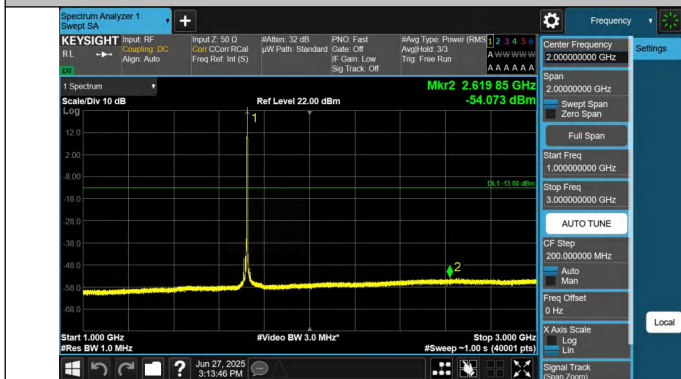
66-66-15MHz-10MHz-QPSK-QPSK-132047-132167-1RB#74-0R B#0-1000~3000MHz-PASS
