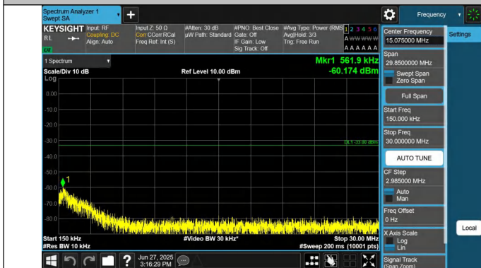
66-66-15MHz-10MHz-QPSK-QPSK-132373-132493-1RB#0-1RB #49-0.15~30MHz-PASS
