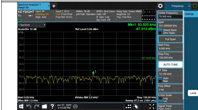
66-66-15MHz-10MHz-QPSK-QPSK-132047-132167-1RB#0-1RB #49-0.009~0.15MHz-PASS
