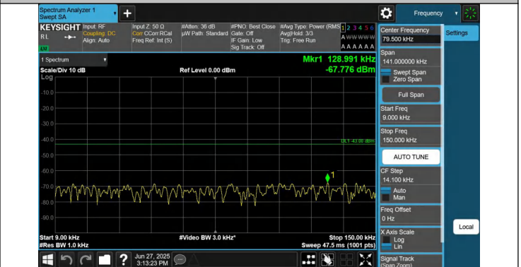
66-66-15MHz-10MHz-QPSK-QPSK-132047-132167-1RB#74-0R B#0-0.009~0.15MHz-PASS
