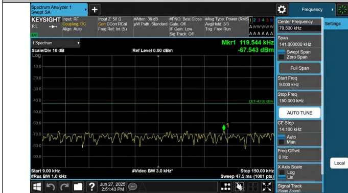
66-66-10MHz-20MHz-QPSK-QPSK-132027-132171-1RB#49-0R B#0-0.009~0.15MHz-PASS
