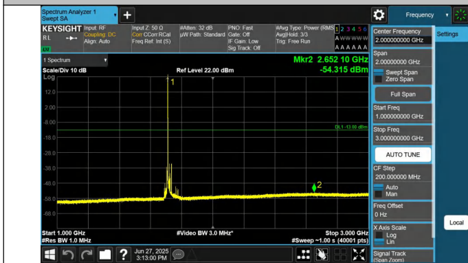
66-66-15MHz-10MHz-QPSK-QPSK-132047-132167-1RB#0-0RB #0-1000~3000MHz-PASS
