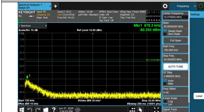
66-66-10MHz-20MHz-QPSK-QPSK-132328-132472-1RB#49-0R B#0-0.15~30MHz-PASS
