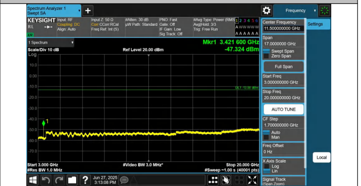
66-66-15MHz-10MHz-QPSK-QPSK-132047-132167-1RB#0-0RB #0-3000~20000MHz-PASS
