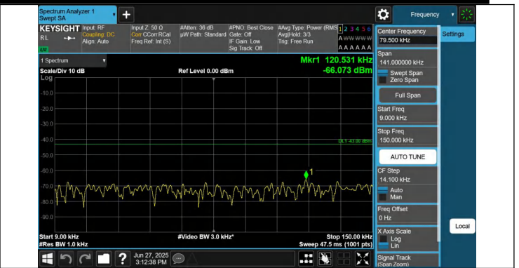
66-66-15MHz-10MHz-QPSK-QPSK-132047-132167-1RB#0-0RB #0-0.009~0.15MHz-PASS
