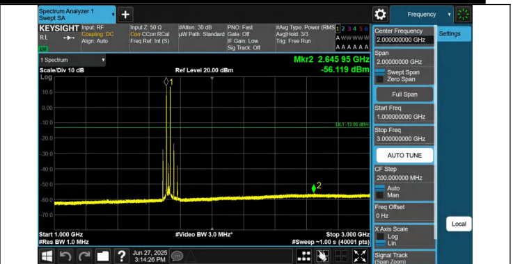
66-66-15MHz-10MHz-QPSK-QPSK-132047-132167-1RB#0-1RB #49-1000~3000MHz-PASS
