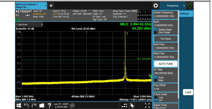
41-41-20MHz-15MHz-QPSK-QPSK-40546-40717-1RB#99-0RB#0 -1000~3000MHz-PASS
