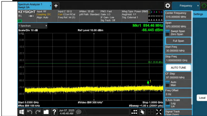
41-41-20MHz-15MHz-QPSK-QPSK-40546-40717-1RB#0-0RB#0-30~1000MHz-PASS
