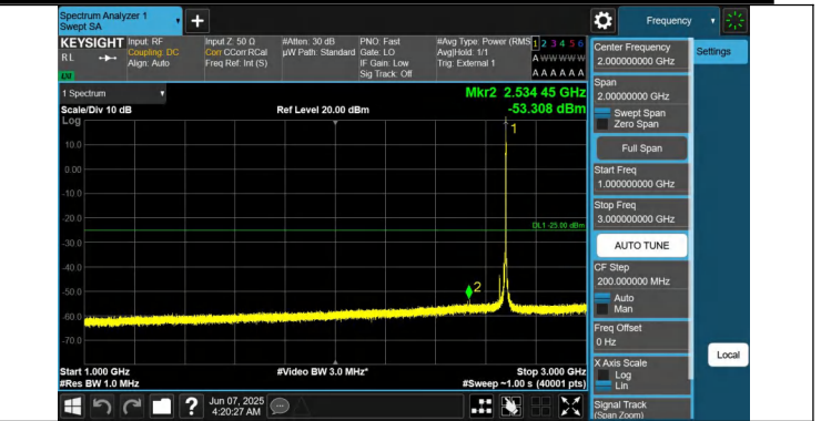
41-41-20MHz-10MHz-QPSK-QPSK-41391-41535-1RB#99-0RB#0 -1000~3000MHz-PASS
