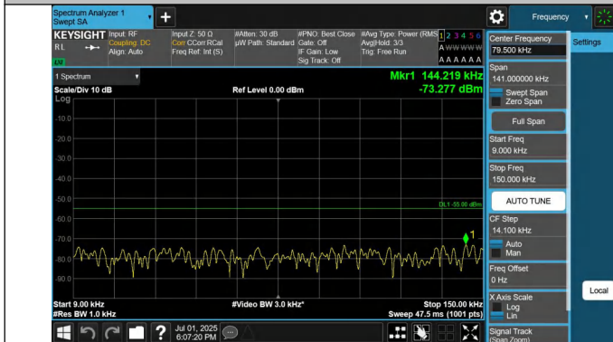
41-41-20MHz-10MHz-QPSK-QPSK-41391-41535-1RB#0-0RB#0- 0.009~0.15MHz-PASS
