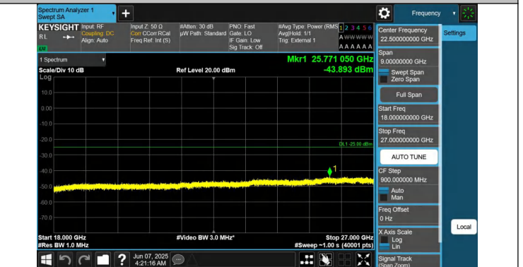
41-41-20MHz-10MHz-QPSK-QPSK-41391-41535-1RB#99-0RB#0 -18000~27000MHz-PASS
