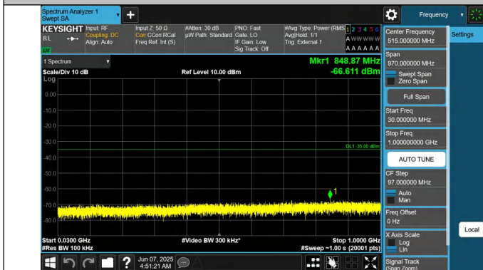
41-41-20MHz-15MHz-QPSK-QPSK-40546-40717-1RB#0-1RB#74-4-30~1000MHz-PASS
