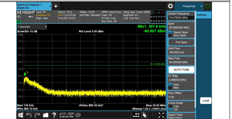
41-41-20MHz-10MHz-QPSK-QPSK-40571-40715-1RB#99-0RB#0 -0.15~30MHz-PASS
