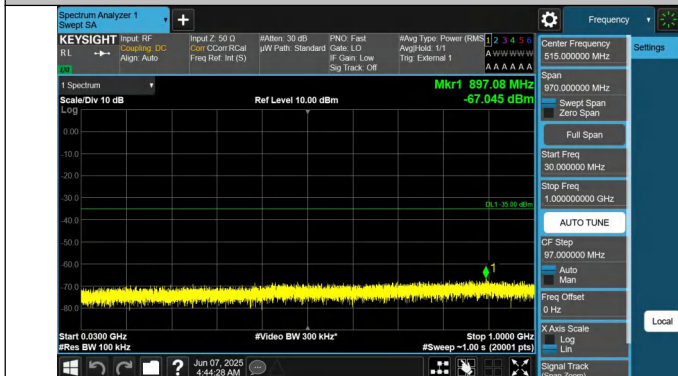
41-41-20MHz-15MHz-QPSK-QPSK-39750-39921-1RB#0-1RB#74-4-30~1000MHz-PASS
