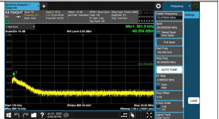
41-41-20MHz-15MHz-QPSK-QPSK-40546-40717-1RB#0-1RB#74-0.15~30MHz-PASS
