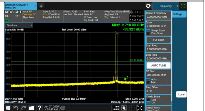
41-41-20MHz-15MHz-QPSK-QPSK-40546-40717-1RB#0-1RB#74-1000~3000MHz-PASS
