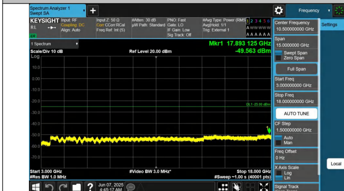
41-41-20MHz-15MHz-QPSK-QPSK-39750-39921-1RB#0-1RB#74-4-3000~18000MHz-PASS
