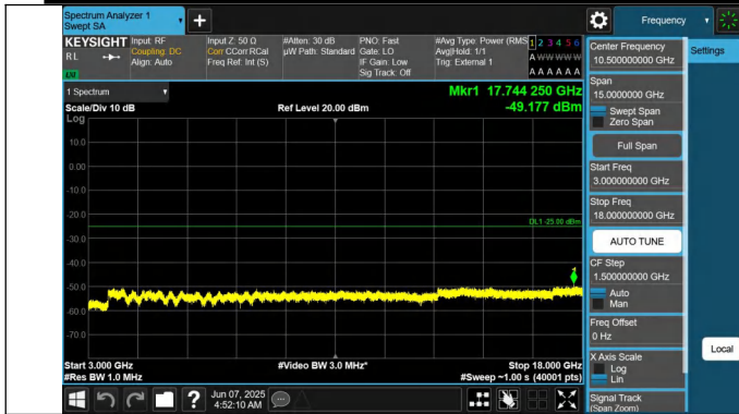
41-41-20MHz-15MHz-QPSK-QPSK-40546-40717-1RB#0-1RB#7 4-3000~18000MHz-PASS
