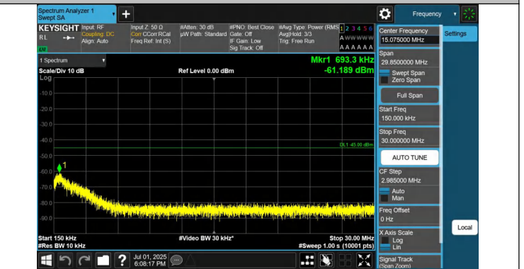
41-41-20MHz-15MHz-QPSK-QPSK-39750-39921-1RB#0-0RB#0- 0.15~30MHz-PASS
