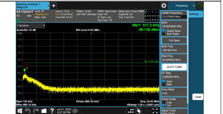
41-41-20MHz-10MHz-QPSK-QPSK-41391-41535-1RB#0-0RB#0- 0.15~30MHz-PASS
