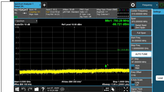
41-41-20MHz-10MHz-QPSK-QPSK-40571-40715-1RB#0-1RB#4 9-30~1000MHz-PASS
