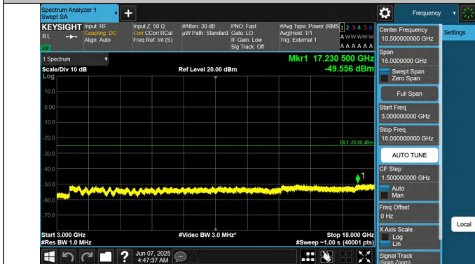
41-41-20MHz-15MHz-QPSK-QPSK-40546-40717-1RB#0-0RB#0-3000~18000MHz-PASS
