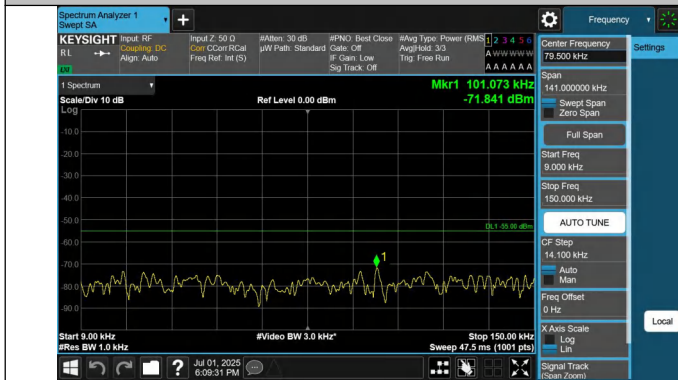
41-41-20MHz-15MHz-QPSK-QPSK-40546-40717-1RB#0-1RB#74-0.009~0.15MHz-PASS
