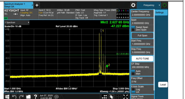
41-41-20MHz-15MHz-QPSK-QPSK-39750-39921-1RB#0-1RB#74-1000~3000MHz-PASS
