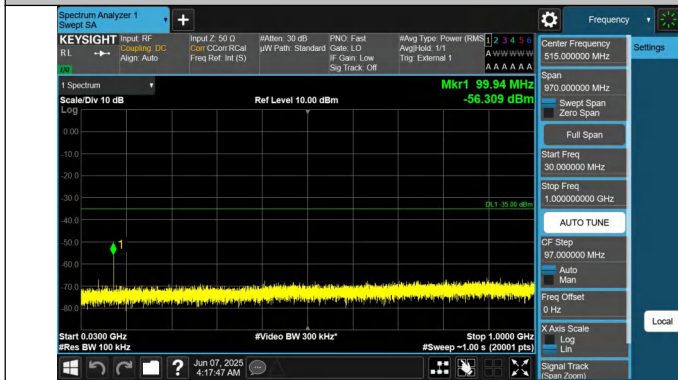
41-41-20MHz-10MHz-QPSK-QPSK-41391-41535-1RB#0-0RB#0- 30~1000MHz-PASS
