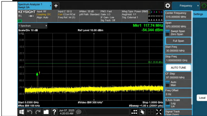
41-41-20MHz-10MHz-QPSK-QPSK-41391-41535-1RB#99-0RB# 0-30~1000MHz-PASS
