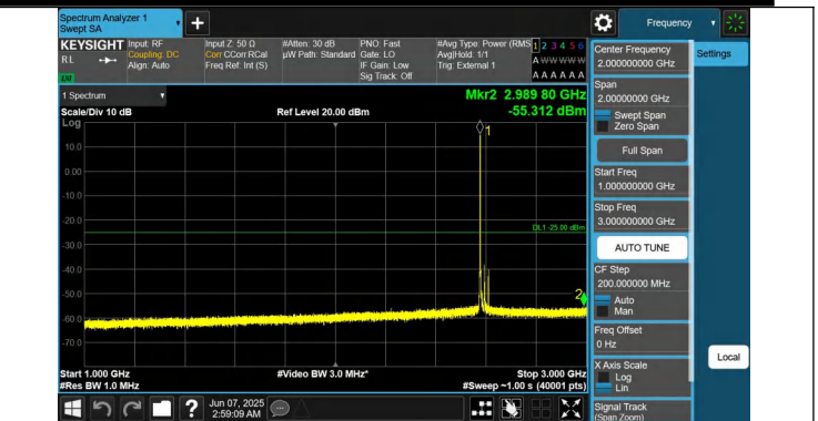
41-41-15MHz-20MHz-QPSK-QPSK-40523-40694-1RB#0-1RB#99 -1000~3000MHz-PASS
