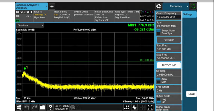
41-41-15MHz-20MHz-QPSK-QPSK-39728-39899-1RB#74-0RB#0 -0.15~30MHz-PASS
