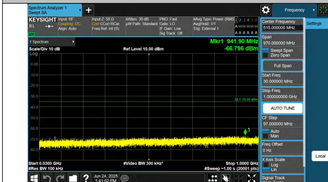
41-41-15MHz-15MHz-QPSK-QPSK-41365-41515-1RB#0-1RB#74-4-30~1000MHz-PASS
