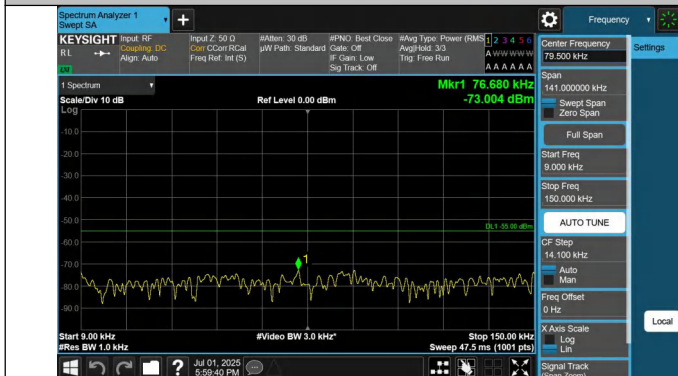
41-41-15MHz-15MHz-QPSK-QPSK-41365-41515-1RB#0-1RB#74-0.009~0.15MHz-PASS
