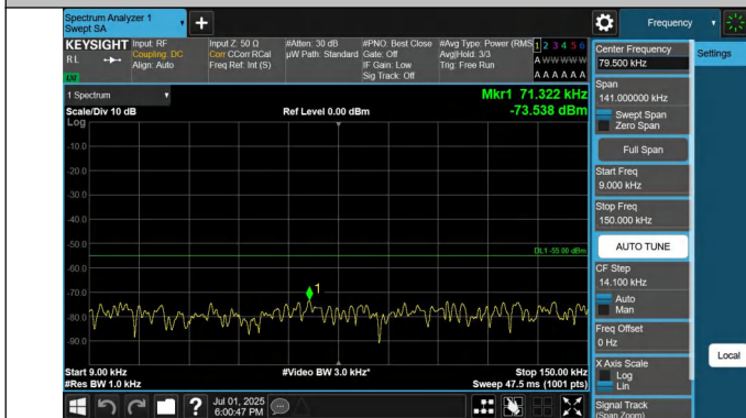
41-41-15MHz-20MHz-QPSK-QPSK-39728-39899-75RB#0-100R B#0-0.009~0.15MHz-PASS
