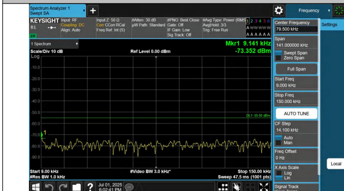
41-41-15MHz-20MHz-QPSK-QPSK-41319-41490-1RB#0-1RB#99-9-0.009~0.15MHz-PASS
