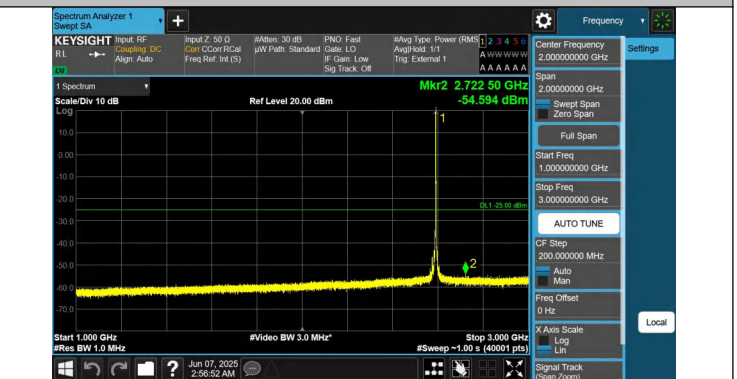
41-41-15MHz-20MHz-QPSK-QPSK-40523-40694-1RB#74-0RB#0 -1000~3000MHz-PASS
