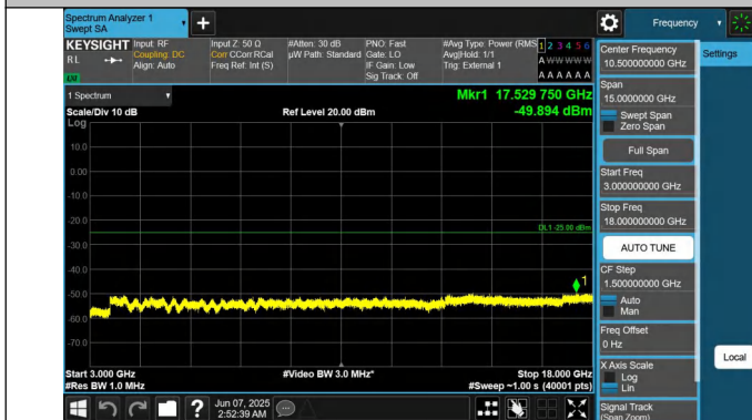
41-41-15MHz-20MHz-QPSK-QPSK-39728-39899-75RB#0-100R B#0-3000~18000MHz-PASS
