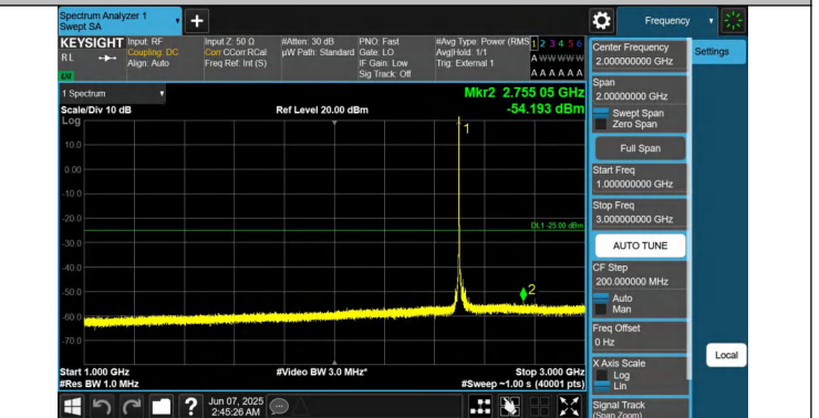
41-41-15MHz-20MHz-QPSK-QPSK-39728-39899-1RB#0-0RB#0-1000~3000MHz-PASS
