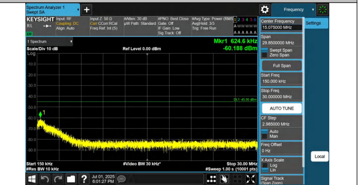
41-41-15MHz-20MHz-QPSK-QPSK-40523-40694-1RB#74-0RB#0 -0.15~30MHz-PASS
