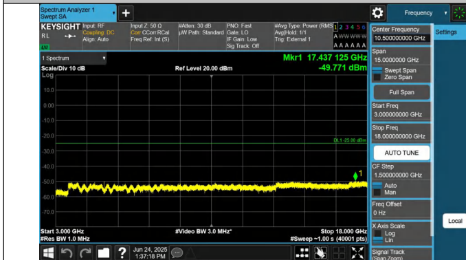
41-41-15MHz-15MHz-QPSK-QPSK-41365-41515-1RB#0-0RB#0-3000~18000MHz-PASS
