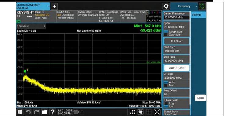
41-41-15MHz-20MHz-QPSK-QPSK-39728-39899-1RB#0-0RB#0-0.15~30MHz-PASS
