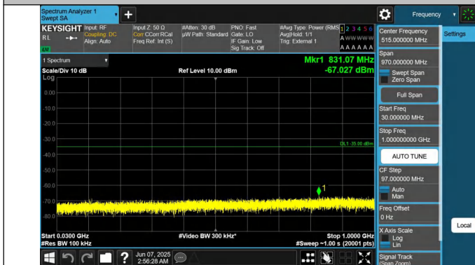
41-41-15MHz-20MHz-QPSK-QPSK-40523-40694-1RB#74-0RB# 0-30~1000MHz-PASS
