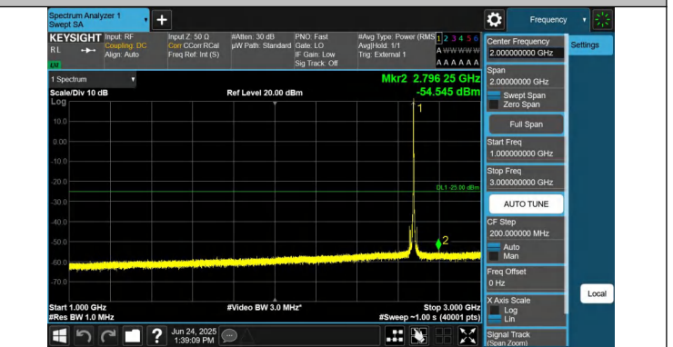
41-41-15MHz-15MHz-QPSK-QPSK-41365-41515-1RB#74-0RB#0 -1000~3000MHz-PASS
