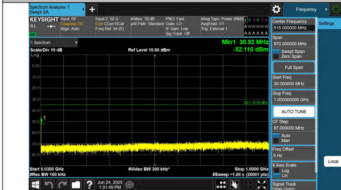
41-15MHz-15MHz-QPSK-QPSK-40545-40695-1RB#74-0RB# 0-30~1000MHz-PASS
