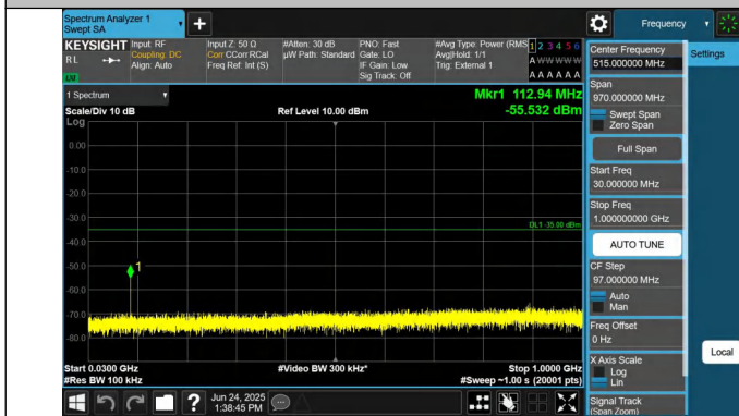
41-41-15MHz-15MHz-QPSK-QPSK-41365-41515-1RB#74-0RB# 0-30~1000MHz-PASS
