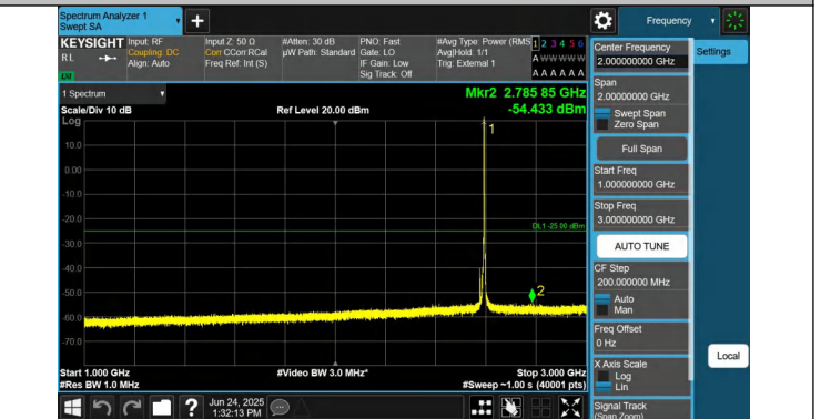
41-15MHz-15MHz-QPSK-QPSK-40545-40695-1RB#74-0RB# -1000~3000MHz-PASS
