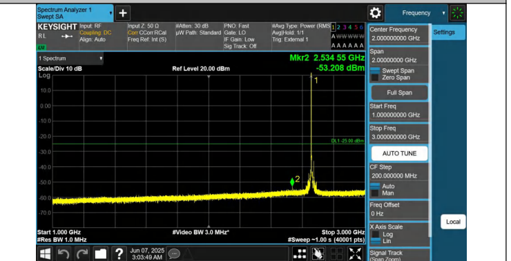
41-41-15MHz-20MHz-QPSK-QPSK-41319-41490-1RB#0-0RB#0-1000~3000MHz-PASS
