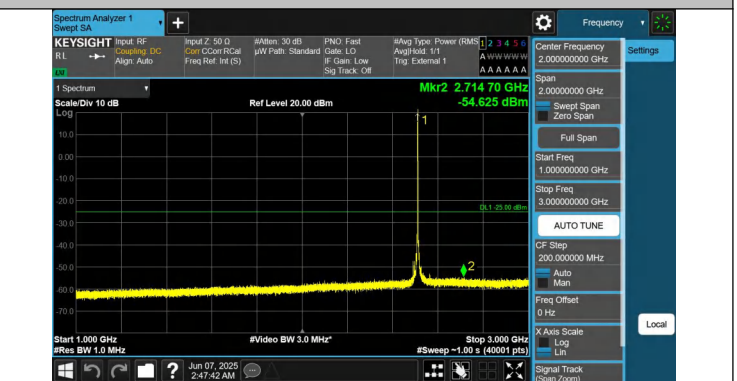
41-41-15MHz-20MHz-QPSK-QPSK-39728-39899-1RB#74-0RB#0 -1000~3000MHz-PASS
