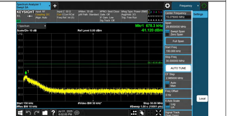
41-41-15MHz-20MHz-QPSK-QPSK-40523-40694-75RB#0-100RB #0-0.15~30MHz-PASS
