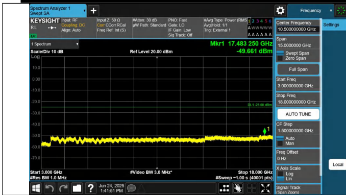
41-41-15MHz-15MHz-QPSK-QPSK-41365-41515-1RB#0-1RB#7 4-3000~18000MHz-PASS
