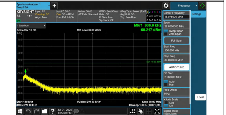
41-41-15MHz-20MHz-QPSK-QPSK-39728-39899-1RB#0-1RB#99-0.15~30MHz-PASS
