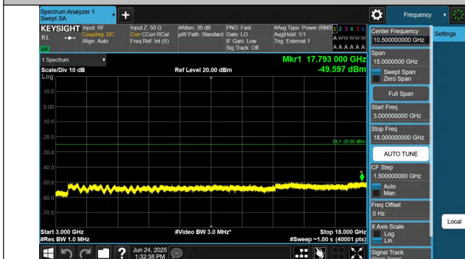
41-15MHz-15MHz-QPSK-QPSK-40545-40695-1RB#74-0RB# 0-3000~18000MHz-PASS
