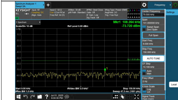
41-41-15MHz-20MHz-QPSK-QPSK-39728-39899-1RB#0-1RB#99-9-0.009~0.15MHz-PASS
