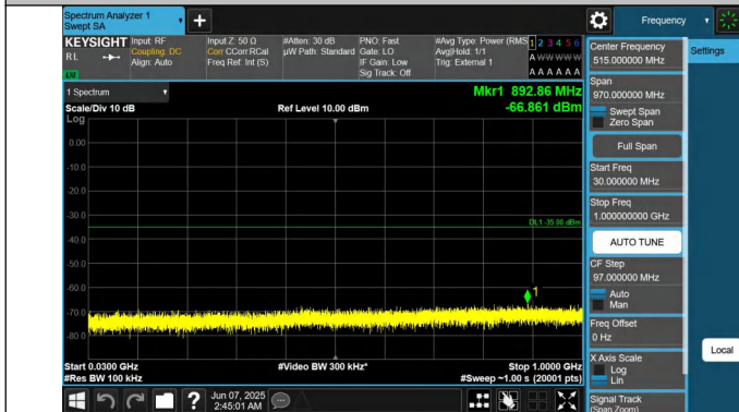
41-41-15MHz-20MHz-QPSK-QPSK-39728-39899-1RB#0-0RB#0-30~1000MHz-PASS
