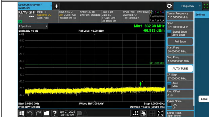
41-41-15MHz-20MHz-QPSK-QPSK-39728-39899-75RB#0-100R B#0-30~1000MHz-PASS
