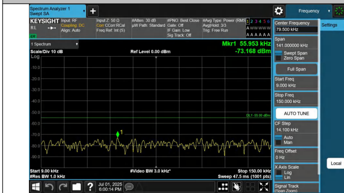
41-41-15MHz-20MHz-QPSK-QPSK-39728-39899-1RB#74-0RB# 0-0.009~0.15MHz-PASS
