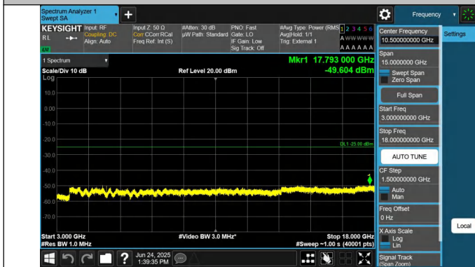
41-41-15MHz-15MHz-QPSK-QPSK-41365-41515-1RB#74-0RB# 0-3000~18000MHz-PASS
