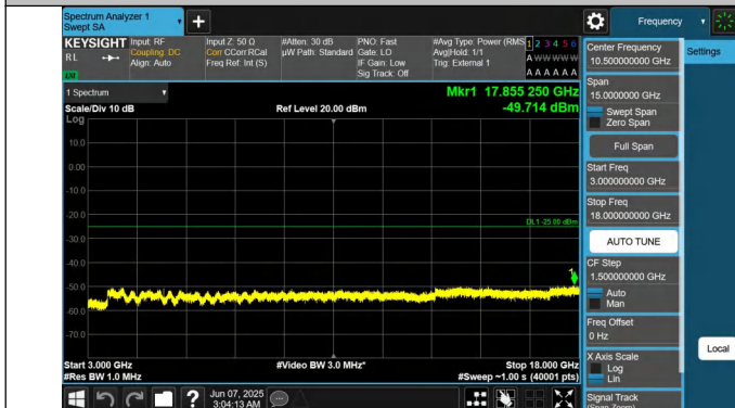
41-41-15MHz-20MHz-QPSK-QPSK-41319-41490-1RB#0-0RB#0-3000~18000MHz-PASS
