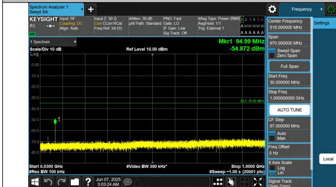
41-41-15MHz-20MHz-QPSK-QPSK-41319-41490-1RB#0-0RB#0-30~1000MHz-PASS
