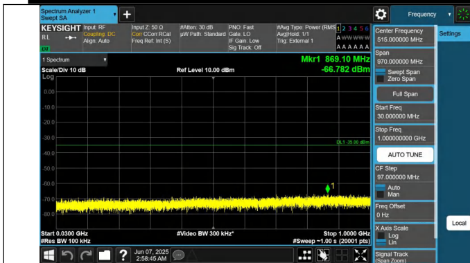
41-41-15MHz-20MHz-QPSK-QPSK-40523-40694-1RB#0-1RB#9 9-30~1000MHz-PASS
