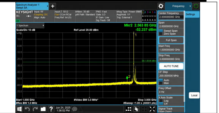
41-41-15MHz-15MHz-QPSK-QPSK-41365-41515-1RB#0-0RB#0-1000~3000MHz-PASS
