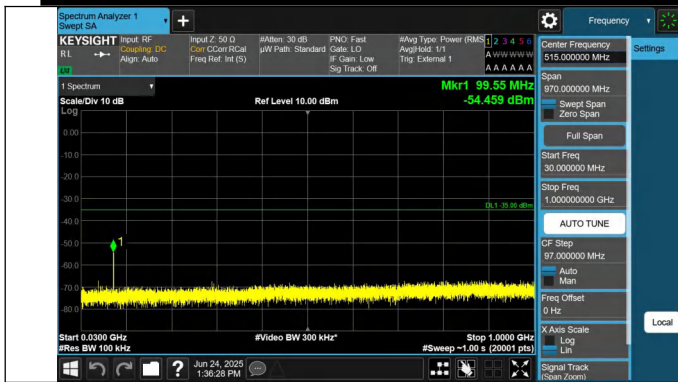
41-41-15MHz-15MHz-QPSK-QPSK-41365-41515-1RB#0-0RB#0-30~1000MHz-PASS
