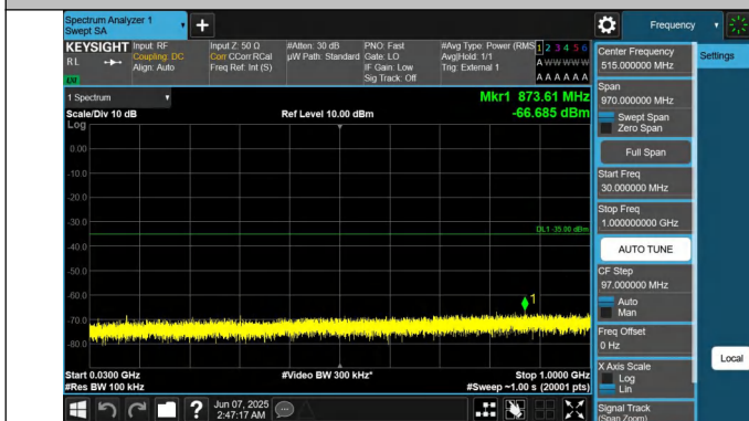
41-41-15MHz-20MHz-QPSK-QPSK-39728-39899-1RB#74-0RB# 0-30~1000MHz-PASS
