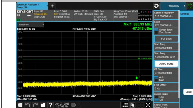
41-41-10MHz-20MHz-QPSK-QPSK-40526-40670-1RB#49-0RB# 0-30~1000MHz-PASS
