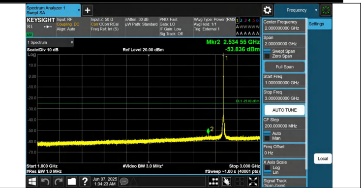
41-41-10MHz-20MHz-QPSK-QPSK-41346-41490-1RB#49-0RB#0 -1000~3000MHz-PASS
