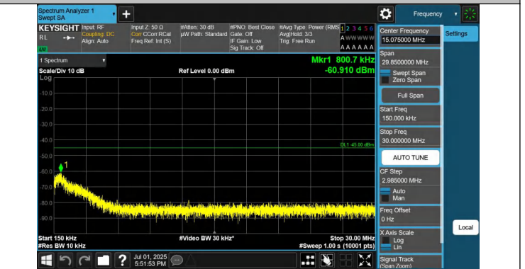
41-41-10MHz-15MHz-QPSK-QPSK-41395-41515-1RB#0-0RB#0- 0.15~30MHz-PASS
