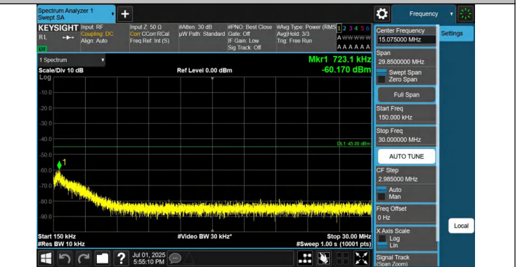
41-41-15MHz-10MHz-QPSK-QPSK-39725-39845-1RB#0-0RB#0- 0.15~30MHz-PASS
