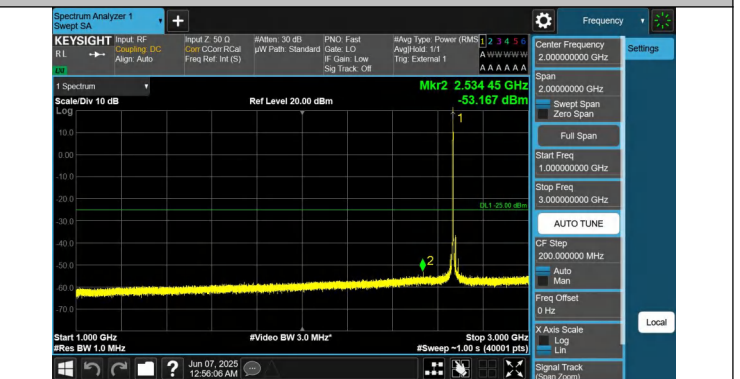
41-41-10MHz-15MHz-QPSK-QPSK-41395-41515-1RB#0-0RB#0- 1000~3000MHz-PASS
