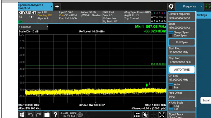
41-41-15MHz-10MHz-QPSK-QPSK-39725-39845-1RB#0-0RB#0- 30~1000MHz-PASS
