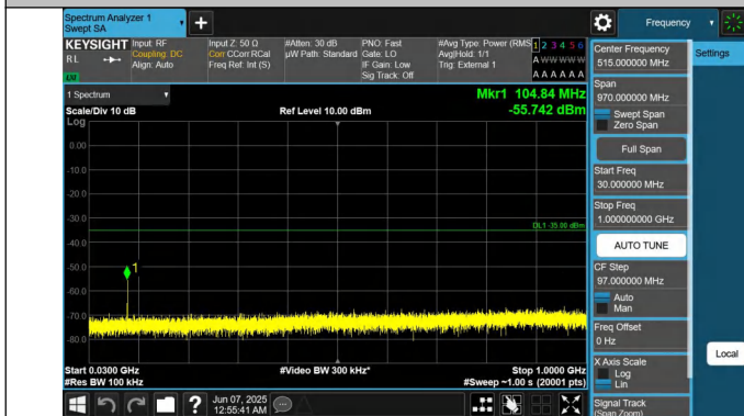
41-41-10MHz-15MHz-QPSK-QPSK-41395-41515-1RB#0-0RB#0- 30~1000MHz-PASS
