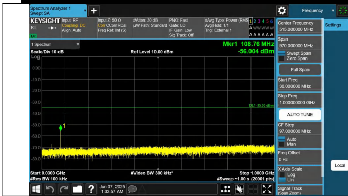
41-41-10MHz-20MHz-QPSK-QPSK-41346-41490-1RB#49-0RB# 0-30~1000MHz-PASS
