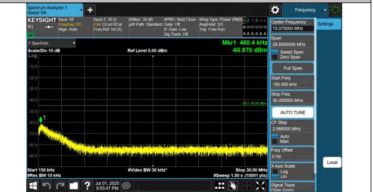
41-41-10MHz-20MHz-QPSK-QPSK-40526-40670-1RB#49-0RB#0 -0.15~30MHz-PASS
