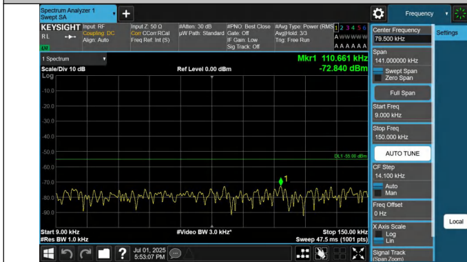
41-41-10MHz-20MHz-QPSK-QPSK-39705-39849-1RB#0-1RB#99-9-0.009~0.15MHz-PASS
