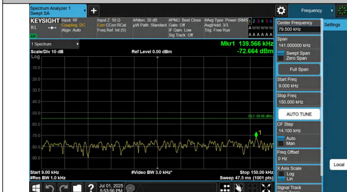
41-41-10MHz-20MHz-QPSK-QPSK-40526-40670-1RB#0-1RB#9 9-0.009~0.15MHz-PASS
