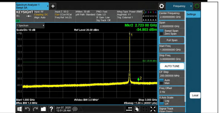
41-41-10MHz-15MHz-QPSK-QPSK-40549-40669-1RB#49-0RB#0 -1000~3000MHz-PASS
