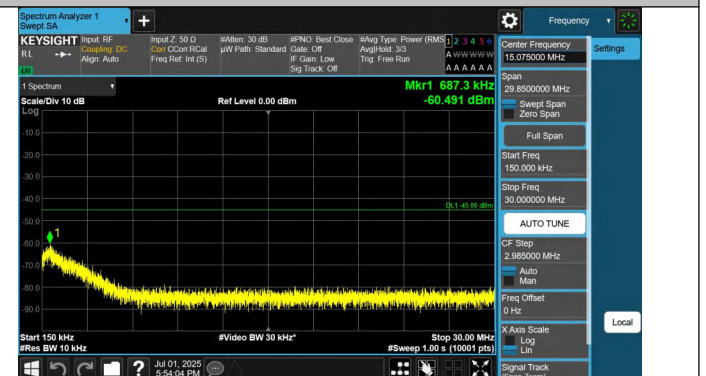
41-41-10MHz-20MHz-QPSK-QPSK-40526-40670-1RB#0-1RB#99 -0.15~30MHz-PASS
