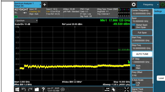
41-41-10MHz-15MHz-QPSK-QPSK-40549-40669-1RB#49-0RB# 0-3000~18000MHz-PASS
