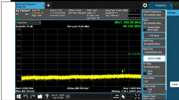
41-41-10MHz-20MHz-QPSK-QPSK-40526-40670-1RB#0-1RB#9 9-30~1000MHz-PASS
