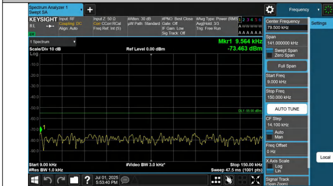
41-41-10MHz-20MHz-QPSK-QPSK-40526-40670-1RB#49-0RB# 0-0.009~0.15MHz-PASS
