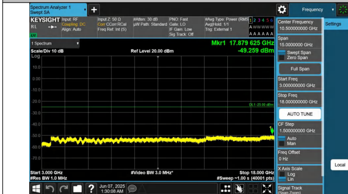
41-41-10MHz-20MHz-QPSK-QPSK-40526-40670-1RB#0-1RB#9 9-3000~18000MHz-PASS
