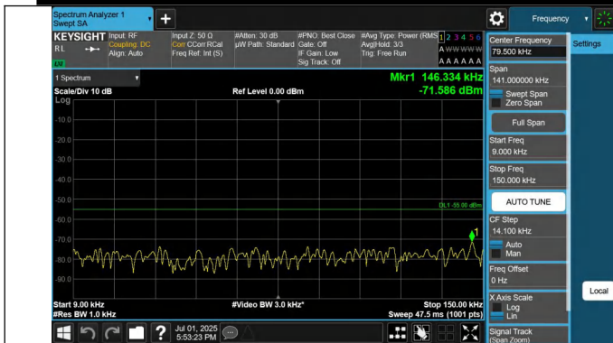
41-41-10MHz-20MHz-QPSK-QPSK-40526-40670-1RB#0-0RB#0- 0.009~0.15MHz-PASS
