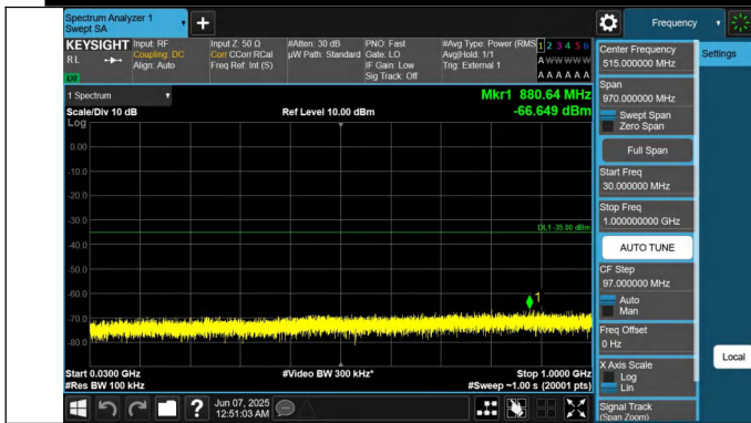
41-41-10MHz-15MHz-QPSK-QPSK-40549-40669-1RB#49-0RB# 0-30~1000MHz-PASS
