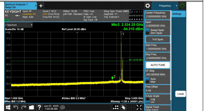
41-41-10MHz-15MHz-QPSK-QPSK-41395-41515-1RB#0-1RB#74-1000~3000MHz-PASS
