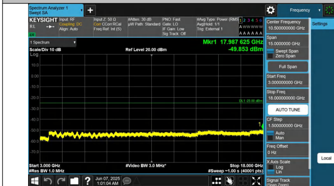
41-41-10MHz-15MHz-QPSK-QPSK-41395-41515-1RB#0-1RB#74-4-3000~18000MHz-PASS
