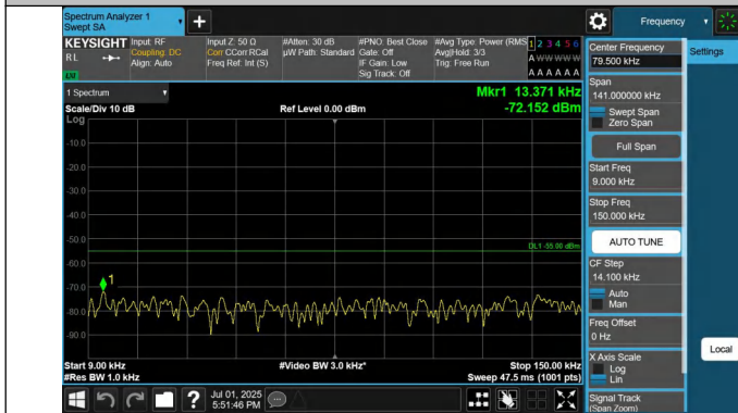
41-41-10MHz-15MHz-QPSK-QPSK-41395-41515-1RB#0-0RB#0- 0.009~0.15MHz-PASS
