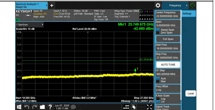
41-41-10MHz-20MHz-QPSK-QPSK-41346-41490-1RB#49-0RB#0 -18000~27000MHz-PASS
