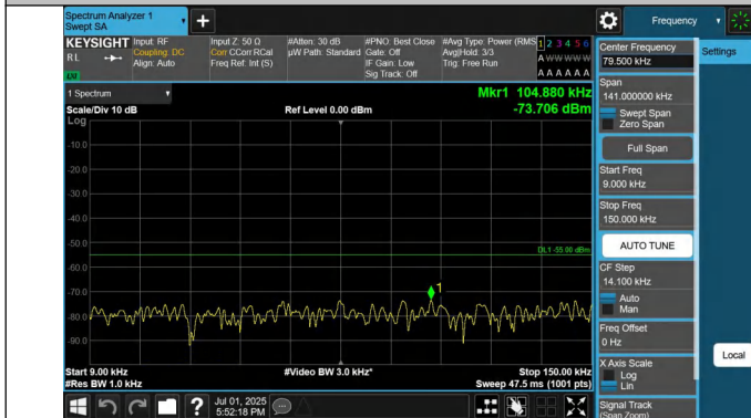
41-41-10MHz-15MHz-QPSK-QPSK-41395-41515-1RB#0-1RB#74-0.009~0.15MHz-PASS
