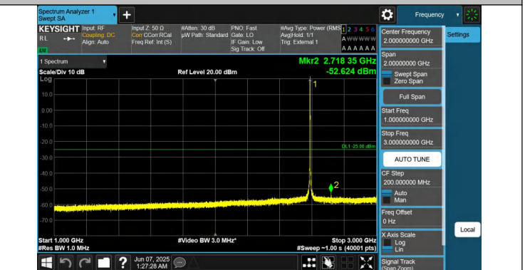
41-41-10MHz-20MHz-QPSK-QPSK-40526-40670-1RB#49-0RB#0 -1000~3000MHz-PASS
