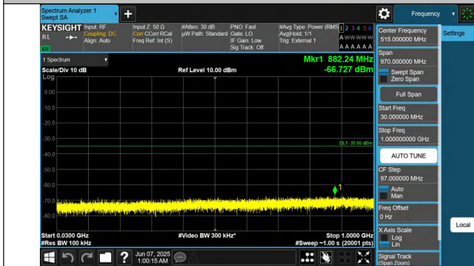
41-41-10MHz-15MHz-QPSK-QPSK-41395-41515-1RB#0-1RB#74-4-30~1000MHz-PASS
