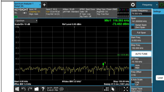
41-41-5MHz-20MHz-QPSK-QPSK-41373-41490-1RB#0-1RB#99- 0.009~0.15MHz-PASS
