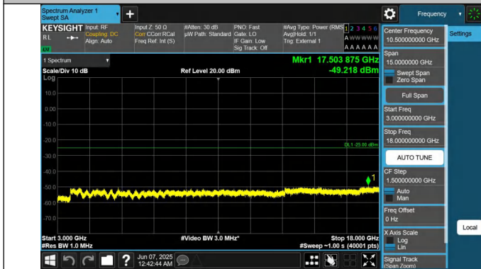
41-41-10MHz-15MHz-QPSK-QPSK-39703-39823-1RB#0-0RB#0- 3000~18000MHz-PASS
