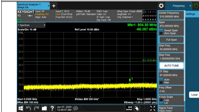
41-41-10MHz-15MHz-QPSK-QPSK-40549-40669-1RB#0-0RB#0- 30~1000MHz-PASS
