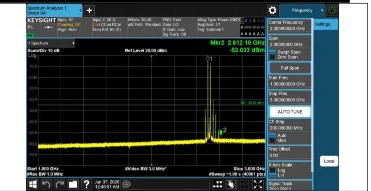
41-41-10MHz-15MHz-QPSK-QPSK-39703-39823-1RB#0-1RB#74 -1000~3000MHz-PASS
