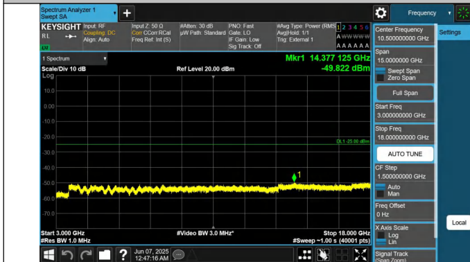
41-41-10MHz-15MHz-QPSK-QPSK-39703-39823-1RB#0-1RB#7 4-3000~18000MHz-PASS
