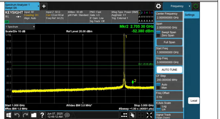
41-41-10MHz-15MHz-QPSK-QPSK-40549-40669-1RB#0-0RB#0- 1000~3000MHz-PASS
