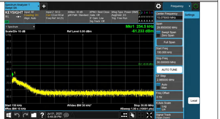
41-41-5MHz-20MHz-QPSK-QPSK-40528-40645-1RB#0-0RB#0-0.15~30MHz-PASS
