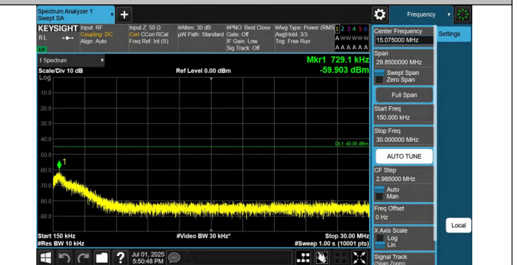
41-41-10MHz-15MHz-QPSK-QPSK-39703-39823-1RB#0-1RB#74 -0.15~30MHz-PASS
