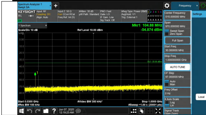
41-41-5MHz-20MHz-QPSK-QPSK-41373-41490-1RB#0-0RB#0-3 0~1000MHz-PASS
