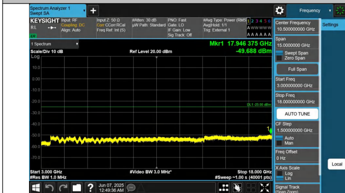
41-41-10MHz-15MHz-QPSK-QPSK-40549-40669-1RB#0-0RB#0- 3000~18000MHz-PASS
