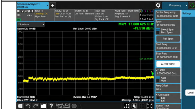
41-41-5MHz-20MHz-QPSK-QPSK-39683-39800-1RB#24-0RB#0-3000~18000MHz-PASS
