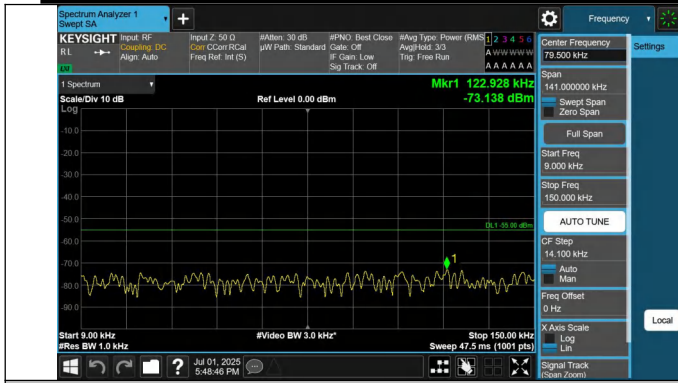
41-41-5MHz-20MHz-QPSK-QPSK-40528-40645-1RB#24-0RB#0- 0.009~0.15MHz-PASS
