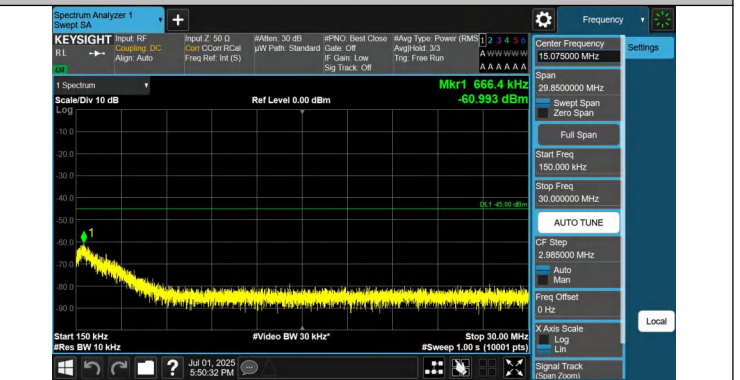
41-41-10MHz-15MHz-QPSK-QPSK-39703-39823-1RB#49-0RB#0 -0.15~30MHz-PASS
