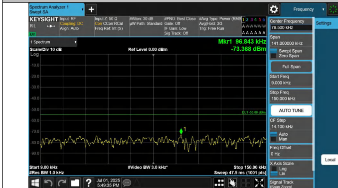
41-41-5MHz-20MHz-QPSK-QPSK-41373-41490-1RB#24-0RB#0- 0.009~0.15MHz-PASS
