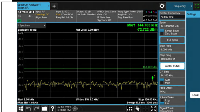
41-41-10MHz-15MHz-QPSK-QPSK-39703-39823-1RB#0-0RB#0- 0.009~0.15MHz-PASS
