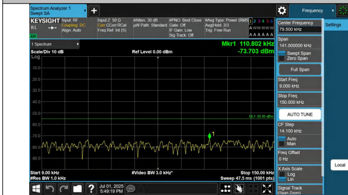
41-41-5MHz-20MHz-QPSK-QPSK-41373-41490-1RB#0-0RB#0-0 .009~0.15MHz-PASS
