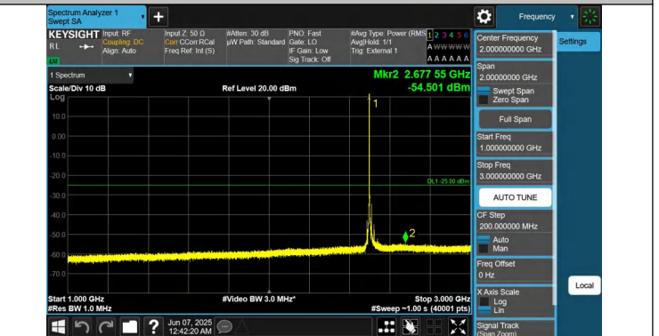
41-41-10MHz-15MHz-QPSK-QPSK-39703-39823-1RB#0-0RB#0- 1000~3000MHz-PASS
