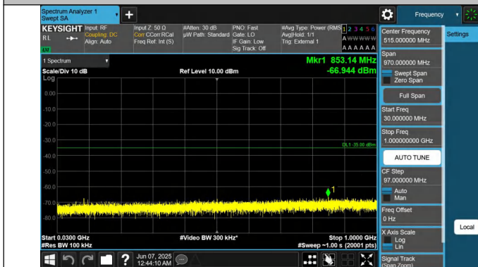
41-41-10MHz-15MHz-QPSK-QPSK-39703-39823-1RB#49-0RB# 0-30~1000MHz-PASS
