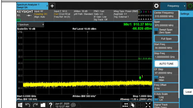
41-41-5MHz-20MHz-QPSK-QPSK-40528-40645-1RB#0-0RB#0-30~1000MHz-PASS
