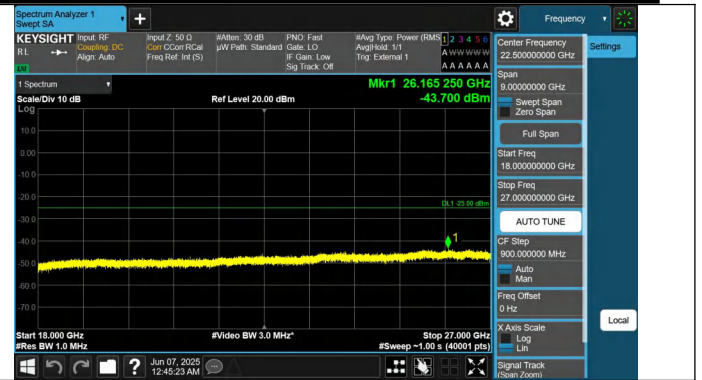
41-41-10MHz-15MHz-QPSK-QPSK-39703-39823-1RB#49-0RB#0 -18000~27000MHz-PASS
