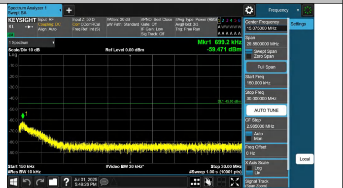
41-41-5MHz-20MHz-QPSK-QPSK-41373-41490-1RB#0-0RB#0-0. 15~30MHz-PASS
