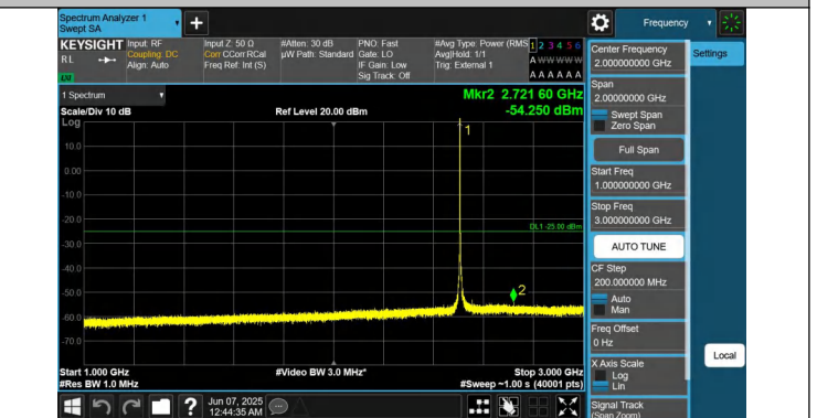
41-41-10MHz-15MHz-QPSK-QPSK-39703-39823-1RB#49-0RB#0 -1000~3000MHz-PASS
