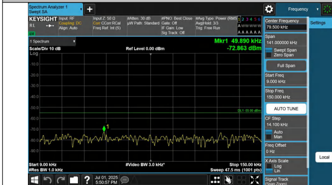
41-41-10MHz-15MHz-QPSK-QPSK-40549-40669-1RB#0-0RB#0- 0.009~0.15MHz-PASS
