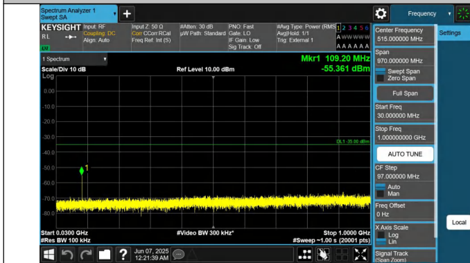
41-41-5MHz-20MHz-QPSK-QPSK-41373-41490-1RB#24-0RB#0- 30~1000MHz-PASS
