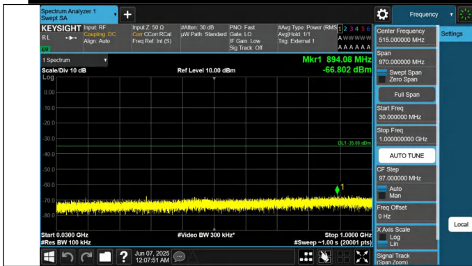
41-41-5MHz-20MHz-QPSK-QPSK-39683-39800-1RB#24-0RB#0-30~1000MHz-PASS
