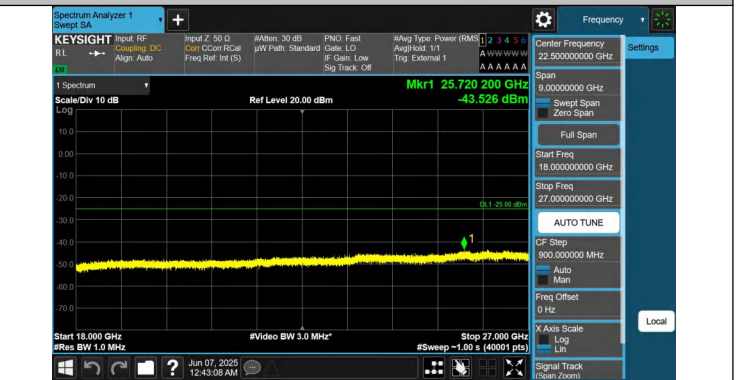
41-41-10MHz-15MHz-QPSK-QPSK-39703-39823-1RB#0-0RB#0- 18000~27000MHz-PASS
