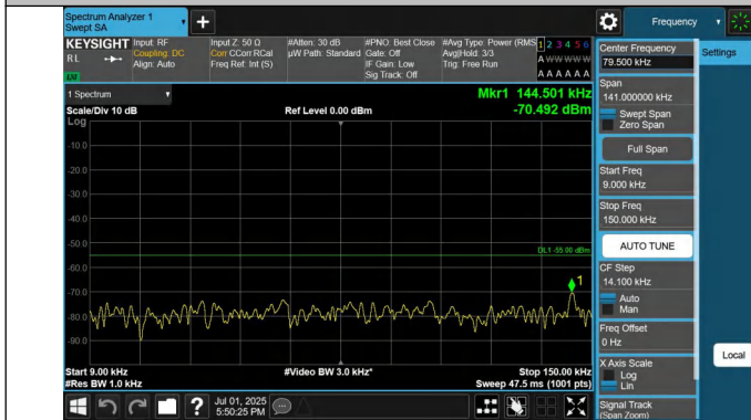
41-41-10MHz-15MHz-QPSK-QPSK-39703-39823-1RB#49-0RB# 0-0.009~0.15MHz-PASS
