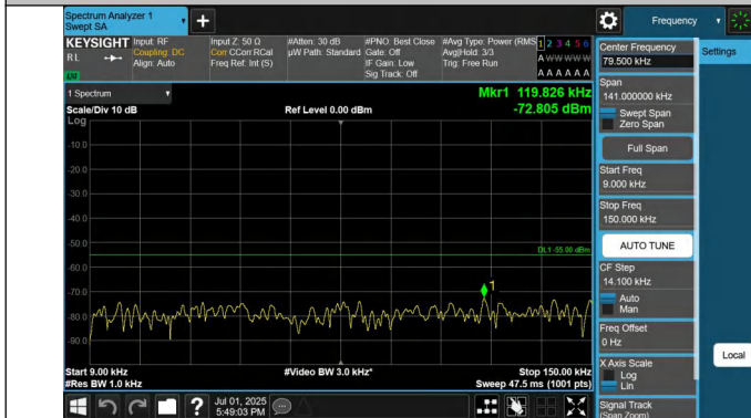
41-41-5MHz-20MHz-QPSK-QPSK-40528-40645-1RB#0-1RB#99- 0.009~0.15MHz-PASS
