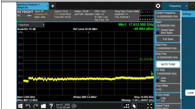
41-41-5MHz-20MHz-QPSK-QPSK-41373-41490-1RB#24-0RB#0- 3000~18000MHz-PASS
