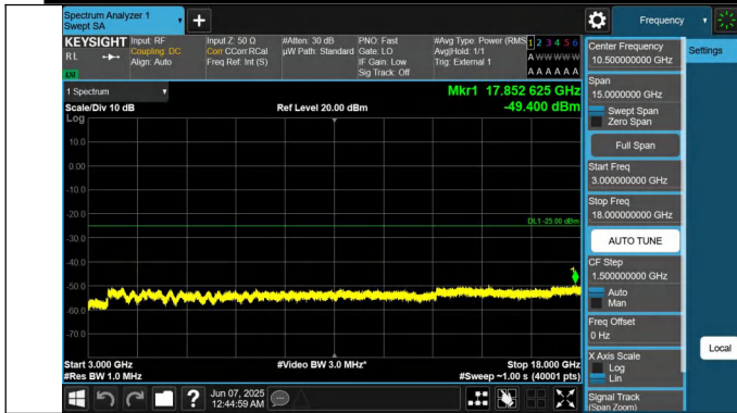
41-41-10MHz-15MHz-QPSK-QPSK-39703-39823-1RB#49-0RB# 0-3000~18000MHz-PASS
