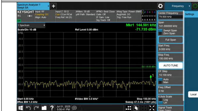
41-41-10MHz-15MHz-QPSK-QPSK-39703-39823-1RB#0-1RB#7 4-0.009~0.15MHz-PASS
