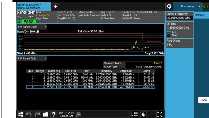
41-41-20MHz-10MHz-QPSK@QPSK-QPSK@QPSK-41391-415 35-1RB#99@100RB#0-0RB#0@50RB#0-PASS
