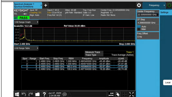
41-41-15MHz-20MHz-QPSK@QPSK-QPSK@QPSK-39728-398 99-1RB#0@75RB#0-0RB#0@100RB#0-PASS
