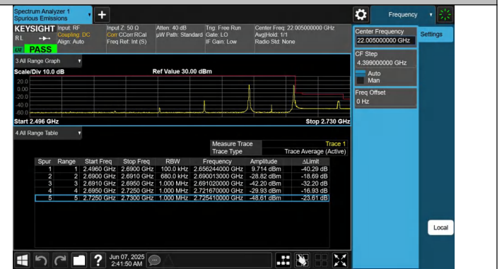
41-41-15MHz-20MHz-QPSK@QPSK-QPSK@QPSK-41319-41490 -1RB#0@75RB#0-1RB#99@100RB#0-PASS
