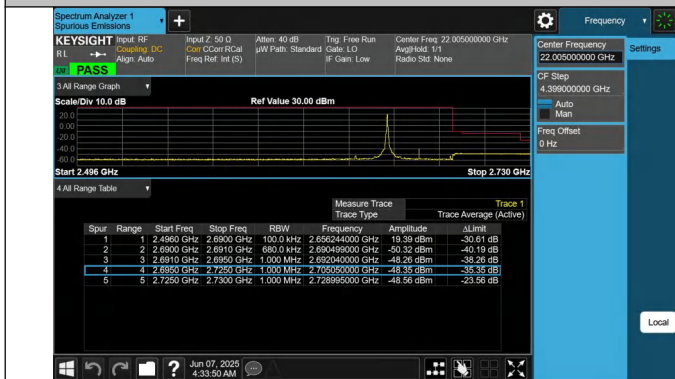
41-41-20MHz-15MHz-QPSK@QPSK-QPSK@QPSK-41341-415 12-1RB#0@100RB#0-0RB#0@75RB#0-PASS
