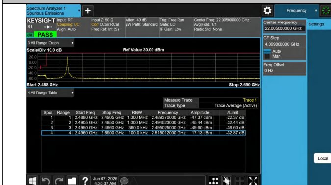
41-41-20MHz-15MHz-QPSK@QPSK-QPSK@QPSK-39750-399 21-1RB#99@100RB#0-0RB#0@75RB#0-PASS
