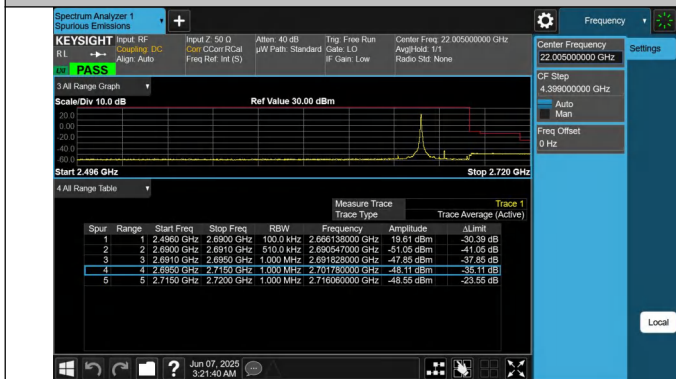
41-41-20MHz-5MHz-QPSK@QPSK-QPSK@QPSK-41440-4155 7-1RB#0@100RB#0-0RB#0@25RB#0-PASS
