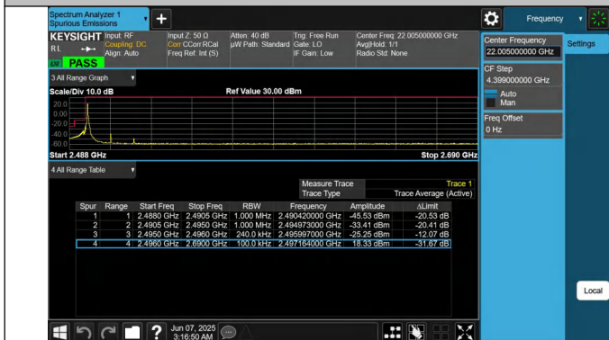
41-41-20MHz-5MHz-QPSK@QPSK-QPSK@QPSK-39750-3986 7-1RB#0@100RB#0-0RB#0@25RB#0-PASS
