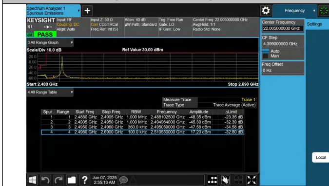
41-41-15MHz-20MHz-QPSK@QPSK-QPSK@QPSK-39728-398 99-1RB#74@75RB#0-0RB#0@100RB#0-PASS
