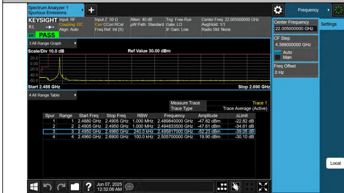
41-41-10MHz-15MHz-QPSK@QPSK-QPSK@QPSK-39703-398 23-1RB#49@50RB#0-0RB#0@75RB#0-PASS
