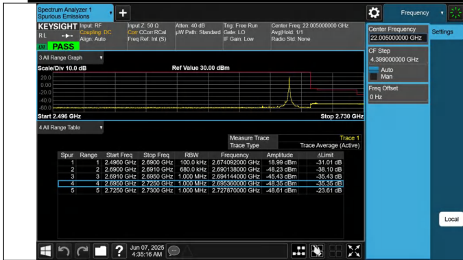
41-41-20MHz-15MHz-QPSK@QPSK-QPSK@QPSK-41341-415 12-1RB#99@100RB#0-0RB#0@75RB#0-PASS
