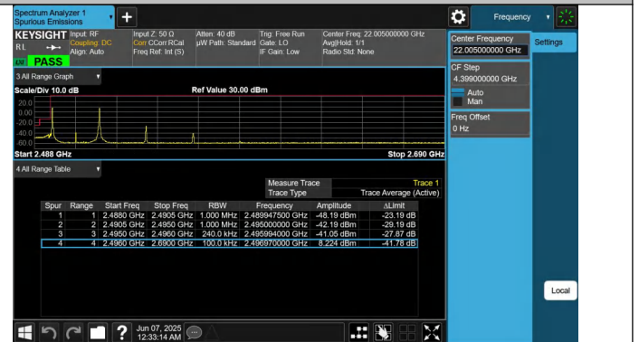
41-41-10MHz-15MHz-QPSK@QPSK-QPSK@QPSK-39703-39823 -1RB#0@50RB#0-1RB#74@75RB#0-PASS
