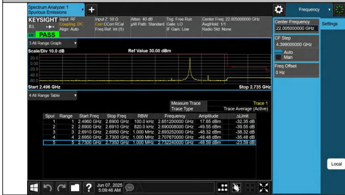
41-41-20MHz-20MHz-QPSK@QPSK-QPSK@QPSK-41292-414 90-1RB#0@100RB#0-0RB#0@100RB#0-PASS
