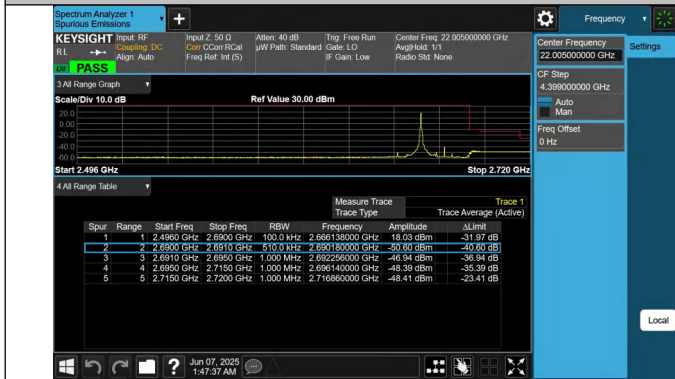
41-41-15MHz-10MHz-QPSK@QPSK-QPSK@QPSK-41417-415 37-1RB#0@75RB#0-0RB#0@50RB#0-PASS
