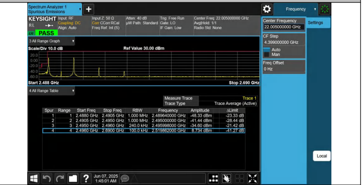
41-41-15MHz-10MHz-QPSK@QPSK-QPSK@QPSK-39725-39845 -1RB#0@75RB#0-1RB#49@50RB#0-PASS
