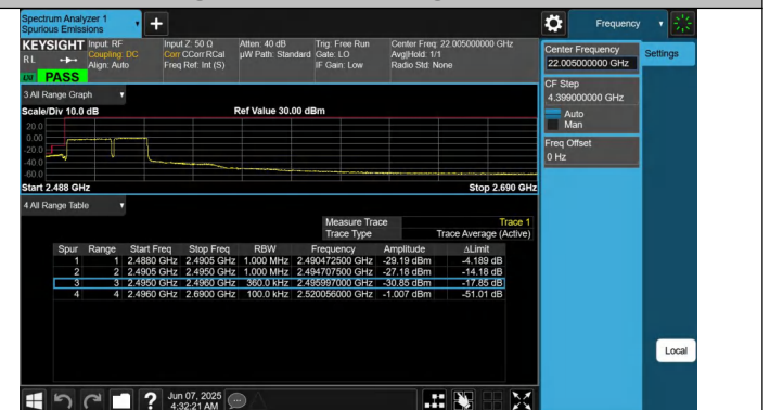
41-41-20MHz-15MHz-QPSK@QPSK-QPSK@QPSK-39750-39921 -100RB#0@100RB#0-75RB#0@75RB#0-PASS
