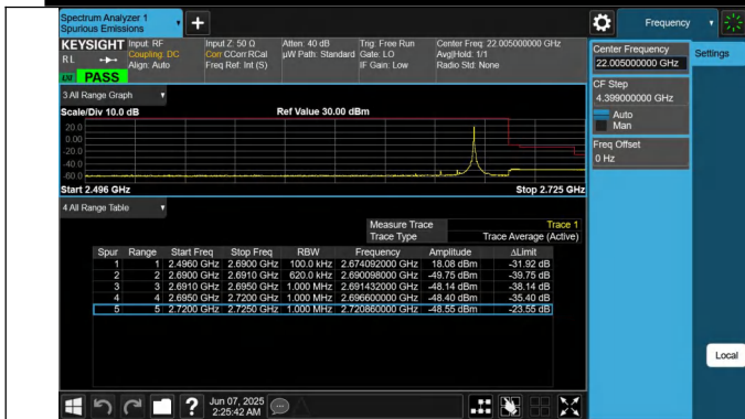
41-41-15MHz-15MHz-QPSK@QPSK-QPSK@QPSK-41365-415 15-1RB#74@75RB#0-0RB#0@75RB#0-PASS
