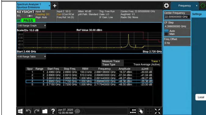
41-41-10MHz-15MHz-QPSK@QPSK-QPSK@QPSK-41395-415 15-1RB#0@50RB#0-0RB#0@75RB#0-PASS
