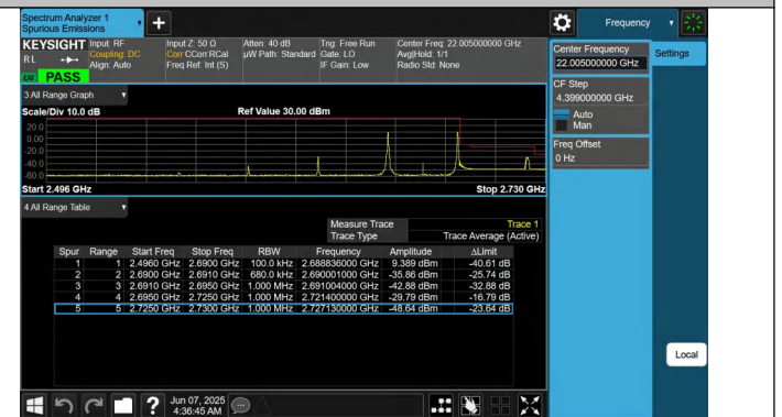
41-41-20MHz-15MHz-QPSK@QPSK-QPSK@QPSK-41341-41512 -1RB#0@100RB#0-1RB#74@75RB#0-PASS
