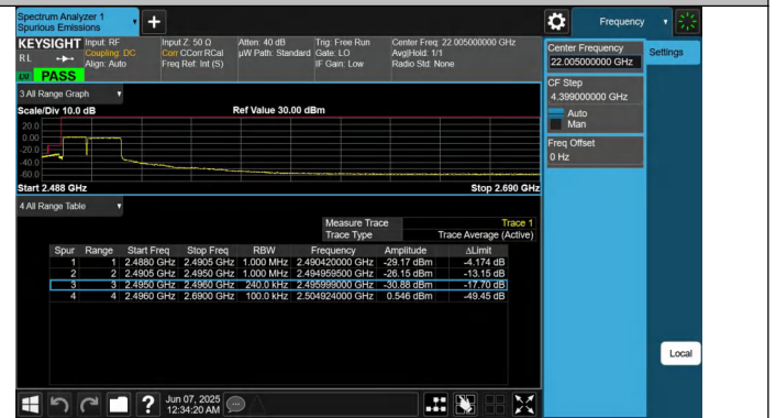
41-41-10MHz-15MHz-QPSK@QPSK-QPSK@QPSK-39703-39823 -50RB#0@50RB#0-75RB#0@75RB#0-PASS
