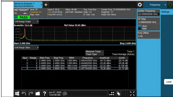
41-41-20MHz-20MHz-QPSK@QPSK-QPSK@QPSK-39750-399 48-1RB#0@100RB#0-0RB#0@100RB#0-PASS
