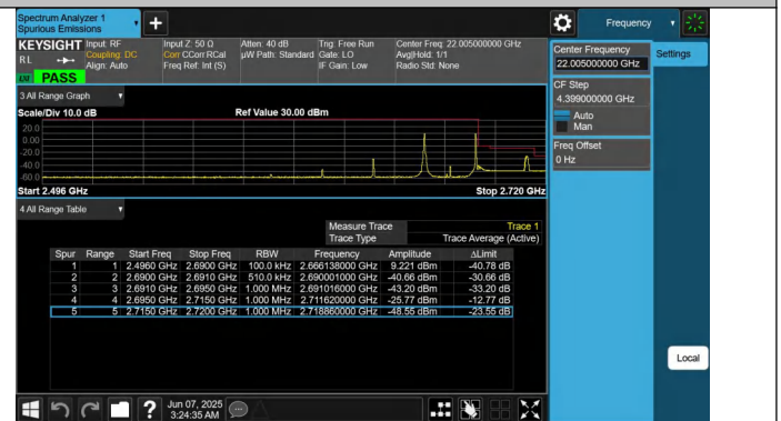
41-41-20MHz-5MHz-QPSK@QPSK-QPSK@QPSK-41440-41557- 1RB#0@100RB#0-1RB#24@25RB#0-PASS
