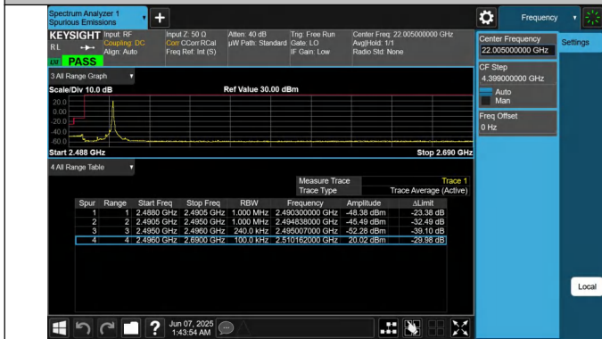
41-41-15MHz-10MHz-QPSK@QPSK-QPSK@QPSK-39725-398 45-1RB#74@75RB#0-0RB#0@50RB#0-PASS
