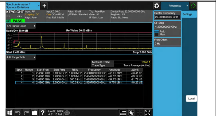
41-41-20MHz-15MHz-QPSK@QPSK-QPSK@QPSK-39750-39921 -1RB#0@100RB#0-1RB#74@75RB#0-PASS
