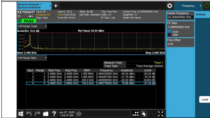
41-41-15MHz-10MHz-QPSK@QPSK-QPSK@QPSK-39725-398 45-1RB#0@75RB#0-0RB#0@50RB#0-PASS
