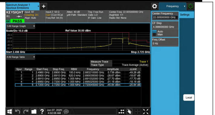
41-41-20MHz-10MHz-QPSK@QPSK-QPSK@QPSK-41391-41535 -100RB#0@100RB#0-50RB#0@50RB#0-PASS
