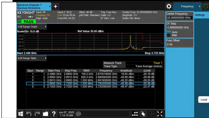
41-41-10MHz-20MHz-QPSK@QPSK-QPSK@QPSK-41346-414 90-1RB#49@50RB#0-0RB#0@100RB#0-PASS
