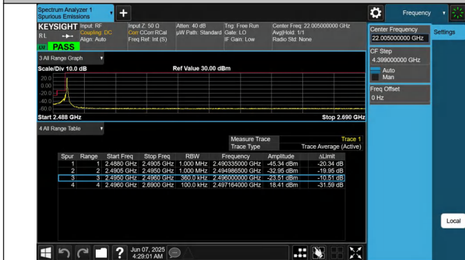
41-41-20MHz-15MHz-QPSK@QPSK-QPSK@QPSK-39750-399 21-1RB#0@100RB#0-0RB#0@75RB#0-PASS
