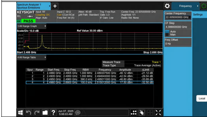
41-41-20MHz-20MHz-QPSK@QPSK-QPSK@QPSK-39750-399 48-1RB#99@100RB#0-0RB#0@100RB#0-PASS
