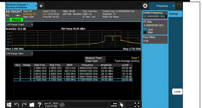
41-41-15MHz-15MHz-QPSK@QPSK-QPSK@QPSK-41365-41515 -75RB#0@75RB#0-75RB#0@75RB#0-PASS
