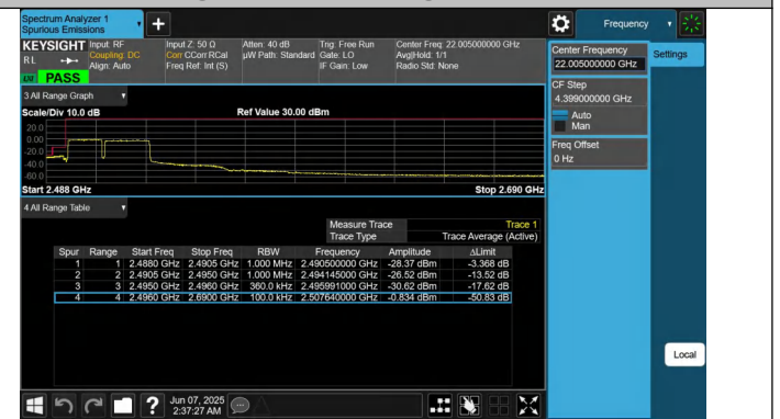
41-41-15MHz-20MHz-QPSK@QPSK-QPSK@QPSK-39728-39899 -75RB#0@75RB#0-100RB#0@100RB#0-PASS
