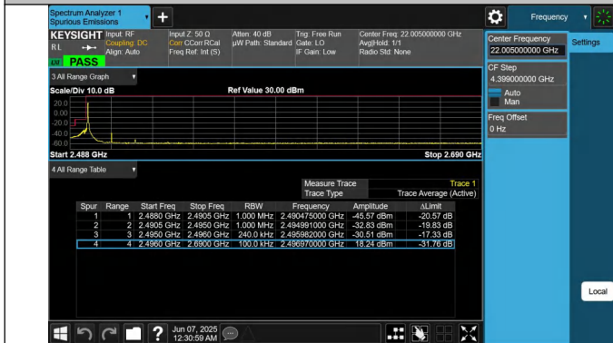
41-41-10MHz-15MHz-QPSK@QPSK-QPSK@QPSK-39703-398 23-1RB#0@50RB#0-0RB#0@75RB#0-PASS
