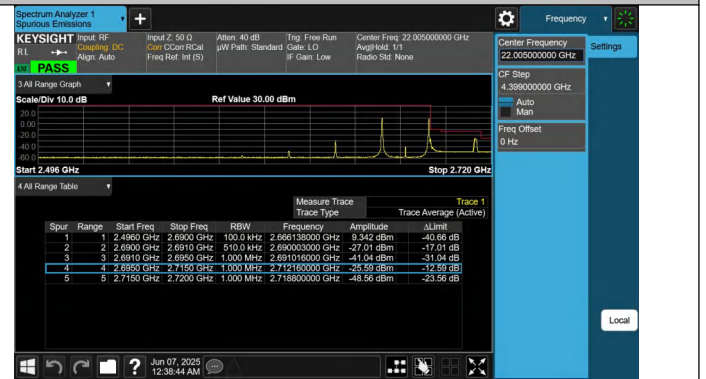
41-41-10MHz-15MHz-QPSK@QPSK-QPSK@QPSK-41395-41515 -1RB#0@50RB#0-1RB#74@75RB#0-PASS
