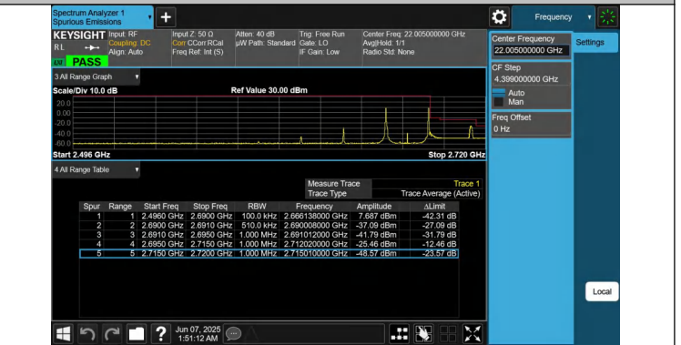
41-41-15MHz-10MHz-QPSK@QPSK-QPSK@QPSK-41417-41537 -1RB#0@75RB#0-1RB#49@50RB#0-PASS
