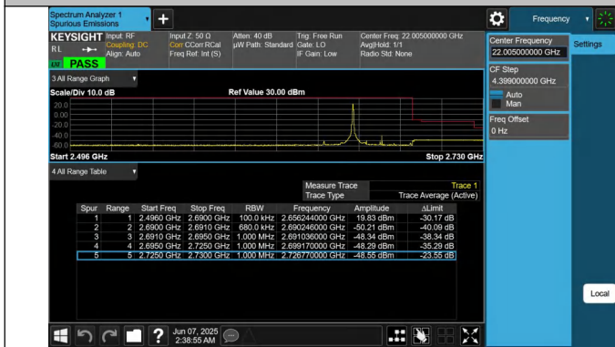
41-41-15MHz-20MHz-QPSK@QPSK-QPSK@QPSK-41319-414 90-1RB#0@75RB#0-0RB#0@100RB#0-PASS
