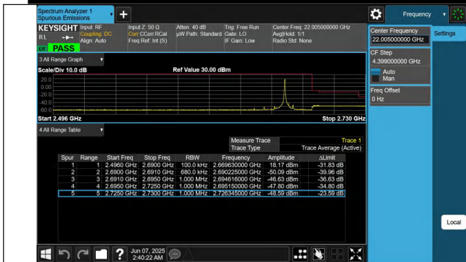
41-41-15MHz-20MHz-QPSK@QPSK-QPSK@QPSK-41319-414 90-1RB#74@75RB#0-0RB#0@100RB#0-PASS
