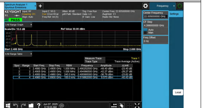
41-41-20MHz-5MHz-QPSK@QPSK-QPSK@QPSK-39750-39867- 1RB#0@100RB#0-1RB#24@25RB#0-PASS
