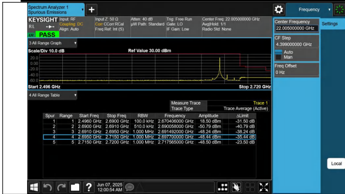
41-41-5MHz-20MHz-QPSK@QPSK-QPSK@QPSK-41373-4149 0-1RB#24@25RB#0-0RB#0@100RB#0-PASS
