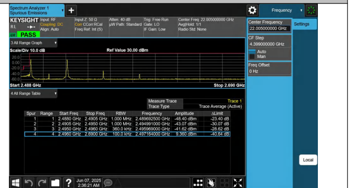
41-41-15MHz-20MHz-QPSK@QPSK-QPSK@QPSK-39728-39899 -1RB#0@75RB#0-1RB#99@100RB#0-PASS
