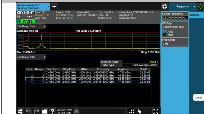
41-41-20MHz-5MHz-QPSK@QPSK-QPSK@QPSK-39750-3986 7-1RB#99@100RB#0-0RB#0@25RB#0-PASS
