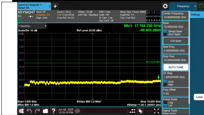
7-7-20MHz-10MHz-QPSK-QPSK-21251-21395-1RB#0-1RB#49- 3000~18000MHz-PASS
