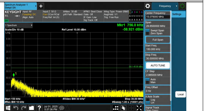
7-7-20MHz-10MHz-QPSK-QPSK-21051-21195-1RB#0-1RB#49-0. 15~30MHz-PASS
