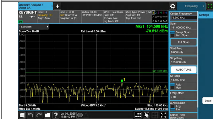
7-7-20MHz-15MHz-QPSK-QPSK-20850-21021-1RB#99-0RB#0-0.009~0.15MHz-PASS
