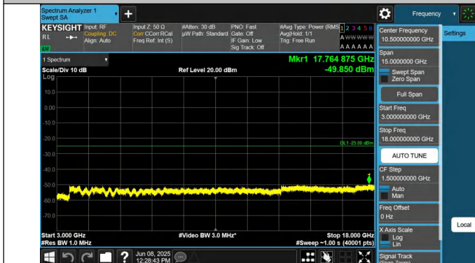
7-7-20MHz-10MHz-QPSK-QPSK-20850-20994-1RB#0-1RB#49-3000~18000MHz-PASS
