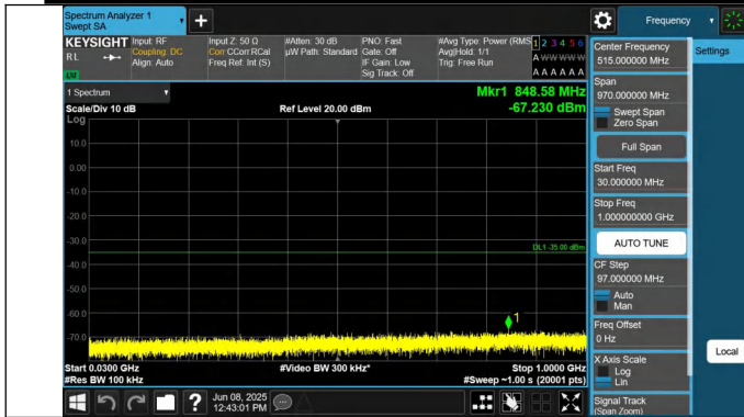
7-7-20MHz-15MHz-QPSK-QPSK-20850-21021-1RB#0-1RB#74-30~1000MHz-PASS
