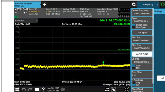
7-7-20MHz-15MHz-QPSK-QPSK-20850-21021-1RB#0-1RB#74-3000~18000MHz-PASS
