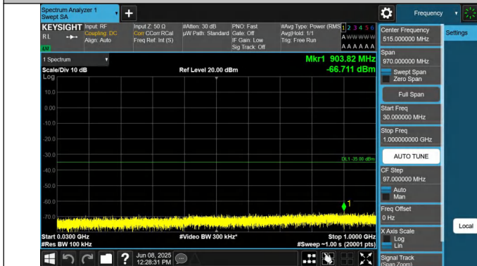
7-7-20MHz-10MHz-QPSK-QPSK-20850-20994-1RB#0-1RB#49-30~1000MHz-PASS
