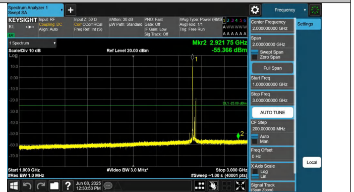
7-7-20MHz-10MHz-QPSK-QPSK-21051-21195-1RB#0-1RB#49-1 000~3000MHz-PASS
