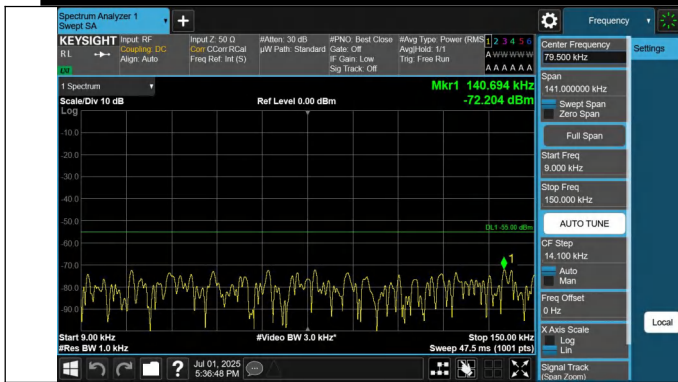
7-7-20MHz-10MHz-QPSK-QPSK-20850-20994-1RB#0-1RB#49-0.009~0.15MHz-PASS
