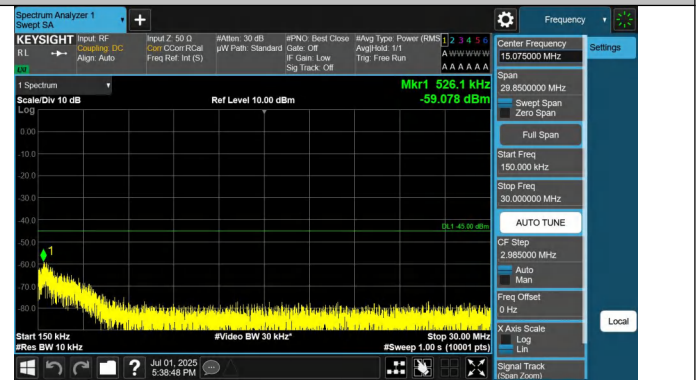
7-7-20MHz-15MHz-QPSK-QPSK-20850-21021-1RB#99-0RB#0-0.15~30MHz-PASS
