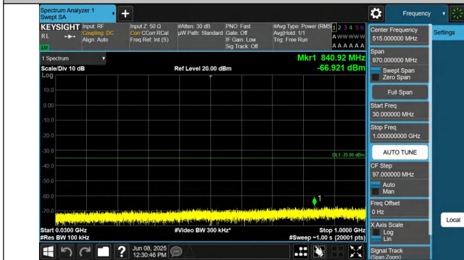
7-7-20MHz-10MHz-QPSK-QPSK-21051-21195-1RB#0-1RB#49-3 0~1000MHz-PASS
