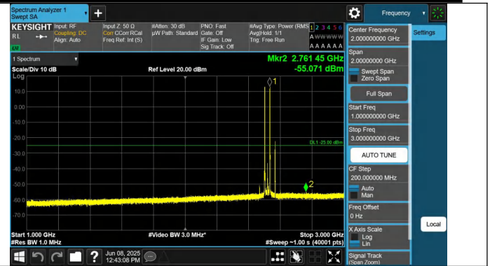
7-7-20MHz-15MHz-QPSK-QPSK-20850-21021-1RB#0-1RB#74-1000~3000MHz-PASS
