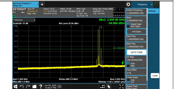
7-7-20MHz-10MHz-QPSK-QPSK-20850-20994-1RB#0-1RB#49-1000~3000MHz-PASS
