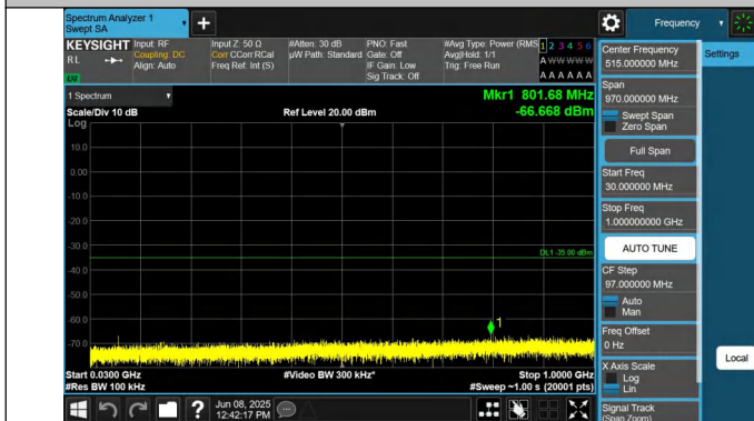
7-7-20MHz-15MHz-QPSK-QPSK-20850-21021-1RB#99-0RB#0-30~1000MHz-PASS
