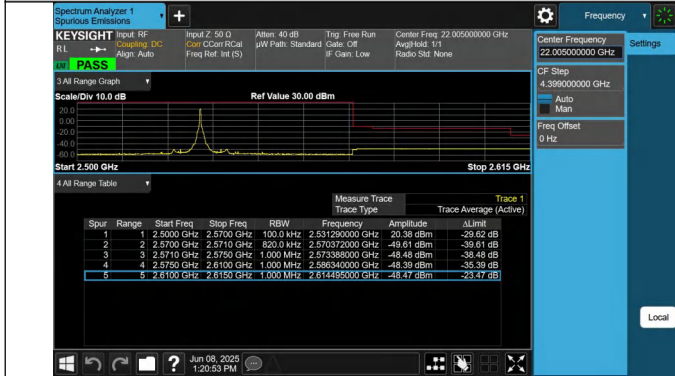
7-7-20MHz-20MHz-QPSK@QPSK-QPSK@QPSK-21152-21350-1RB#0@100RB#0-0RB#0@100RB#0-PASS
