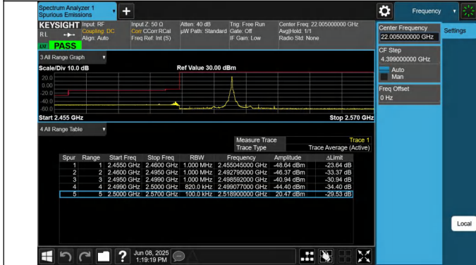
7-7-20MHz-20MHz-QPSK@QPSK-QPSK@QPSK-20850-21048-1RB#99@100RB#0-0RB#0@100RB#0-PASS
