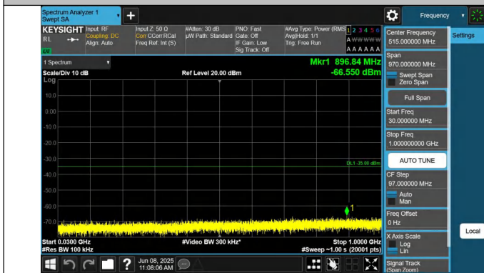
7-7-10MHz-20MHz-QPSK-QPSK-21206-21350-1RB#49-0RB#0-30~1000MHz-PASS
