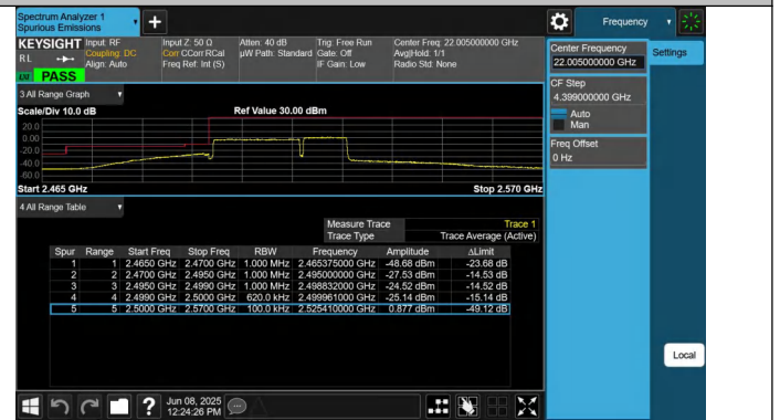
7-7-20MHz-10MHz-QPSK@QPSK-QPSK@QPSK-20850-20994-100RB#0@100RB#0-50RB#0@50RB#0-PASS
