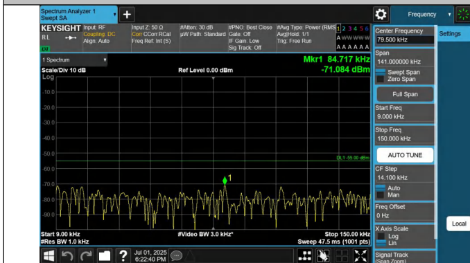
7-7-10MHz-20MHz-QPSK-QPSK-21206-21350-1RB#49-0RB#0-0.009~0.15MHz-PASS
