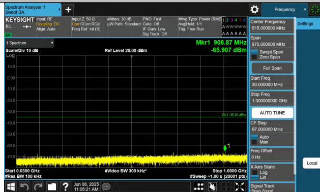
7-7-10MHz-20MHz-QPSK-QPSK-21006-21150-1RB#49-0RB#0-3 0~1000MHz-PASS
