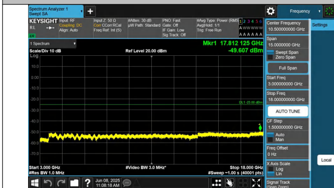
7-7-10MHz-20MHz-QPSK-QPSK-21206-21350-1RB#49-0RB#0-3000~18000MHz-PASS
