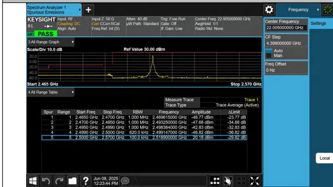
7-7-20MHz-10MHz-QPSK@QPSK-QPSK@QPSK-20850-20994-1RB#99@100RB#0-0RB#0@50RB#0-PASS
