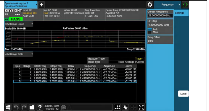
7-7-20MHz-20MHz-QPSK@QPSK-QPSK@QPSK-20850-21048-100RB#0@100RB#0-100RB#0@100RB#0-PASS
