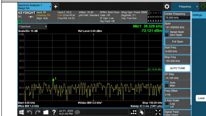
7-7-10MHz-20MHz-QPSK-QPSK-21006-21150-1RB#0-0RB#0-0.009~0.15MHz-PASS
