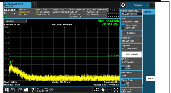
7-7-10MHz-20MHz-QPSK-QPSK-21006-21150-1RB#49-0RB#0-0. 15~30MHz-PASS
