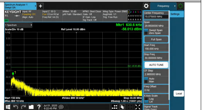
7-7-10MHz-20MHz-QPSK-QPSK-21206-21350-1RB#49-0RB#0-0.15~30MHz-PASS
