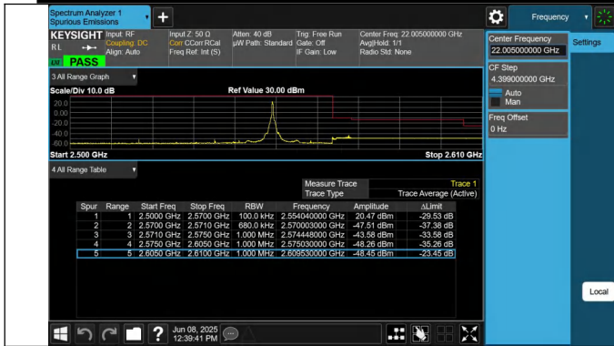
7-7-20MHz-15MHz-QPSK@QPSK-QPSK@QPSK-21201-21372-1RB#99@100RB#0-0RB#0@75RB#0-PASS
