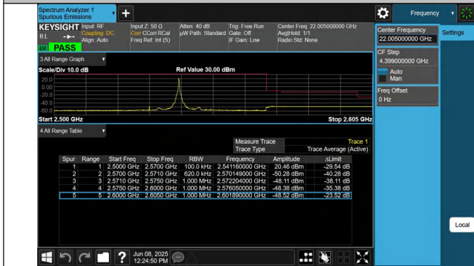
7-7-20MHz-10MHz-QPSK@QPSK-QPSK@QPSK-21251-21395-1RB#0@100RB#0-0RB#0@50RB#0-PASS
