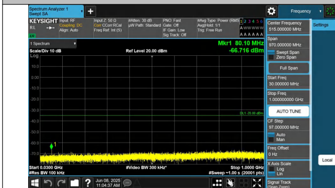
7-7-10MHz-20MHz-QPSK-QPSK-21006-21150-1RB#0-0RB#0-30~1000MHz-PASS
