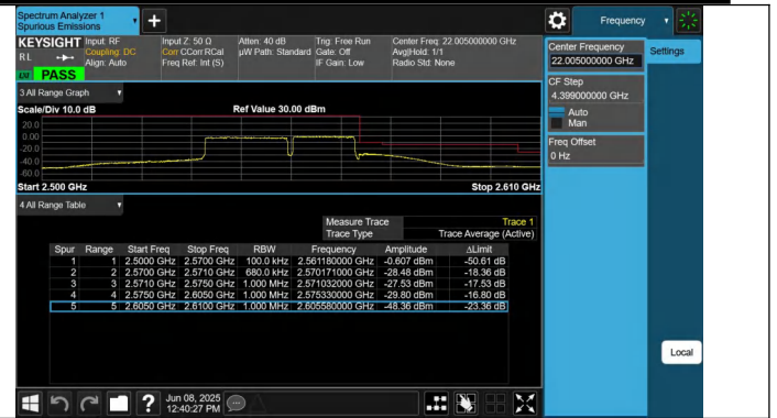
7-7-20MHz-15MHz-QPSK@QPSK-QPSK@QPSK-21201-21372-100RB#0@100RB#0-75RB#0@75RB#0-PASS
