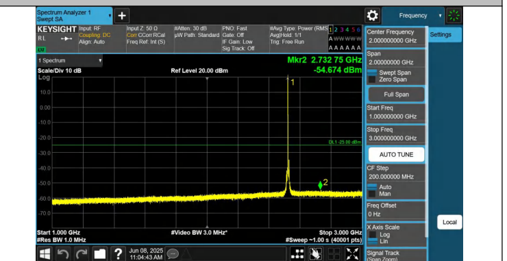
7-7-10MHz-20MHz-QPSK-QPSK-21006-21150-1RB#0-0RB#0-1000~3000MHz-PASS
