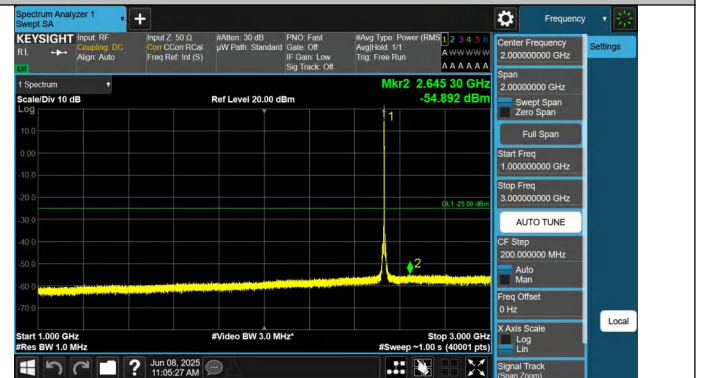
7-7-10MHz-20MHz-QPSK-QPSK-21006-21150-1RB#49-0RB#0-1 000~3000MHz-PASS
