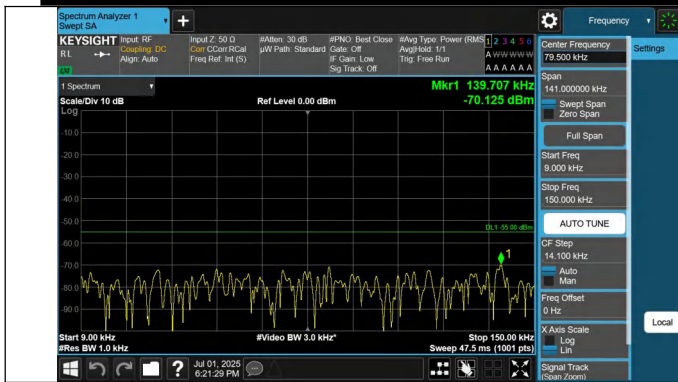
7-7-10MHz-20MHz-QPSK-QPSK-20805-20949-1RB#0-1RB#99- 0.009~0.15MHz-PASS
