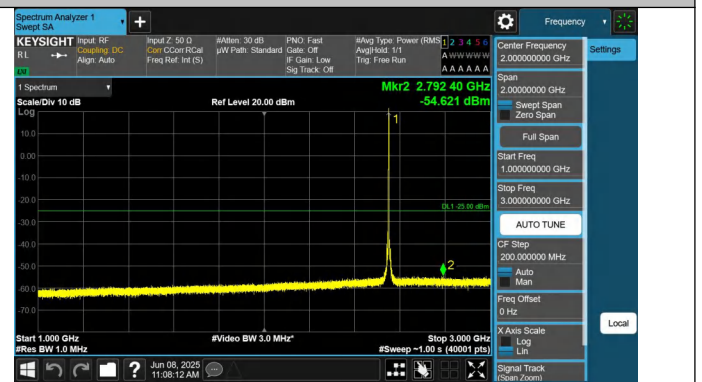
7-7-10MHz-20MHz-QPSK-QPSK-21206-21350-1RB#49-0RB#0-1000~3000MHz-PASS
