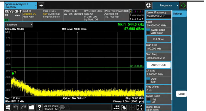
7-7-10MHz-20MHz-QPSK-QPSK-21206-21350-1RB#0-0RB#0-0.1 5~30MHz-PASS
