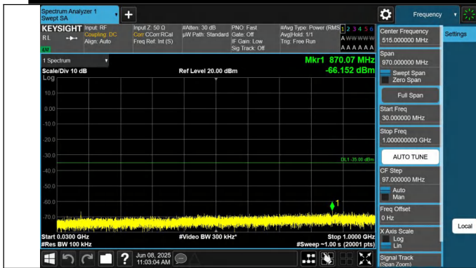
7-7-10MHz-20MHz-QPSK-QPSK-20805-20949-1RB#49-0RB#0-30~1000MHz-PASS
