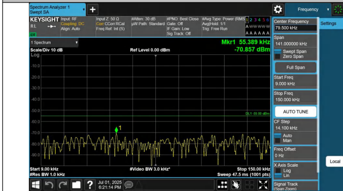
7-7-10MHz-20MHz-QPSK-QPSK-20805-20949-1RB#49-0RB#0- 0.009~0.15MHz-PASS
