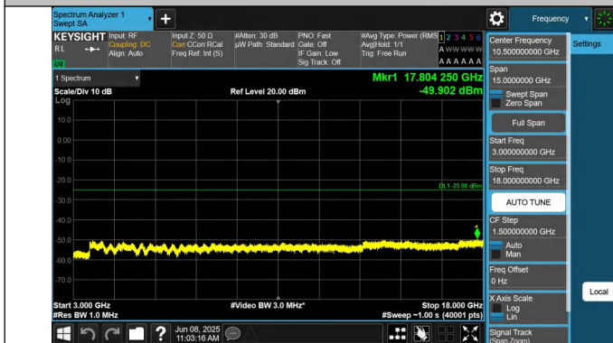
7-7-10MHz-20MHz-QPSK-QPSK-20805-20949-1RB#49-0RB#0-3000~18000MHz-PASS
