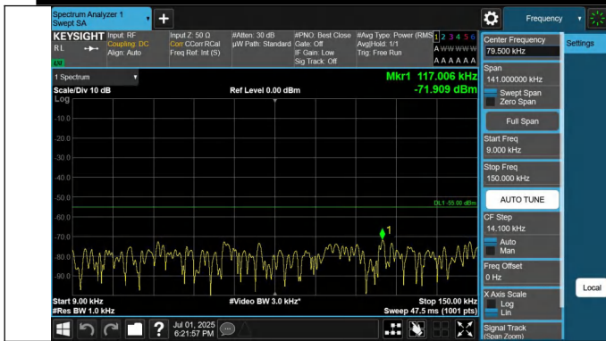
7-7-10MHz-20MHz-QPSK-QPSK-21006-21150-1RB#49-0RB#0-0 .009~0.15MHz-PASS
