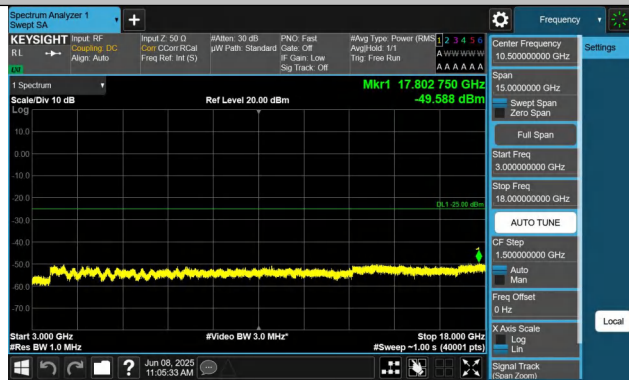
7-7-10MHz-20MHz-QPSK-QPSK-21006-21150-1RB#49-0RB#0-3 000~18000MHz-PASS
