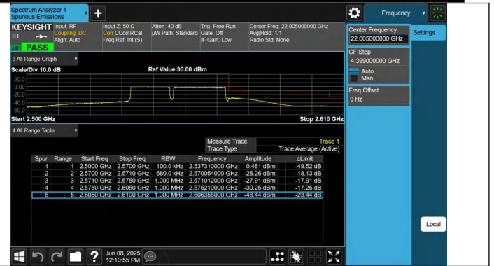
7-7-15MHz-20MHz-QPSK@QPSK-QPSK@QPSK-21179-21350-75RB#0@75RB#0-100RB#0@100RB#0-PASS
