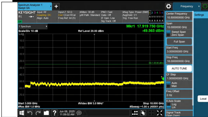
7-7-10MHz-20MHz-QPSK-QPSK-21206-21350-1RB#0-1RB#99-3000~18000MHz-PASS
