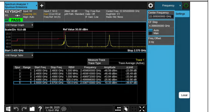
7-7-20MHz-20MHz-QPSK@QPSK-QPSK@QPSK-20850-21048-1RB#0@100RB#0-1RB#99@100RB#0-PASS
