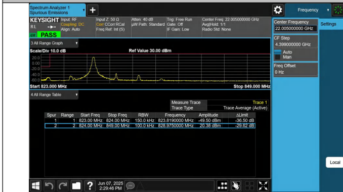
5-5-5MHz-10MHz-QPSK@QPSK-QPSK@QPSK-20428-20500-1 RB#24@25RB#0-0RB#0@50RB#0-PASS
