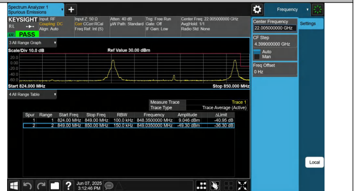
5-5-10MHz-5MHz-QPSK@QPSK-QPSK@QPSK-20550-20622-1 RB#0@50RB#0-1RB#24@25RB#0-PASS
