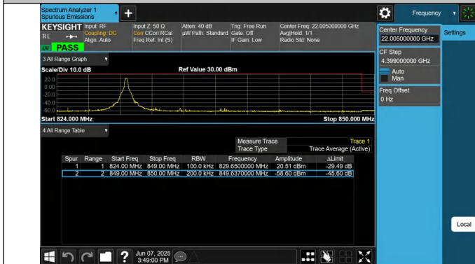
5-5-10MHz-10MHz-QPSK@QPSK-QPSK@QPSK-20501-20600- 1RB#0@50RB#0-0RB#0@50RB#0-PASS
