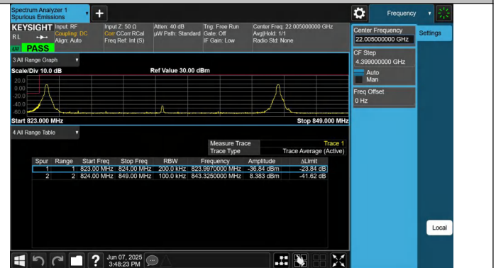
5-5-10MHz-10MHz-QPSK@QPSK-QPSK@QPSK-20450-20549-1 RB#0@50RB#0-1RB#49@50RB#0-PASS
