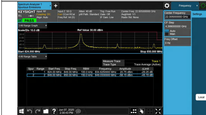
5-5-5MHz-10MHz-QPSK@QPSK-QPSK@QPSK-20528-20600-1 RB#0@25RB#0-0RB#0@50RB#0-PASS
