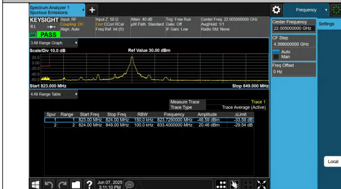
5-5-10MHz-5MHz-QPSK@QPSK-QPSK@QPSK-20450-20522-1 RB#49@50RB#0-0RB#0@25RB#0-PASS
