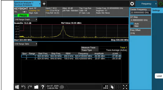
5-5-10MHz-10MHz-QPSK@QPSK-QPSK@QPSK-20450-20549- 1RB#49@50RB#0-0RB#0@50RB#0-PASS
