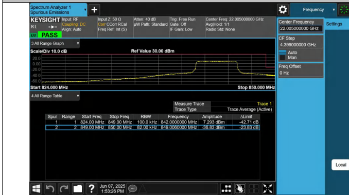
5-5-5MHz-3MHz-QPSK@QPSK-QPSK@QPSK-20595-20634-1R B#0@25RB#0-1RB#15@15RB#0-PASS
