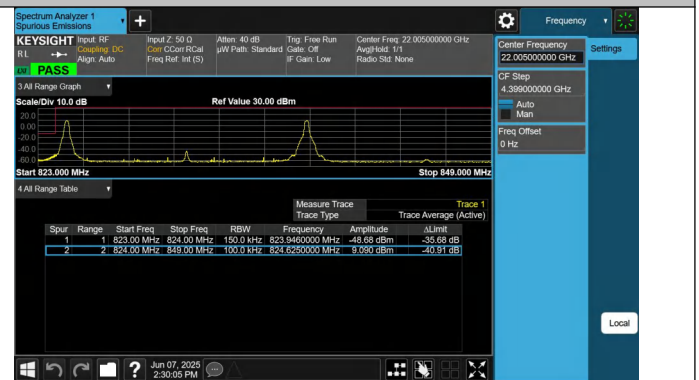
5-5-5MHz-10MHz-QPSK@QPSK-QPSK@QPSK-20428-20500-1 RB#0@25RB#0-1RB#49@50RB#0-PASS
