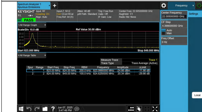
5-5-10MHz-10MHz-QPSK@QPSK-QPSK@QPSK-20450-20549- 1RB#0@50RB#0-0RB#0@50RB#0-PASS
