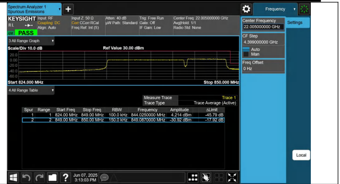
5-5-10MHz-5MHz-QPSK@QPSK-QPSK@QPSK-20550-20622-50 RB#0@50RB#0-25RB#0@25RB#0-PASS
