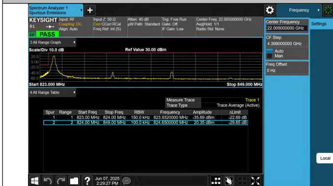
5-5-5MHz-10MHz-QPSK@QPSK-QPSK@QPSK-20428-20500-1 RB#0@25RB#0-0RB#0@50RB#0-PASS
