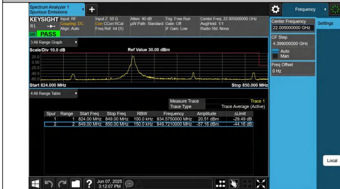
5-5-10MHz-5MHz-QPSK@QPSK-QPSK@QPSK-20550-20622-1 RB#0@50RB#0-0RB#0@25RB#0-PASS
