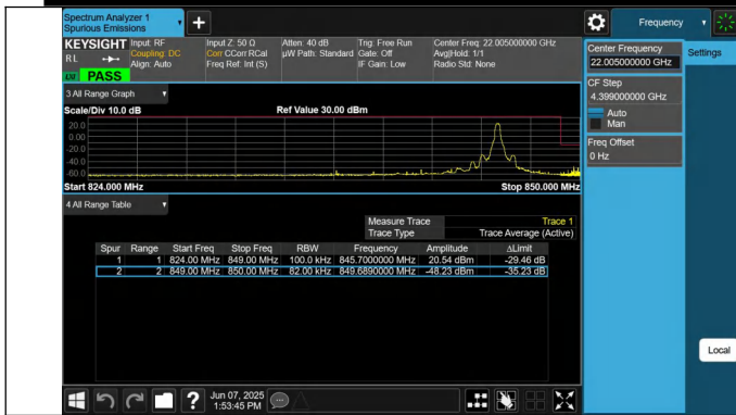
5-5-5MHz-3MHz-QPSK@QPSK-QPSK@QPSK-20595-20634-1R B#24@25RB#0-0RB#0@15RB#0-PASS
