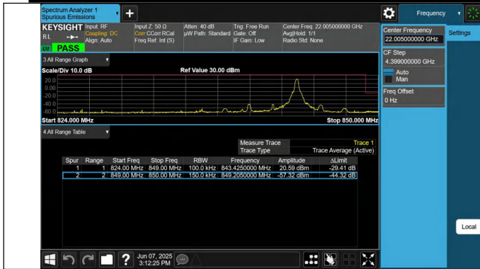
5-5-10MHz-5MHz-QPSK@QPSK-QPSK@QPSK-20550-20622-1 RB#49@50RB#0-0RB#0@25RB#0-PASS
