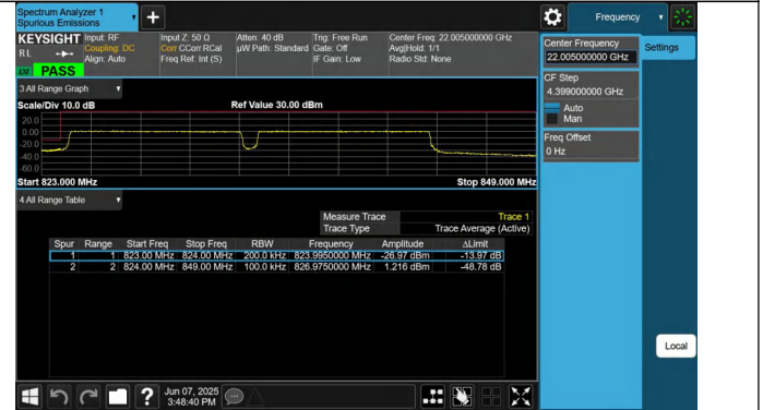
5-5-10MHz-10MHz-QPSK@QPSK-QPSK@QPSK-20450-20549-5 0RB#0@50RB#0-50RB#0@50RB#0-PASS
