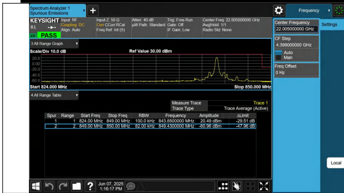
5-5-3MHz-5MHz-QPSK@QPSK-QPSK@QPSK-20586-20625-1R B#14@15RB#0-0RB#0@25RB#0-PASS
