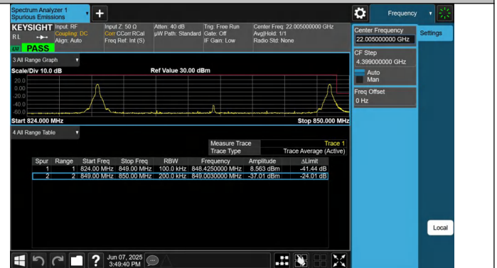
5-5-10MHz-10MHz-QPSK@QPSK-QPSK@QPSK-20501-20600-1 RB#0@50RB#0-1RB#49@50RB#0-PASS
