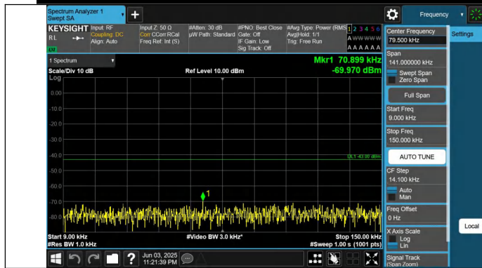
Band66-20MHz-QPSK-132322-1RB#0-0.009~0.15-PASS
