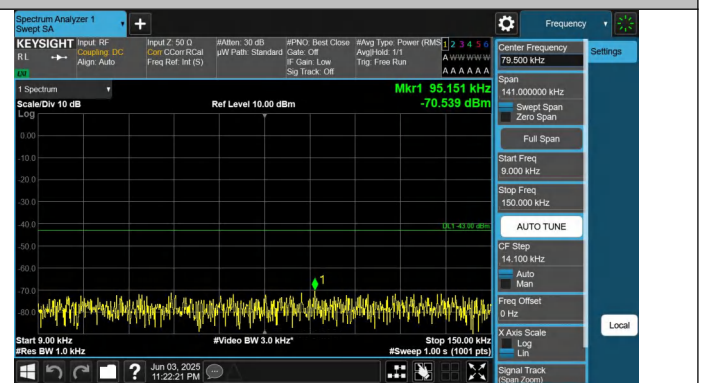
Band66-20MHz-QPSK-132322-1RB#99-0.009~0.15-PASS
