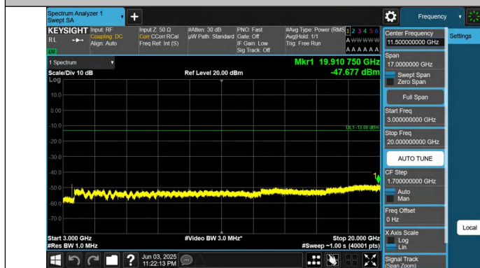
Band66-20MHz-QPSK-132322-1RB#0-3000~20000-PASS
