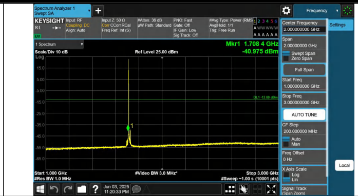
Band66-20MHz-QPSK-132072-1RB#0-1000~3000-PASS
