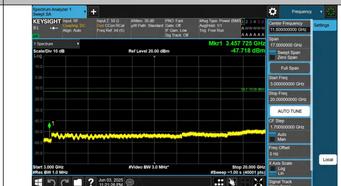
Band66-20MHz-QPSK-132072-1RB#99-3000~20000-PASS
