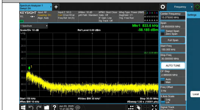
Band66-20MHz-QPSK-132072-1RB#99-0.15~30-PASS
