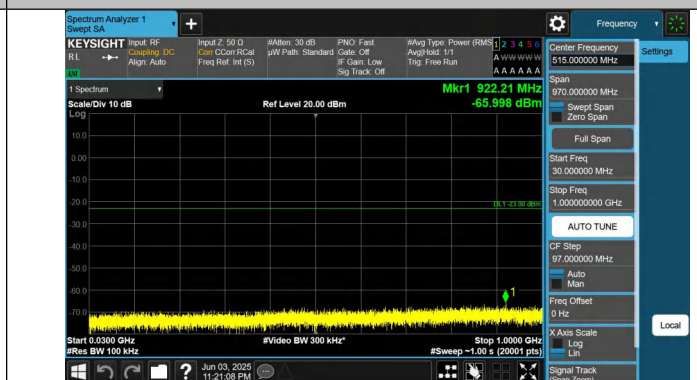
Band66-20MHz-QPSK-132072-1RB#99-30~1000-PASS
