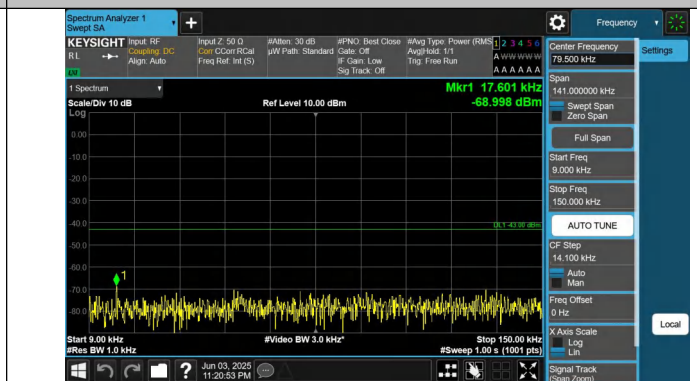
Band66-20MHz-QPSK-132072-1RB#99-0.009~0.15-PASS
