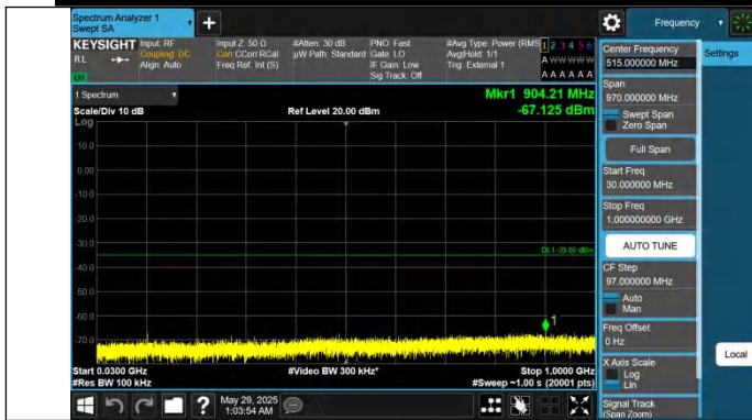
Band41-10MHz-QPSK-39700-1RB#0-30~1000-PASS
