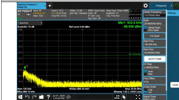
Band41-10MHz-QPSK-39700-1RB#49-0.15~30-PASS
