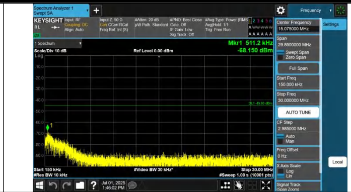
Band41-15MHz-QPSK-41515-1RB#0-0.15~30-PASS
