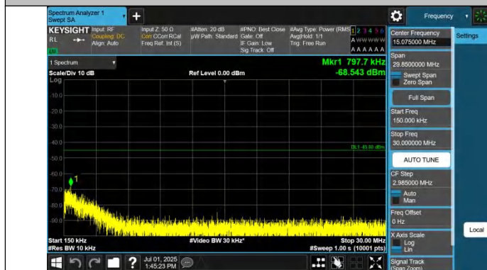
Band41-15MHz-QPSK-39725-1RB#74-0.15~30-PASS
