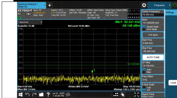
Band41-15MHz-QPSK-41515-1RB#0-0.009~0.15-PASS
