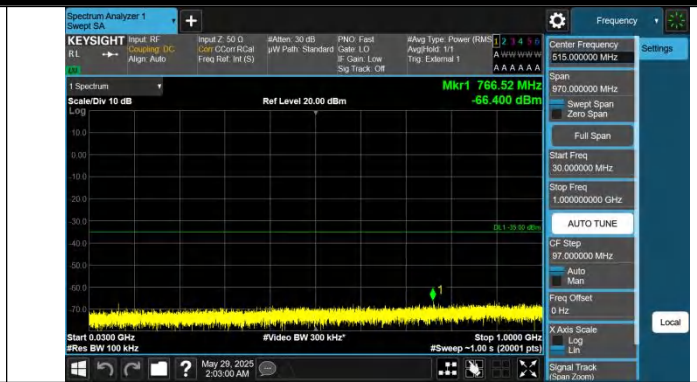
Band41-20MHz-QPSK-39750-1RB#99-30~1000-PASS
