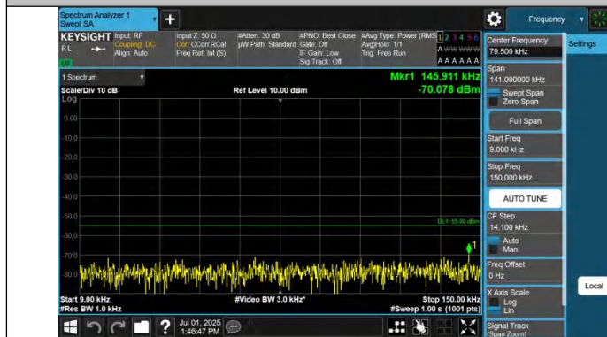
Band41-20MHz-QPSK-40620-1RB#0-0.009~0.15-PASS
