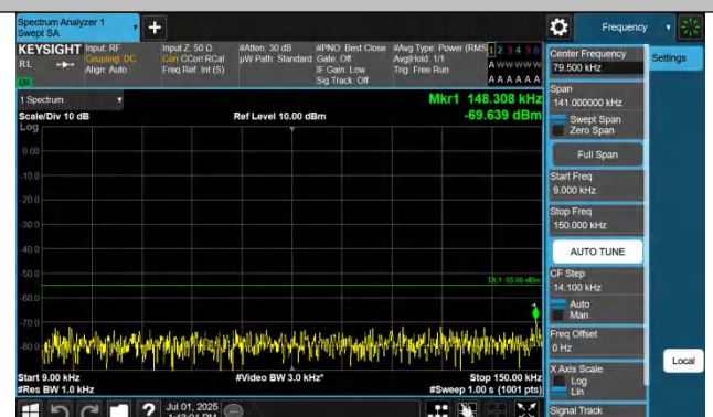
Band41-5MHz-QPSK-40620-1RB#24-0.009~0.15-PASS
