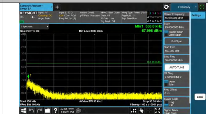
Band41-5MHz-QPSK-41565-1RB#0-0.15~30-PASS
