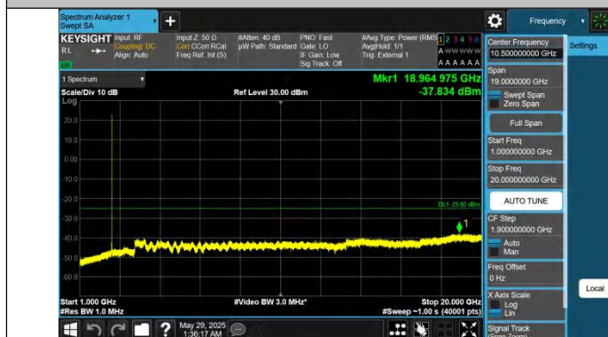
Band41-15MHz-QPSK-39725-1RB#74-1000~20000-PASS
