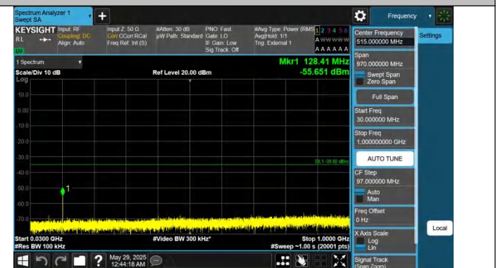
Band41-5MHz-QPSK-41565-1RB#24.30~1000-PASS
