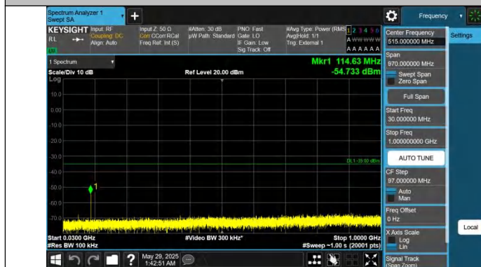
Band41-15MHz-QPSK-41515-1RB#0-30~1000-PASS
