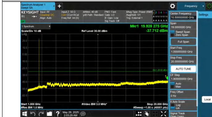
Band41-20MHz-QPSK-39750-1RB#99-1000~20000-PASS
