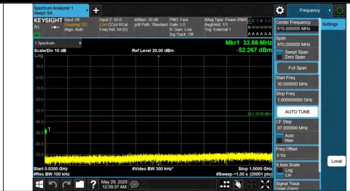
Band41-5MHz-QPSK-40620-1RB#24-30~1000-PASS
