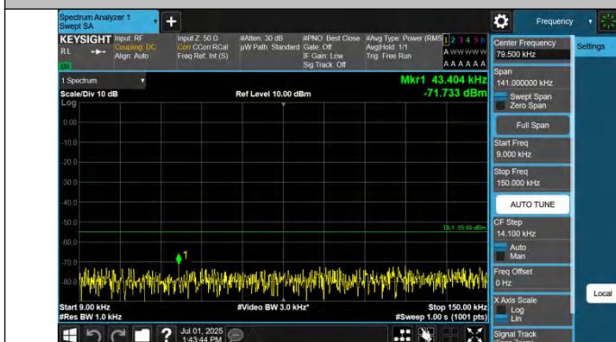
Band41-10MHz-QPSK-39700-1RB#0-0.009~0.15-PASS
