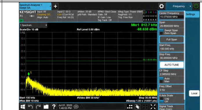
Band41-20MHz-QPSK-40620-1RB#0-0.15~30-PASS
