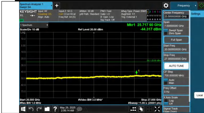
Band41-20MHz-QPSK-40620-1RB#0-20000-PASS
