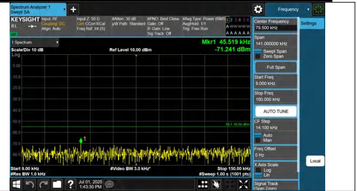
Band41-5MHz-QPSK-41565-1RB#24.0.009~0.15-PASS
