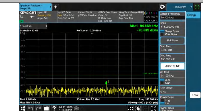
Band41-15MHz-QPSK-41515-1RB#74-0.009~0.15-PASS
