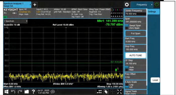
Band41-20MHz-QPSK-40620-1RB#99-0.009~0.15-PASS
