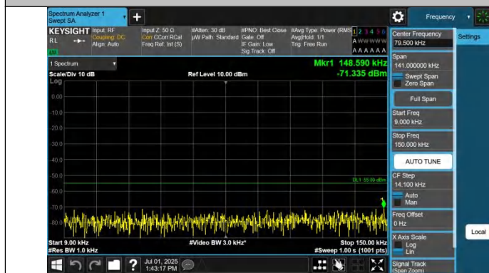
Band41-5MHz-QPSK-41565-1RB#0-0.009~0.15-PASS
