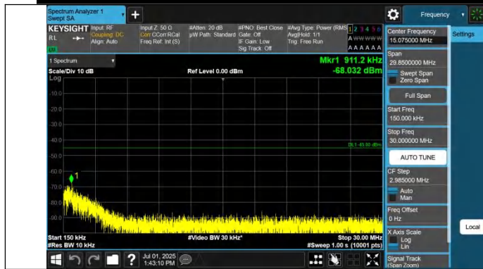
Band41-5MHz-QPSK-40620-1RB#24-0.15~30-PASS
