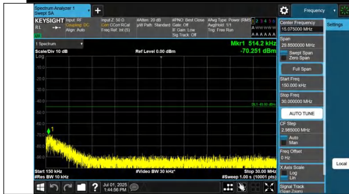
Band41-10MHz-QPSK-41540-1RB#49-0.15~30-PASS
