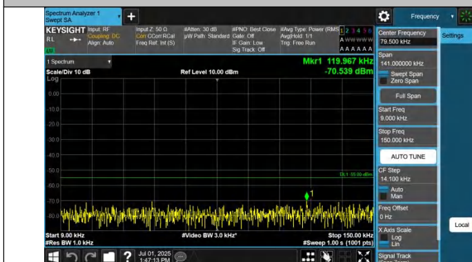
Band41-20MHz-QPSK-41490-1RB#0-0.009~0.15-PASS
