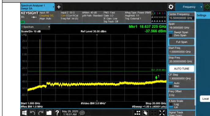
Band41-10MHz-QPSK-41540-1RB#49-1000~20000-PASS
