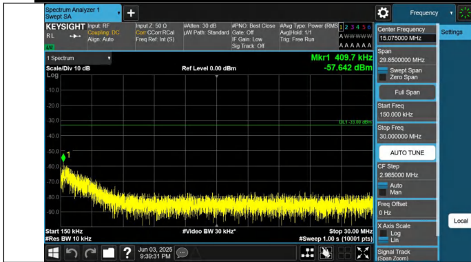
Band25-15MHz-QPSK-26365-1RB#74-0.15~30-PASS
