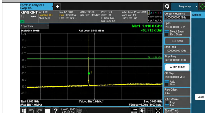
Band25-10MHz-QPSK-26640-1RB#49-1000~3000-PASS
