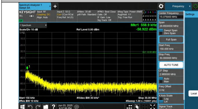
Band25-15MHz-QPSK-26115-1RB#74-0.15~30-PASS
