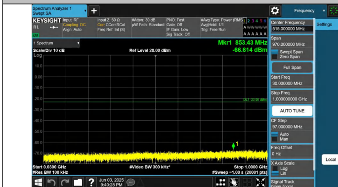
Band25-15MHz-QPSK-26615-1RB#0-30~1000-PASS
