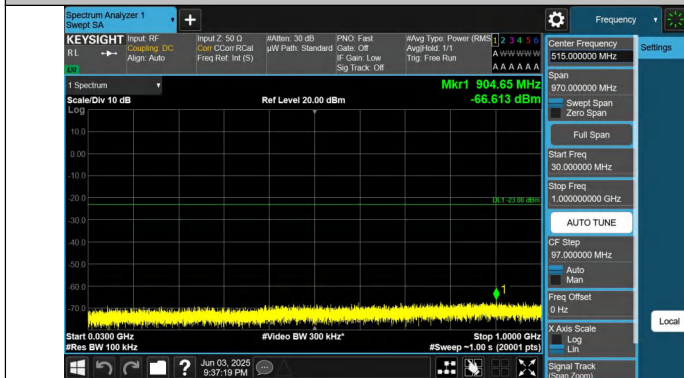
Band25-15MHz-QPSK-26115-1RB#0-30~1000-PASS
