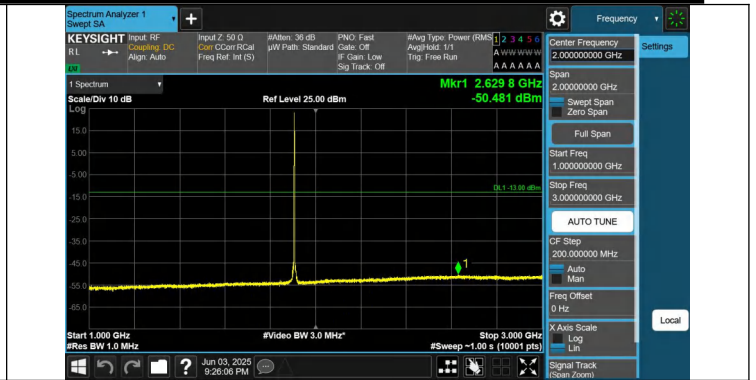
Band25-10MHz-QPSK-26640-1RB#0-1000~3000-PASS
