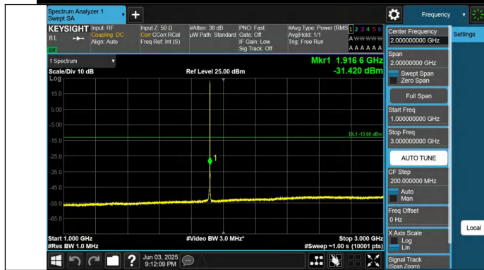
Band25-5MHz-QPSK-26665-1RB#24-1000~3000-PASS
