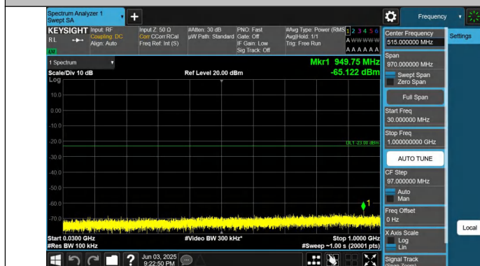
Band25-10MHz-QPSK-26090-1RB#0-30~1000-PASS
