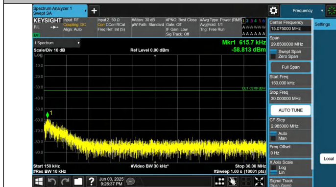
Band25-10MHz-QPSK-26640-1RB#49-0.15~30-PASS
