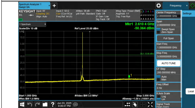
Band25-15MHz-QPSK-26365-1RB#74-1000~3000-PASS
