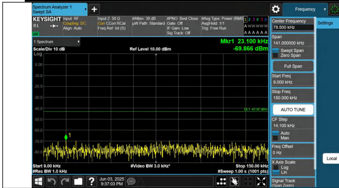
Band25-15MHz-QPSK-26115-1RB#0-0.009~0.15-PASS
