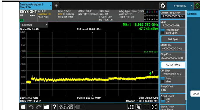
Band25-10MHz-QPSK-26640-1RB#0-3000~20000-PASS
