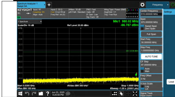
Band25-10MHz-QPSK-26640-1RB#0-30~1000-PASS
