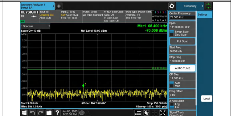
Band25-10MHz-QPSK-26640-1RB#49-0.009~0.15-PASS
