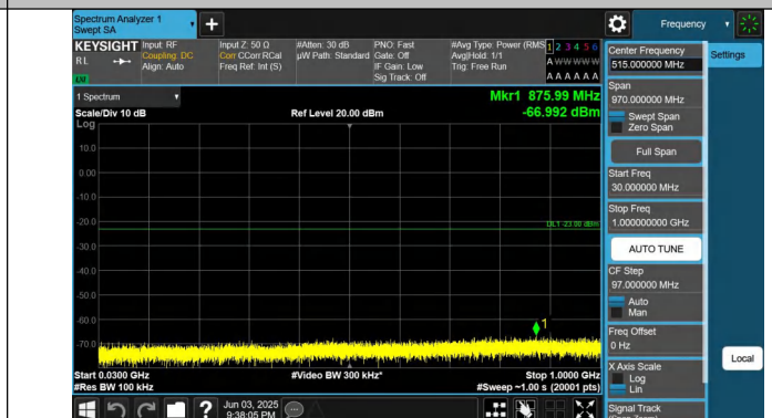
Band25-15MHz-QPSK-26115-1RB#74-30~1000-PASS
