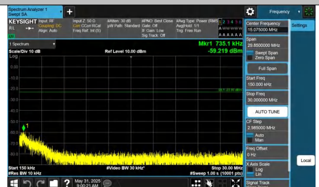
Band5-3MHz-QPSK-20415-1RB#0-0.15~30-PASS
