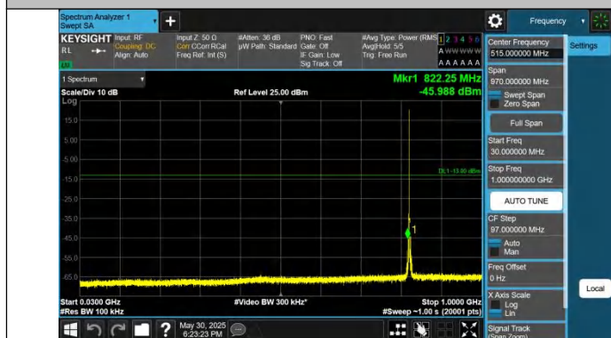
Band5-5MHz-QPSK-20425-1RB#0-30~1000-PASS
