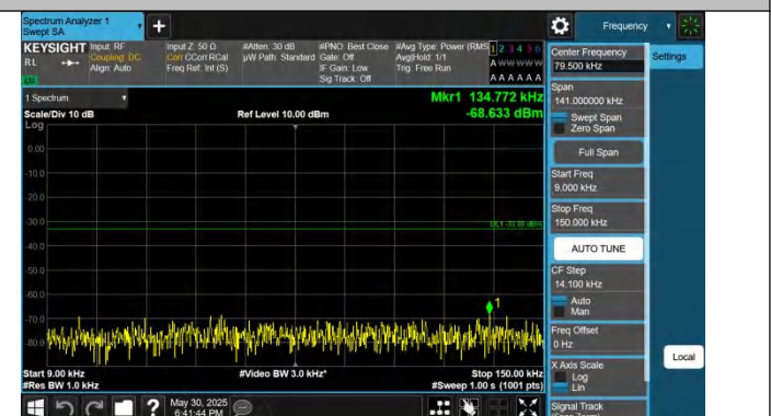
Band5-10MHz-QPSK-20450-1RB#49-0.009~0.15-PASS
