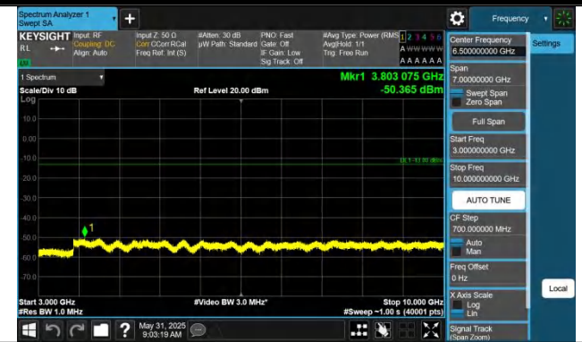
Band5-3MHz-QPSK-20525-1RB#14-3000~10000-PASS
