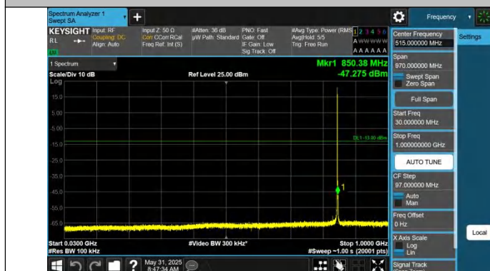
Band5-1.4MHz-QPSK-20643-1RB#0-30~1000-PASS
