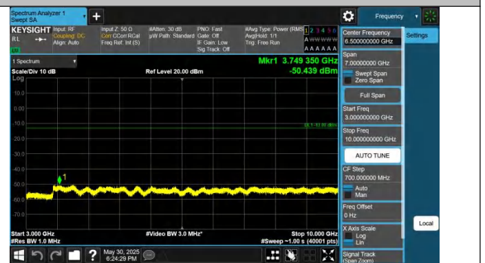
Band5-5MHz-QPSK-20425-1RB#24-3000~10000-PASS
