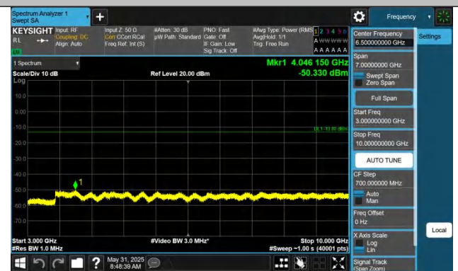
Band5-1.4MHz-QPSK-20643-1RB#5-3000~10000-PASS
