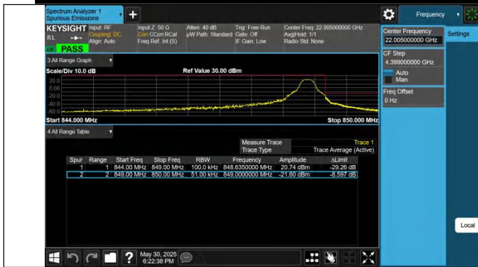
Band5-5MHz-QPSK-20625-1RB#24-PASS
