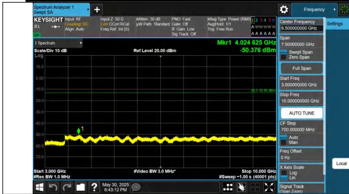
Band5-10MHz-QPSK-20525-1RB#0-3000~10000-PASS
