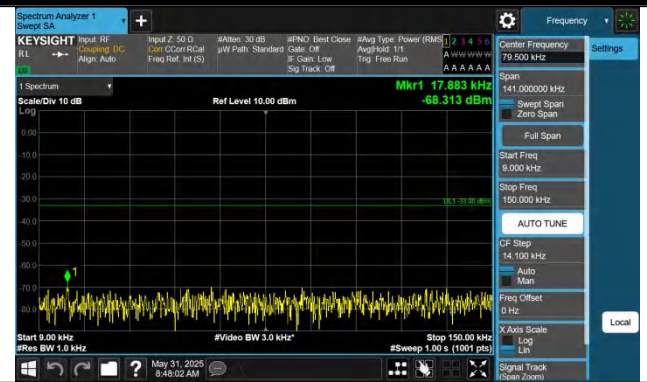
Band5-1.4MHz-QPSK-20643-1RB#5-0.009~0.15-PASS
