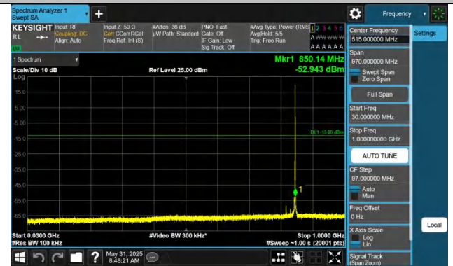
Band5-1.4MHz-QPSK-20643-1RB#5-30~1000-PASS
