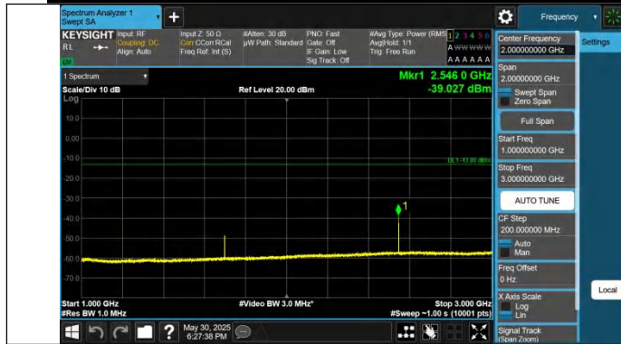
Band5-5MHz-QPSK-20625-1RB#24-1000~3000-PASS
