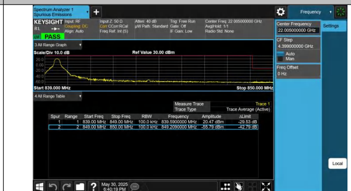
Band5-10MHz-QPSK-20600-1RB#0-PASS
