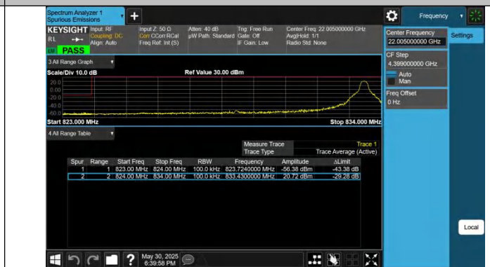
Band5-10MHz-QPSK-20450-1RB#49-PASS
