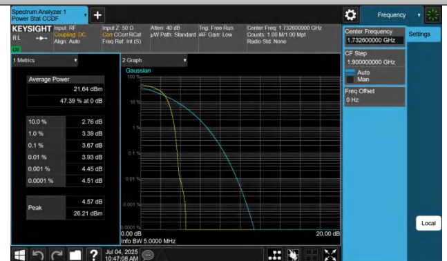
Band4-1413-2-PASS
