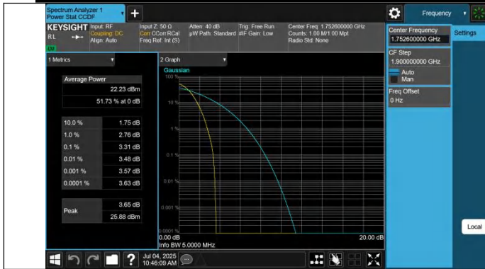
Band4-1513-1-PASS
