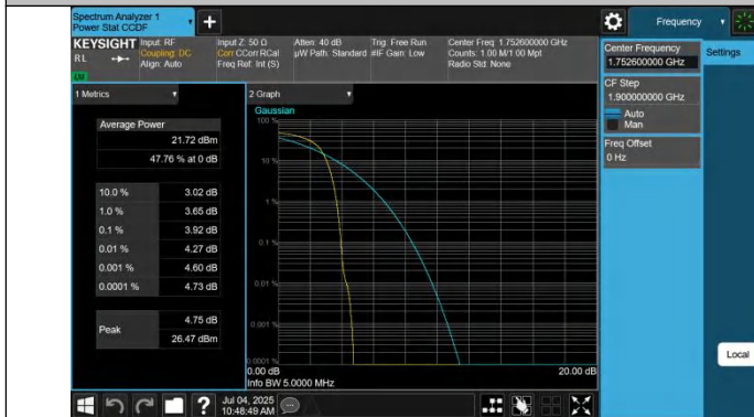
Band4-1513-3-PASS
