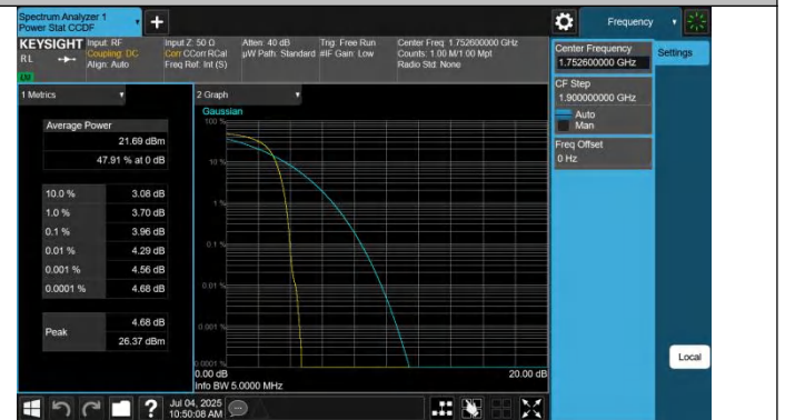
Band4-1513-4-PASS
