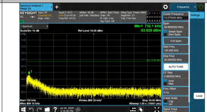
Band4-1413-1-0.15~30MHz-PASS
