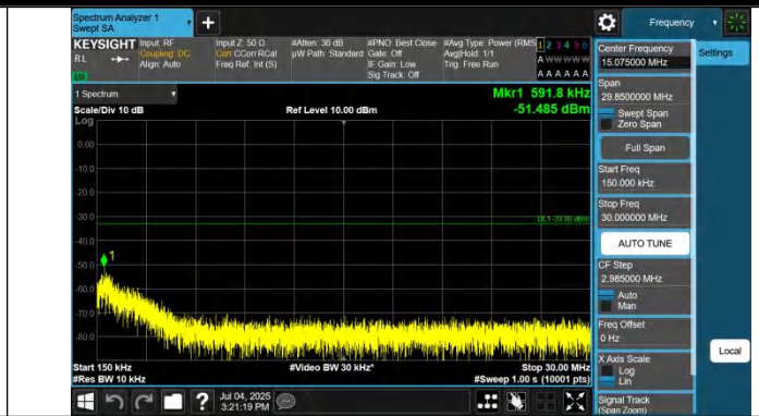
Band4-1312-4-0.15~30MHz-PASS
