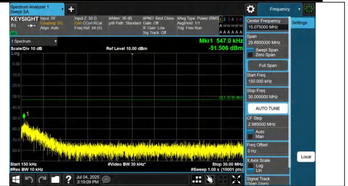
Band4-1513-0.15~30MHz-PASS
