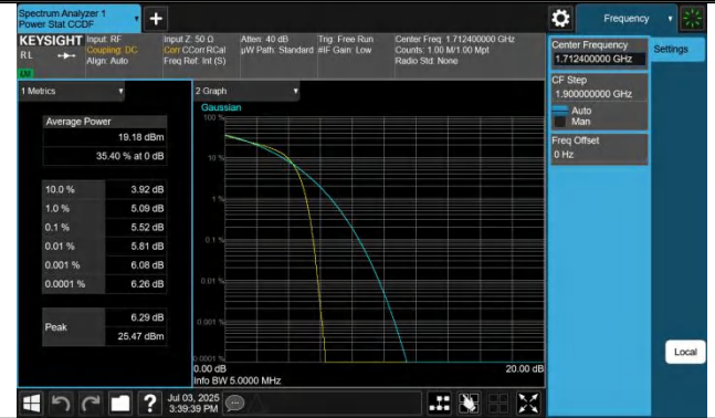
Band4-1312-2-PASS
