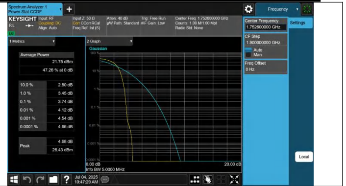
Band4-1513-2-PASS
