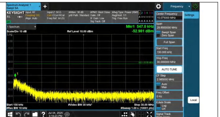
Band4-1312-1-0.15~30MHz-PASS
