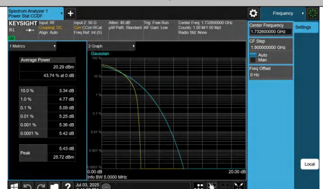
Band4-1413-3-PASS
