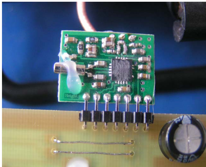
RF Board Front View
