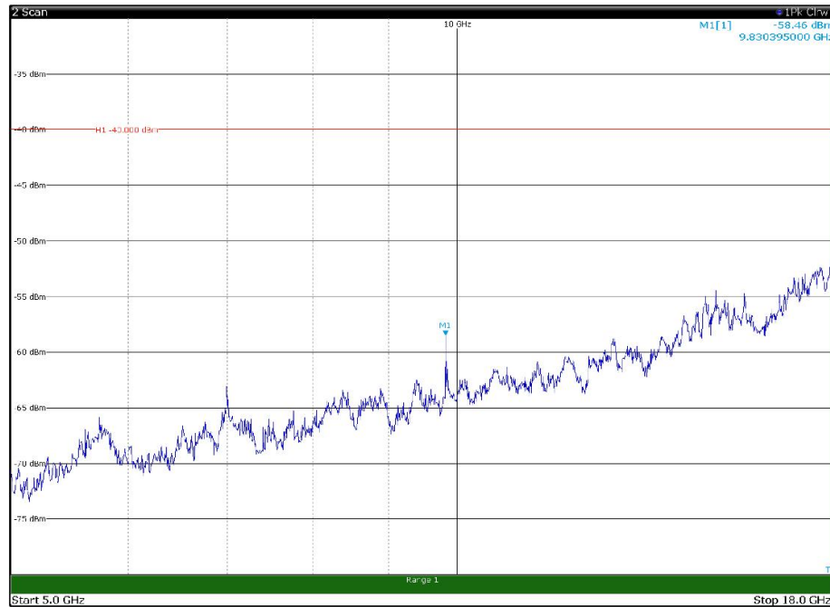
Channel: BOTTOM, Modulation: 256QAM, BW=5MHz, Range: 5GHz - 18GHz, Polarization: Horizontal
