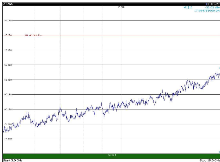
Channel: BOTTOM, Modulation: 256QAM, BW=5MHz, Range: 5GHz - 18GHz, Polarization: Vertical
