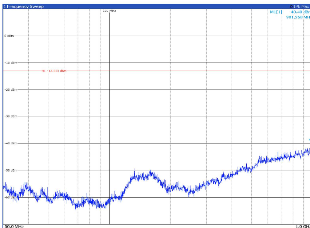
Channel: MIDDLE, Modulation: 64QAM, BW=80MHz, Range: 30MHz - 1GHz, Polarization: Vertical
