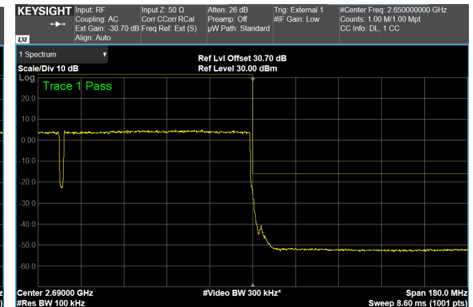
High Band Edge, 2 Carriers, Modulation: 64QAM, BW=80MHz
