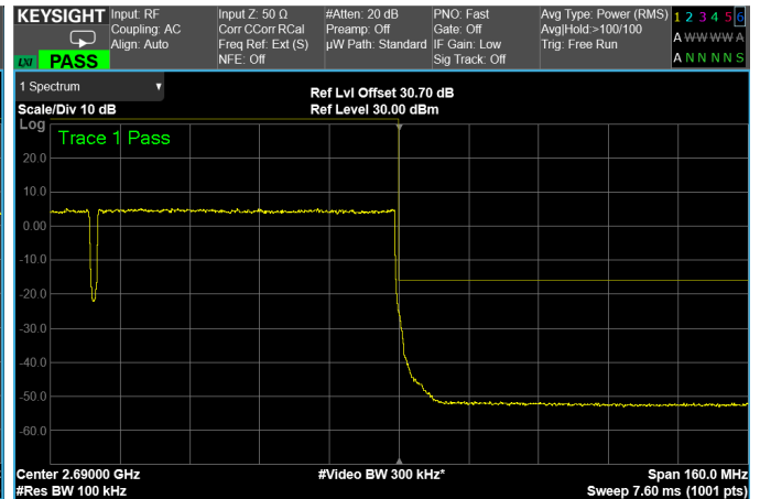
High Band Edge, 2 Carriers, Modulation: 64QAM, BW=70MHz
