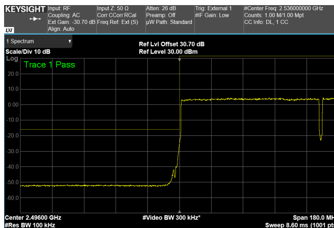
Low Band Edge, 2 Carriers, Modulation: 64QAM, BW=80MHz
