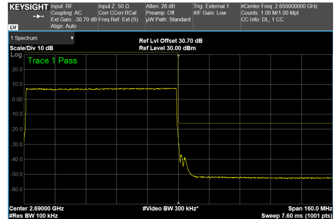
High Band Edge, 1 Carrier, Modulation: 64QAM, BW=80MHz
