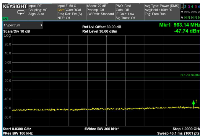
Channel: TOP, Modulation: 64QAM, BW=5MHz, Range: Lower
