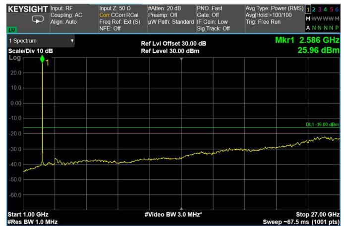
Channel: MIDDLE, Modulation: 64QAM, BW=5MHz, Range: Upper
