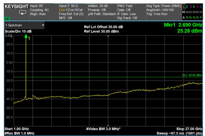
Channel: TOP, Modulation: 64QAM, BW=5MHz, Range: Upper
