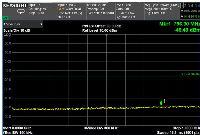
Channel: MIDDLE, Modulation: 64QAM, BW=5MHz, Range: Lower
