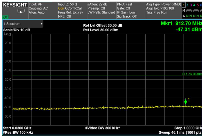
Channel: BOTTOM, Modulation: 64QAM, BW=5MHz, Range: Lower
