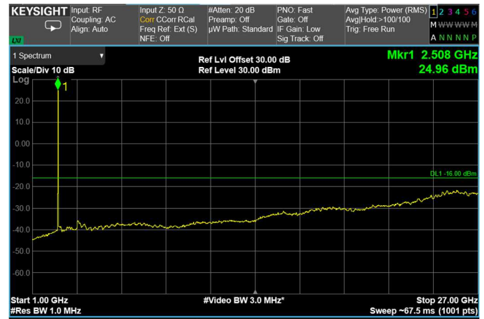
Channel: BOTTOM, Modulation: 64QAM, BW=5MHz, Range: Upper
