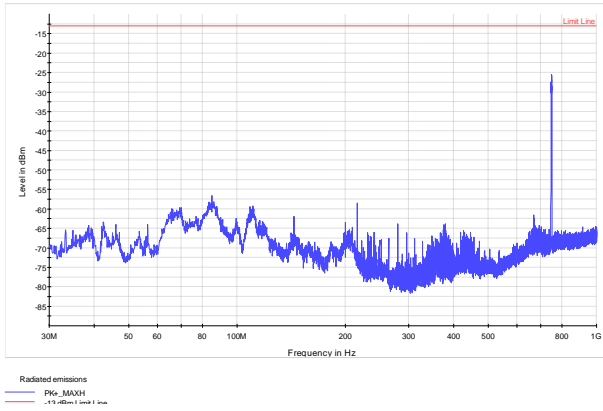
Figure 8.5-4: Radiated spurious emissions within 30 MHz to 1 GHz – Low Channel (LTE700)
