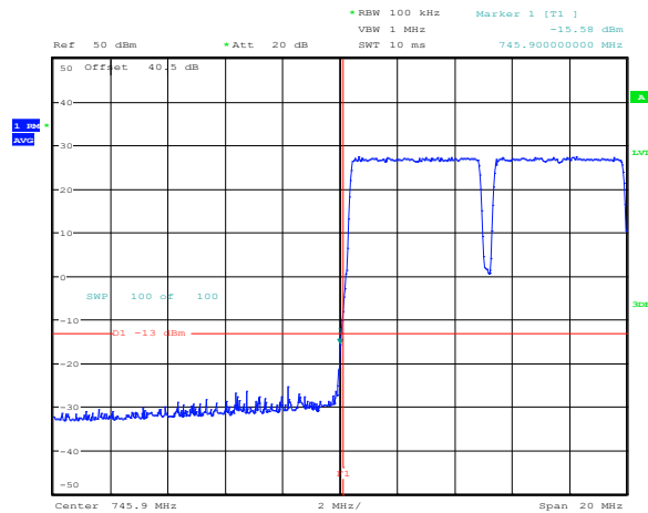
Figure 8.4-40: Conducted lower band edge at 746 MHz at AGC threshold + 3 dB (intermodulation) (LTE700)
