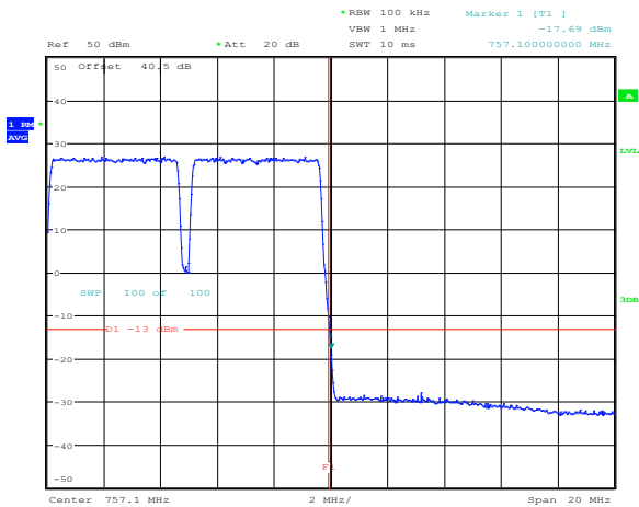
Figure 8.4-47: Conducted upper band edge at 758 MHz at AGC threshold (intermodulation) (LTE700)
