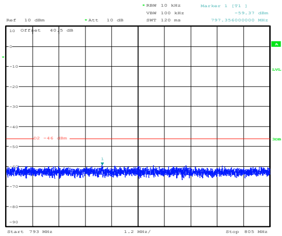
Figure 8.4-14: Conducted spurious emissions 793-805 MHz for mid channel (LTE700)
