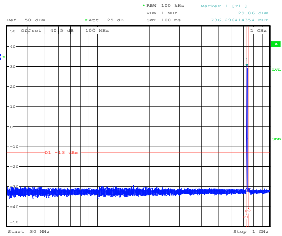
Figure 8.4-2: Conducted spurious emissions below 1 GHz for mid channel (SMR700)
