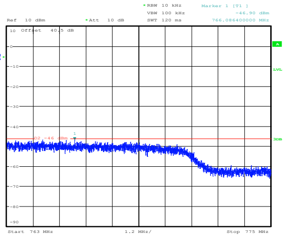
Figure 8.4-17: Conducted spurious emissions 763-775 MHz for mid channel (LTE700)
