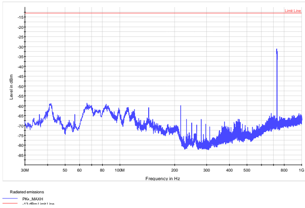
Figure 8.5-1: Radiated spurious emissions within 30 MHz to 1 GHz – Low Channel (SMR700)
