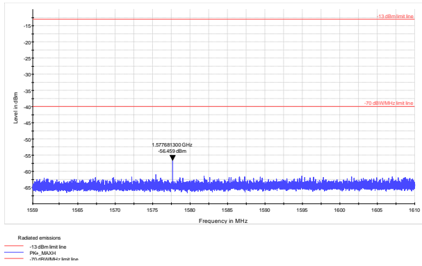
Figure 8.5-13: Radiated spurious emissions within 1559- 1610 MHz – Low Channel (LTE700)
