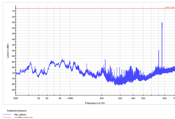
Figure 8.5-6: Radiated spurious emissions within 30 MHz to 1 GHz – High Channel (LTE700)
