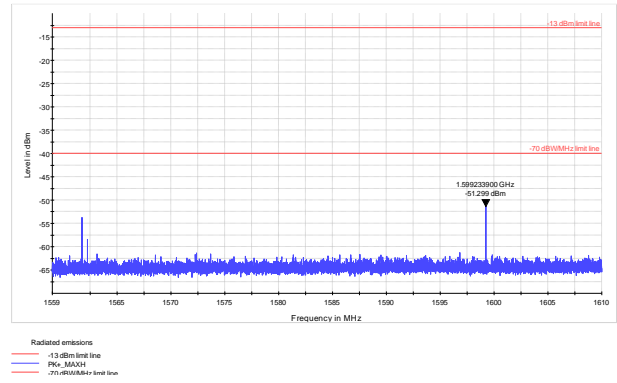
Figure 8.5-14: Radiated spurious emissions within 1559- 1610 MHz – Mid Channel (LTE700)
