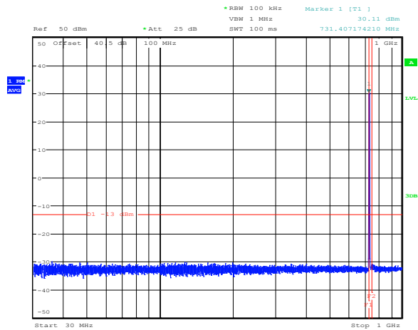
Figure 8.4-3: Conducted spurious emissions below 1 GHz for high channel (SMR700)
