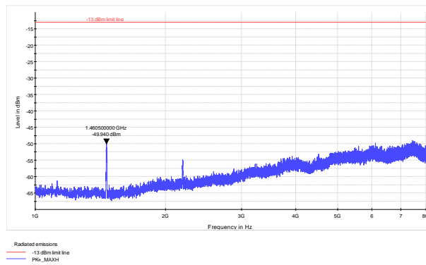
Figure 8.5-7: Radiated spurious emissions within 1 to 8 GHz – Low Channel (SMR700)
