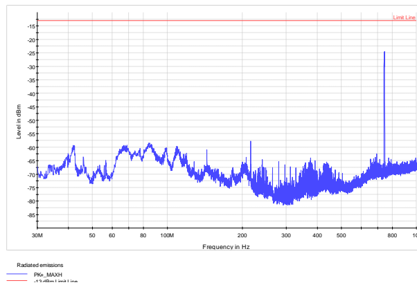
Figure 8.5-3: Radiated spurious emissions within 30 MHz to 1 GHz – High Channel (SMR700)
