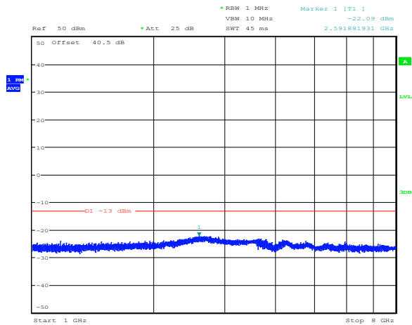
Figure 8.4-9: Conducted spurious emissions above 1 GHz for high channel (SMR700)
