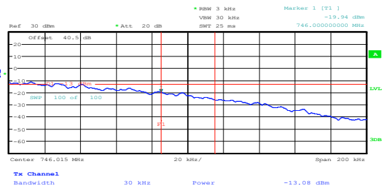
Figure 8.4-28: Conducted upper band edge at 746 MHz at AGC threshold + 3 dB (SMR700)
