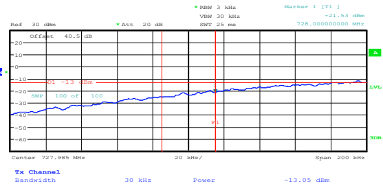
Figure 8.4-20: Conducted lower band edge at 728 MHz at AGC threshold + 3 dB (SMR700)
