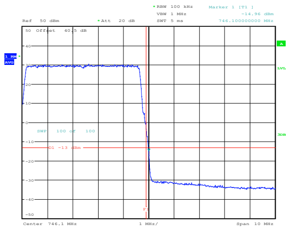
Figure 8.4-27: Conducted upper band edge at 746 MHz at AGC threshold (SMR700)
