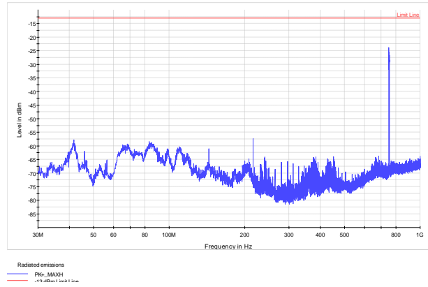
Figure 8.5-5: Radiated spurious emissions within 30 MHz to 1 GHz – Middle Channel (LTE700)
