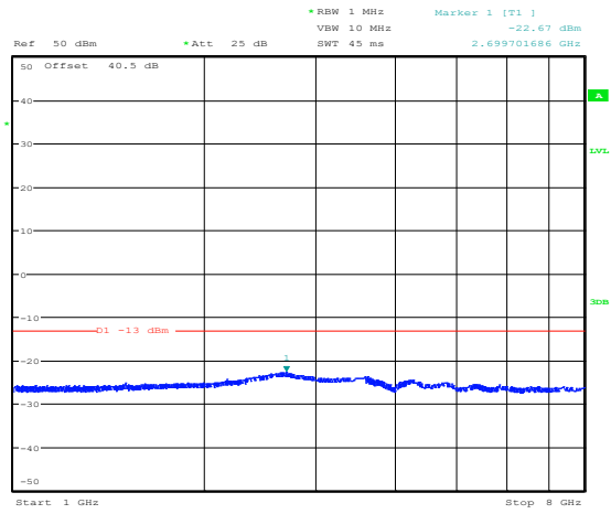
Figure 8.4-11: Conducted spurious emissions above 1 GHz for mid channel (LTE700)
