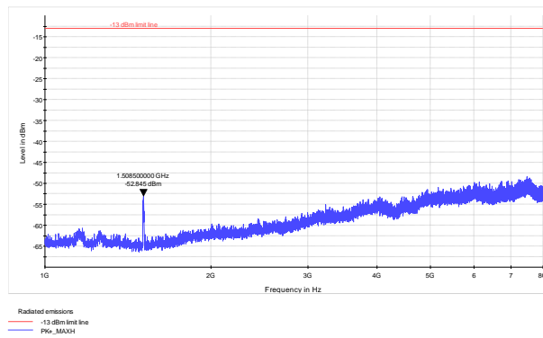
Figure 8.5-10: Radiated spurious emissions within 1 to 8 GHz – Low Channel (LTE700)
