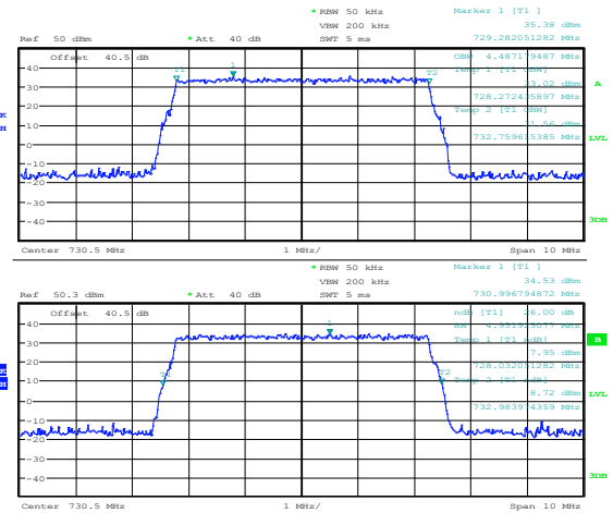
Figure 8.6-2: 99% OBW and 26 dB EBW at the output of the EUT at AGC threshold, low channel (SMR700)
