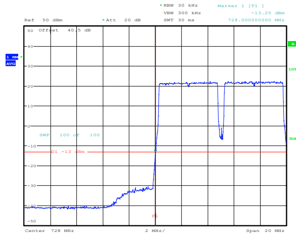
Figure 8.4-36: Conducted lower band edge at 728 MHz at AGC threshold + 3 dB (intermodulation) (SMR700)
