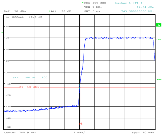
Figure 8.4-24: Conducted lower band edge at 746 MHz at AGC threshold + 3 dB (LTE700)
