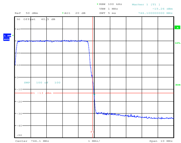
Figure 8.4-28: Conducted upper band edge at 746 MHz at AGC threshold + 3 dB (SMR700)
