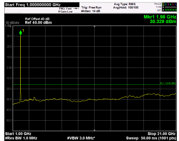
AWGN SIGNAL, 1GHz-21GHz
