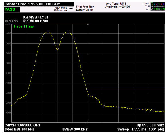
MSK Signal, Nominal Input Signal +3dB, High Band Edge, 2 Carrier
