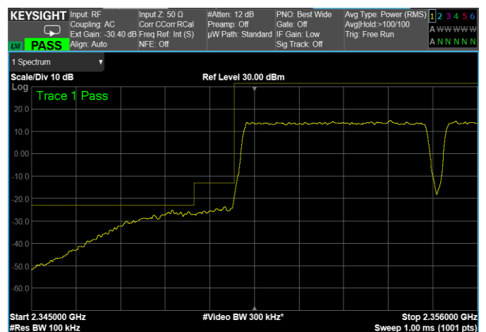
5 MHz signal, Low Band Edge, 2 carriers, nominal input signal + 3dB
