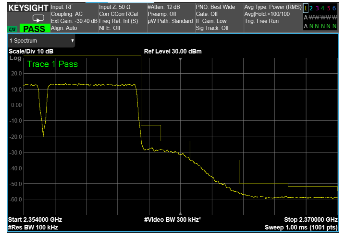
5 MHz signal, High Band Edge, 2 carriers, nominal input signal + 3dB
