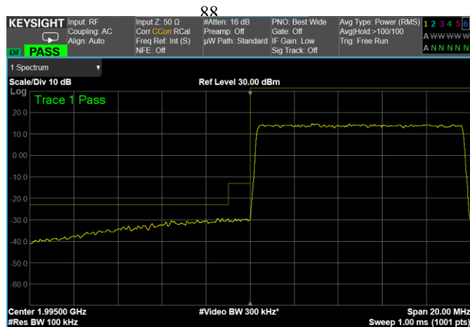
10 MHz signal, Low Band Edge, 1 carrier, nominal input signal + 3dB
