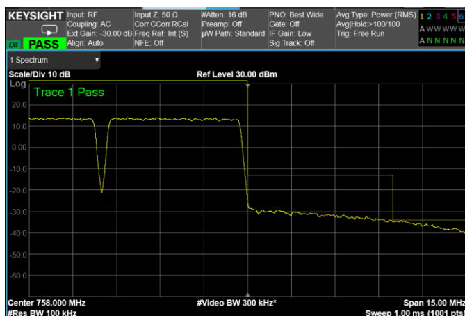
5 MHz signal, High Band Edge, 2 carriers, nominal input signal
