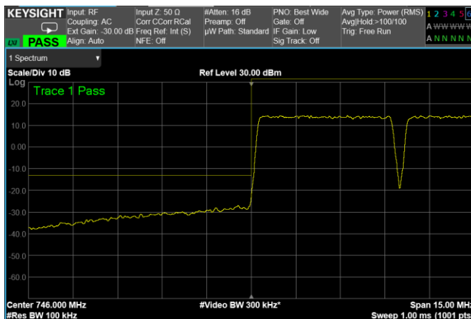
5 MHz signal, Low Band Edge, 2 carriers, nominal input signal
