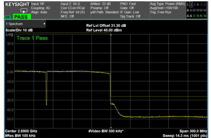
100 MHz signal, High Band Edge, 2 carrier, nominal input signal + 3dB
