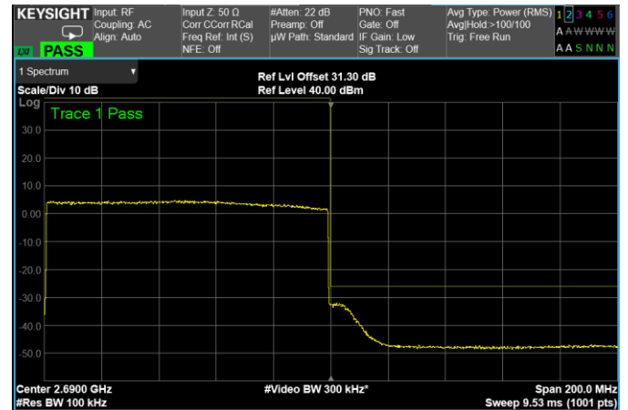
100 MHz signal, High Band Edge, 1 carrier, nominal input signal + 3dB
