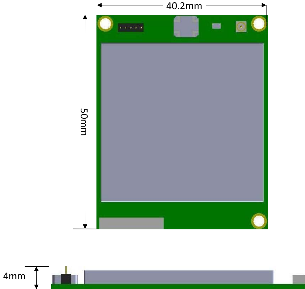
Figure 1 - Outline Drawing of the FS-GM102
