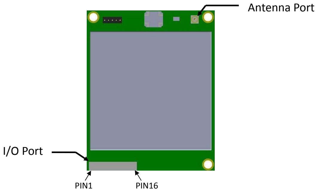
Figure 2 – 0.80mm pitch 16 pin I/O connector
