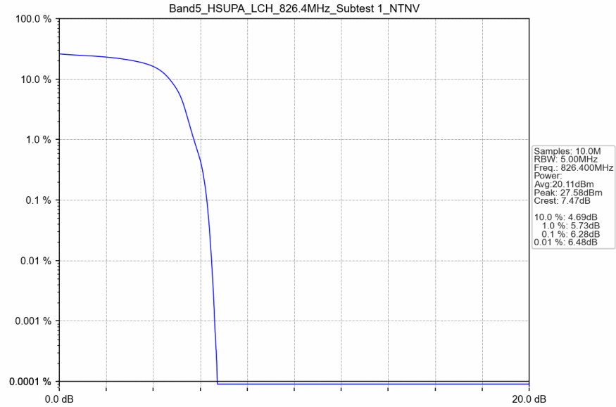
Band5_HSUPA_LCH_826.4MHz_Subtest 1_NTNV
