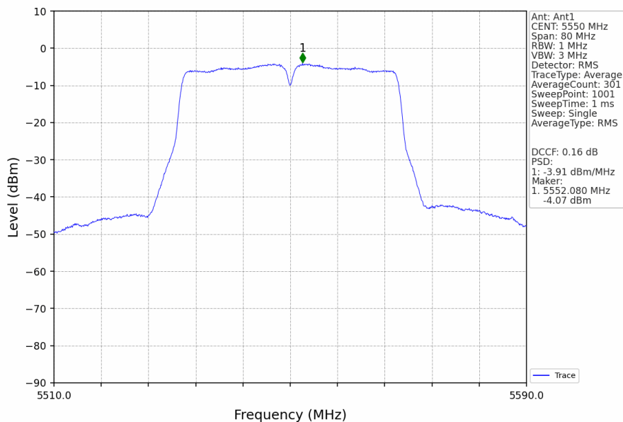
802.11ac(VHT40)_MCH_5550MHz_Ant1_NTNV
