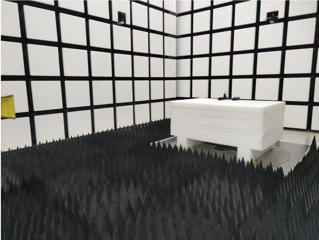
Radiated Emissions Above 1G rear View-M2
