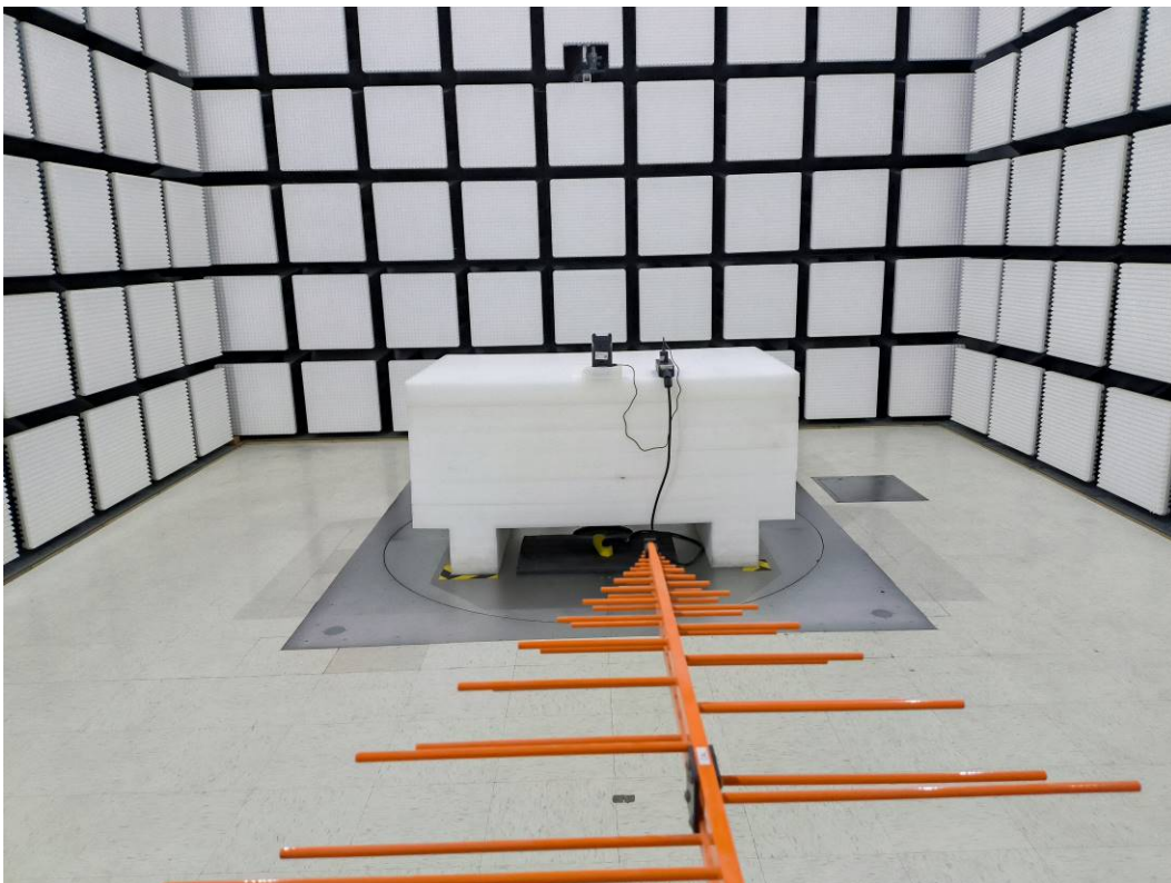
Radiated Emissions Below 1G rear View-M4
