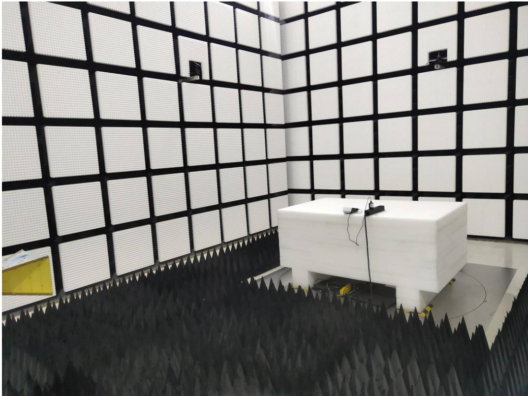
Radiated Emissions Above 1G rear View-M6
