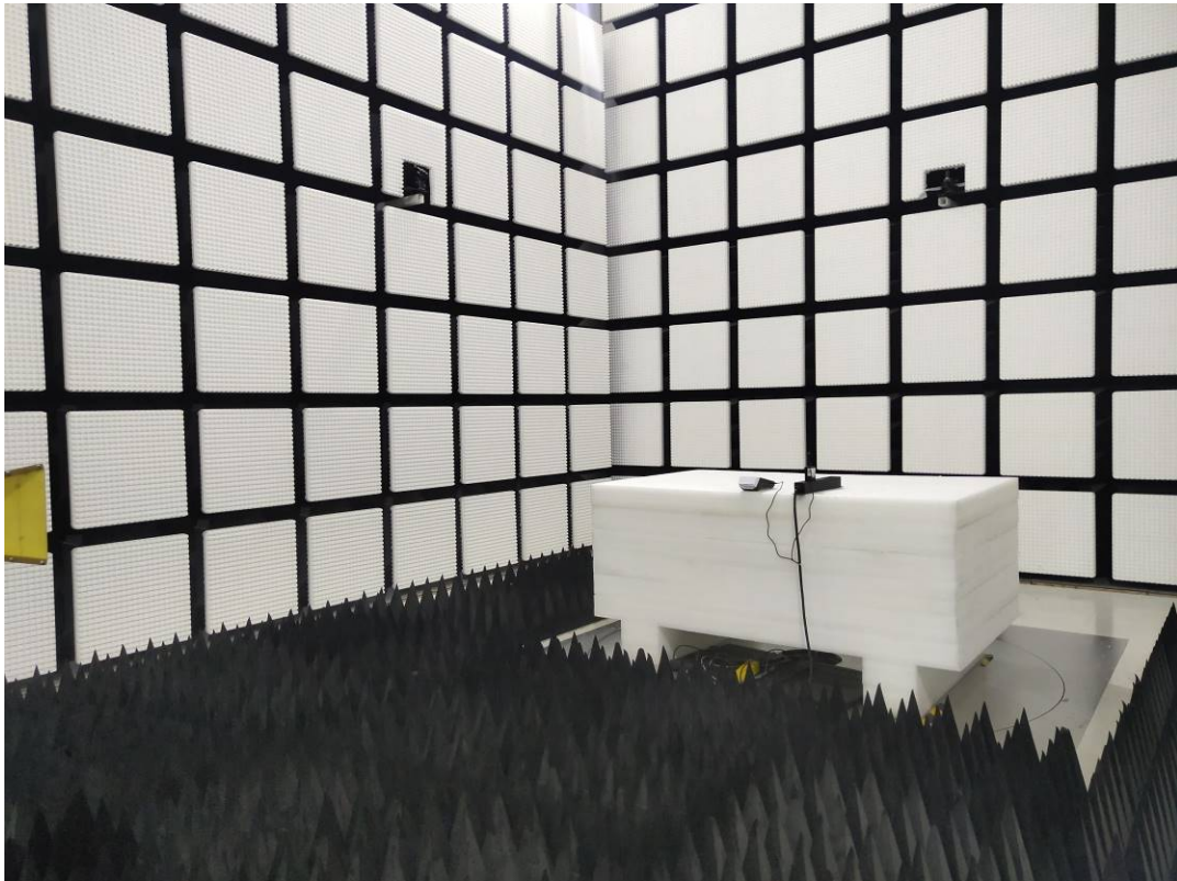
Radiated Emissions Above 1G rear View-M5
