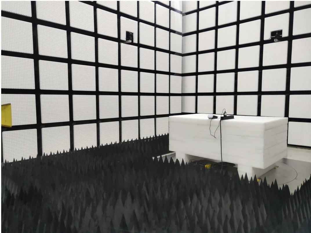
Radiated Emissions Above 1G rear View-M7
