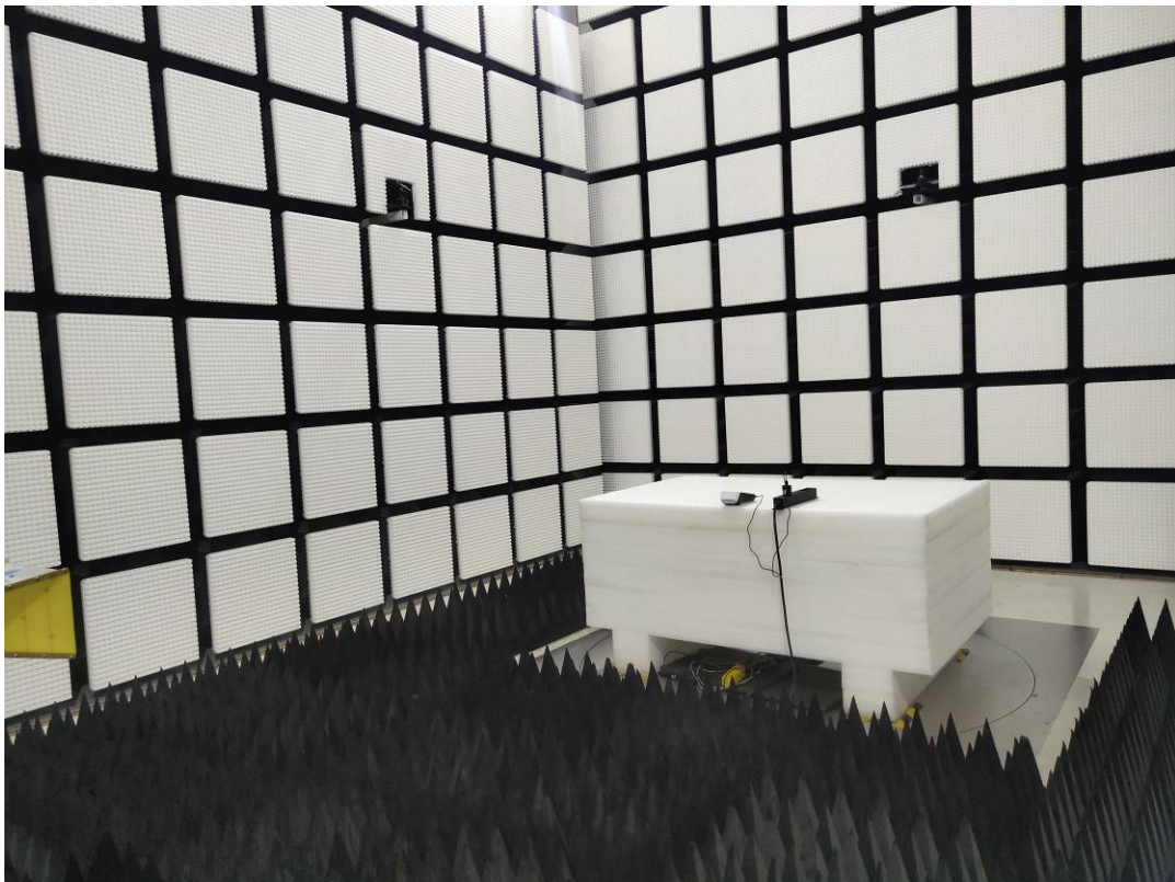
Radiated Emissions Above 1G rear View-M4
