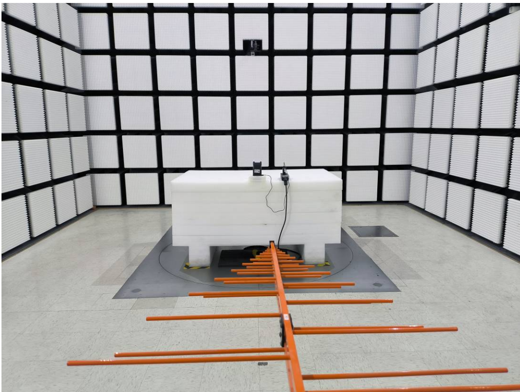
Radiated Emissions Below 1G rear View-M7
