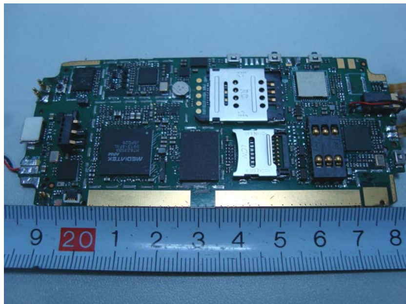
EUT – Main Board without Shielded-Cover Components View
