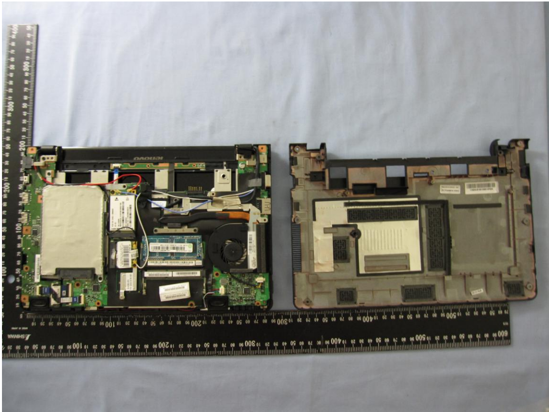
bottom side with RT3090 Module
