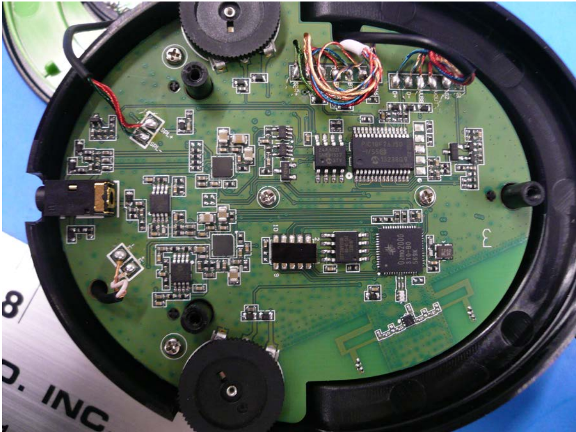
Figure 1: Internal Photo of Ear Force Stealth 500X RX - Top
