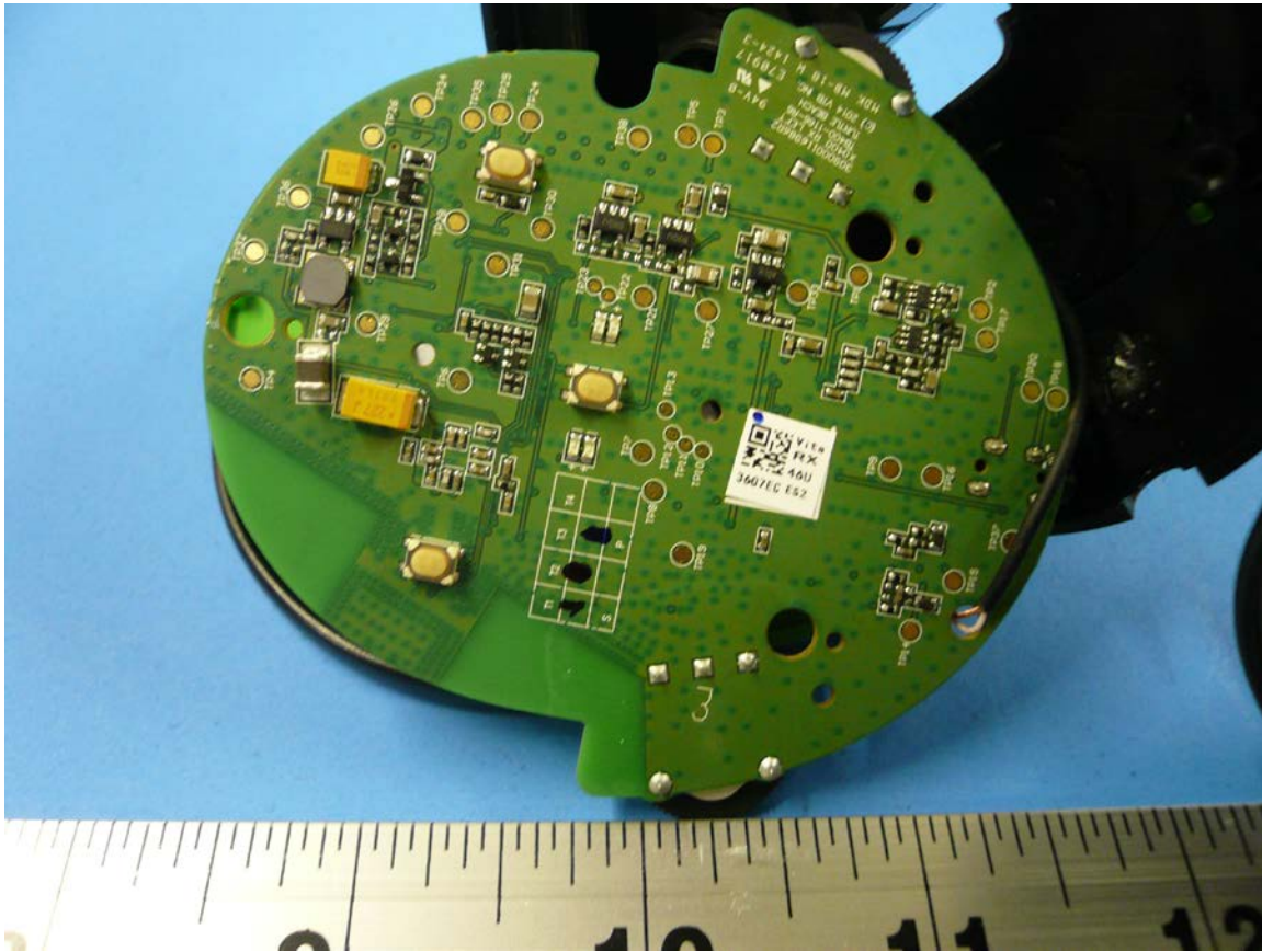
Figure 2: Internal Photo of Ear Force Stealth 500X RX - Bottom
