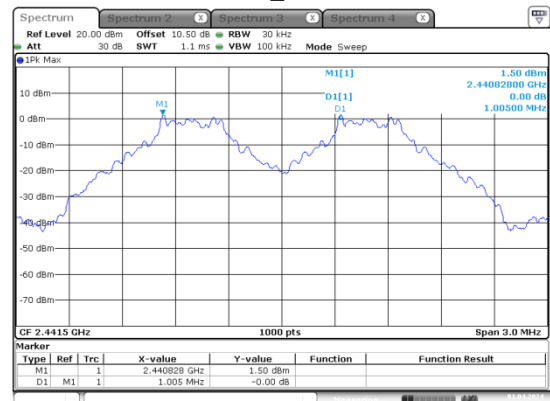
GFSK_Middle
