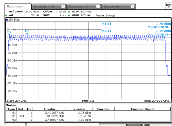
PI/4-DQPSK_Hopping_2DH1
