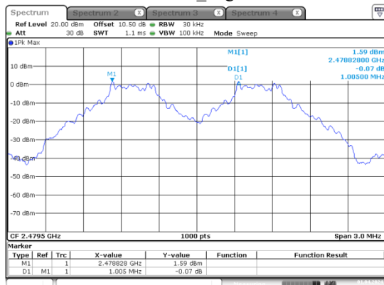
GFSK_High
