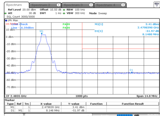
GFSK_High_DH1
