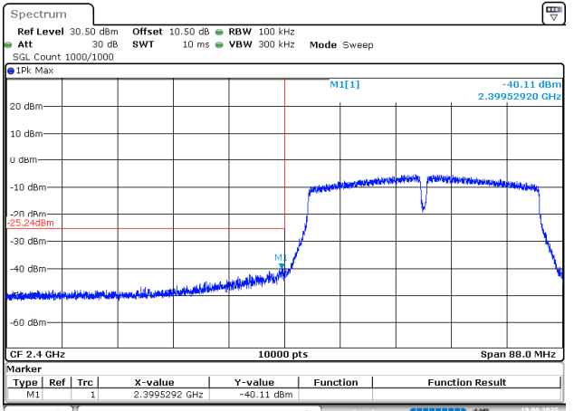
802.11n40_2422MHz
