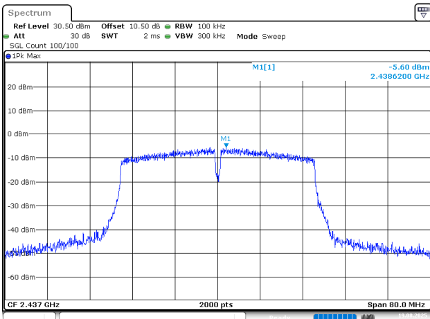
802.11n40_2437MHz
