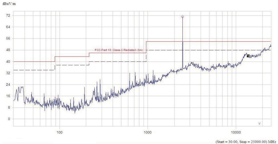
(Plot C.2: Antenna Vertical)
