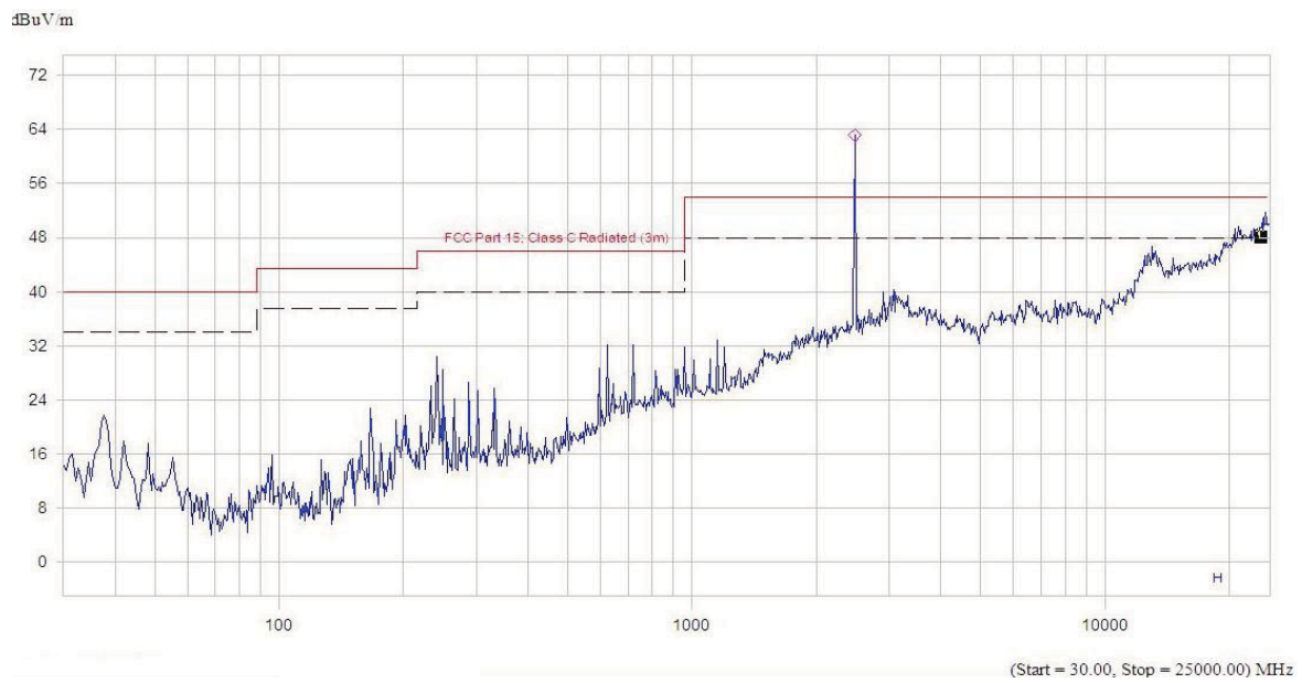
(Plot C.1: Antenna Horizontal)
