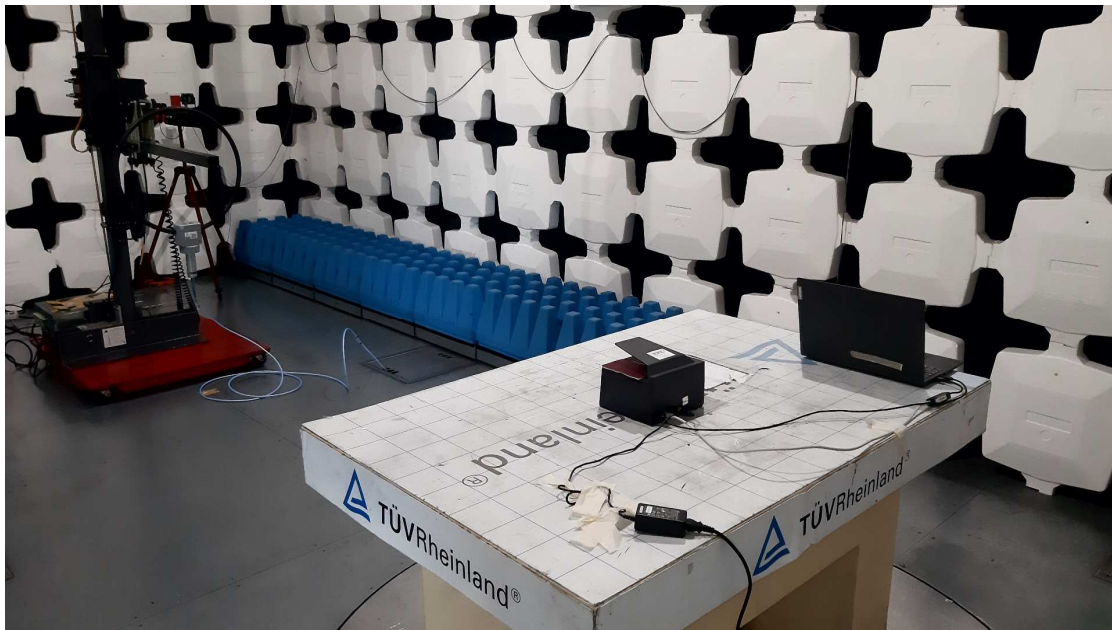
radiated emission test set-up (range 0.15-30MHz)
