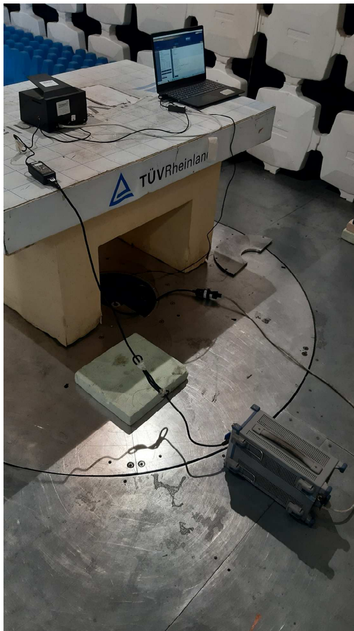
Conducted emission test set-up
