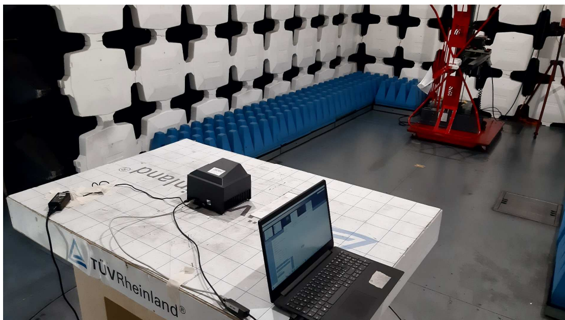
radiated emission test set-up (range 30-1000MHz)
