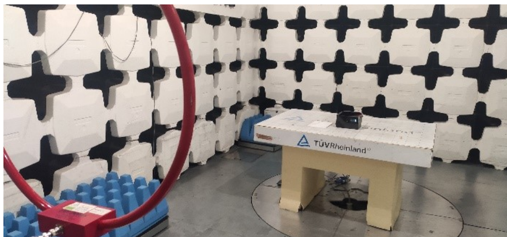
Radiated emission
