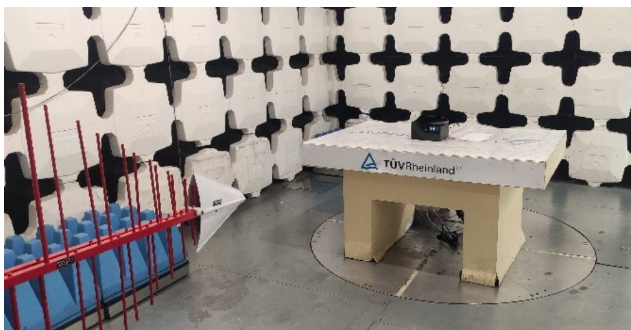
Radiated emission
