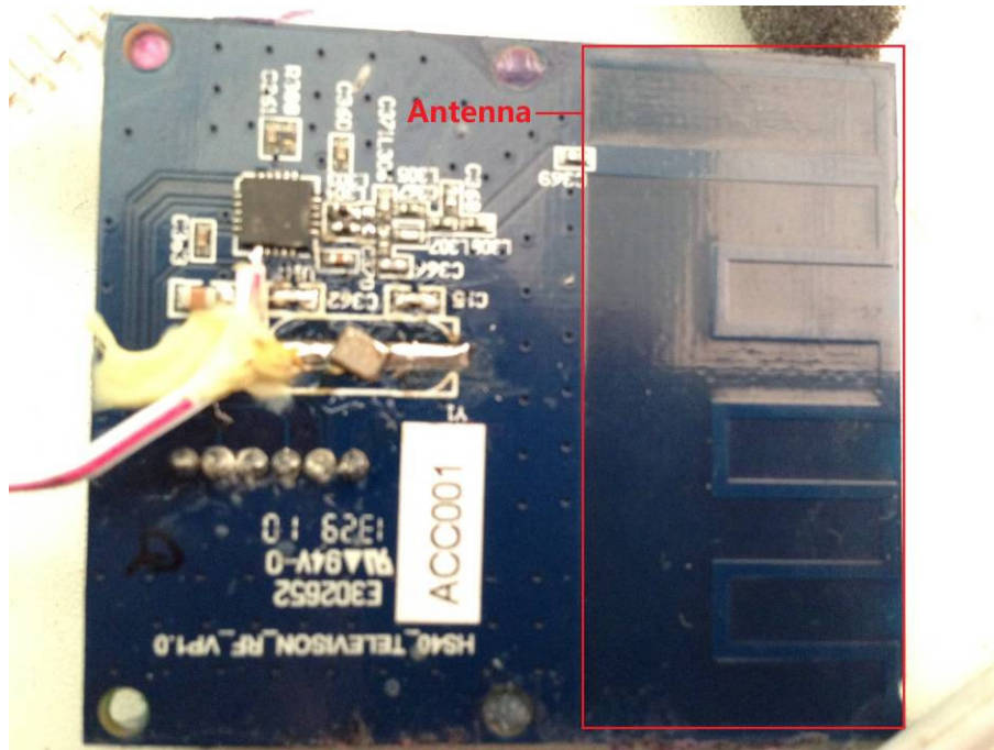
RF remote receiving board of VIFA020
