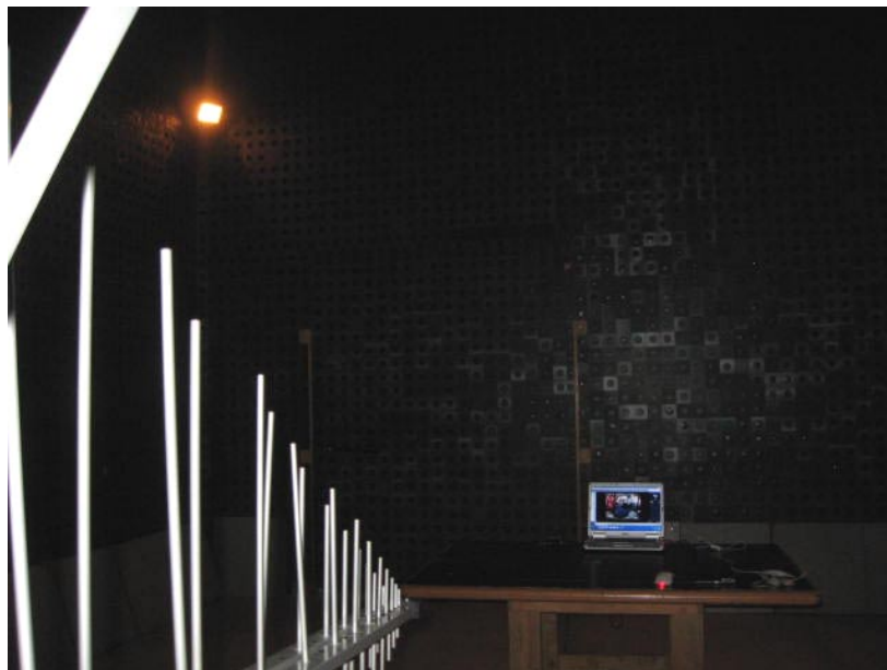
Photograph No.6 Radiated emissions measurement setup in the anechoic chamber in 30-1000 MHz range
