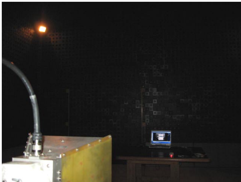
Photograph No.7 Radiated emissions measurement setup in the anechoic chamber above 1000 MHz
