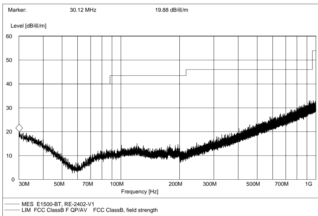
(Plot A.6: Antenna Vertical, 30MHz to 1GHz)
