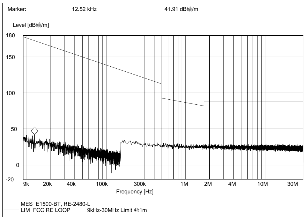
(Plot C.1: 9 kHz to 30MHz)
