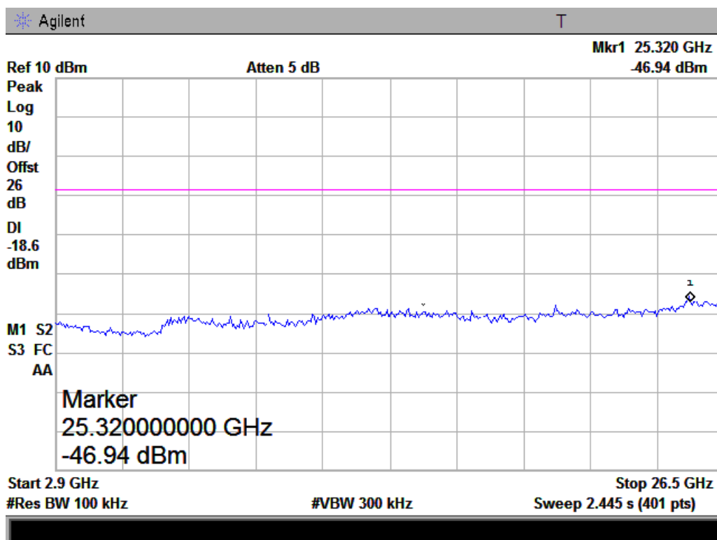
(Plot A.2: Channel = 0, 2.9GHz to 26.5GHz)
