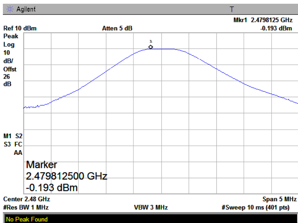
(Plot C: Channel=78)
