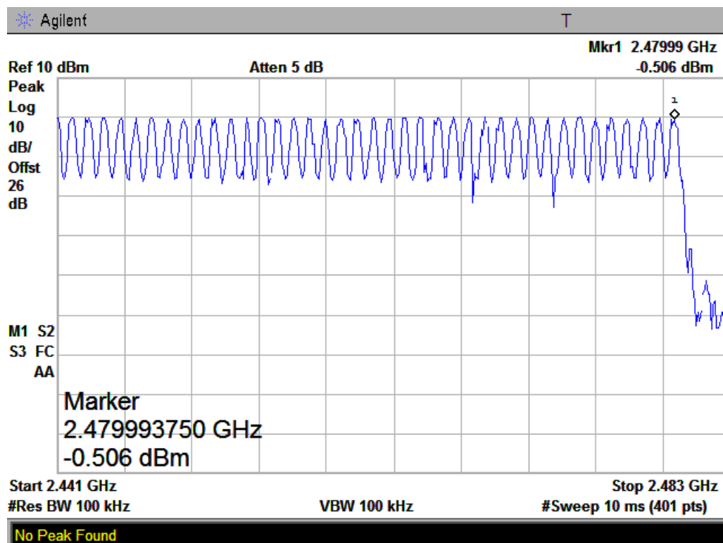
(Plot A.2: 2441MHz to 2483.5MHz)
