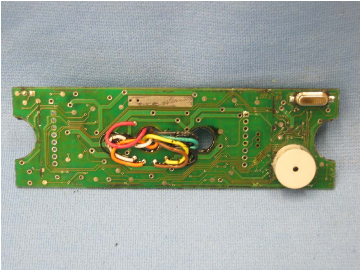
Front of main PCB
