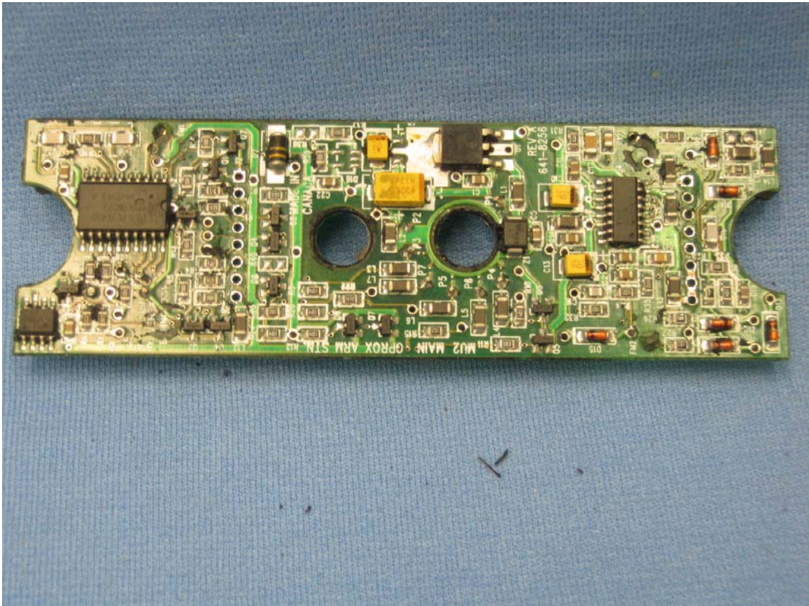
Rear of Main PCB
