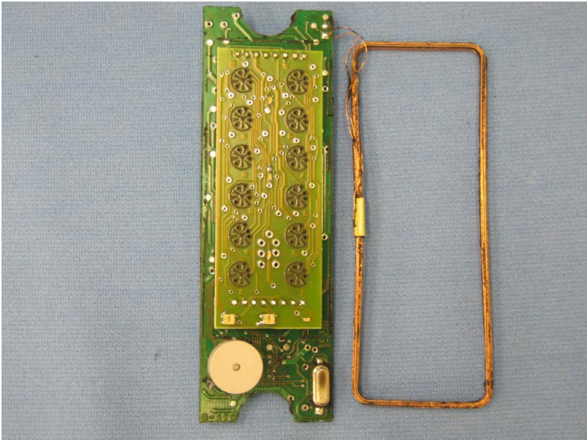
Assembly without silicone keypad
