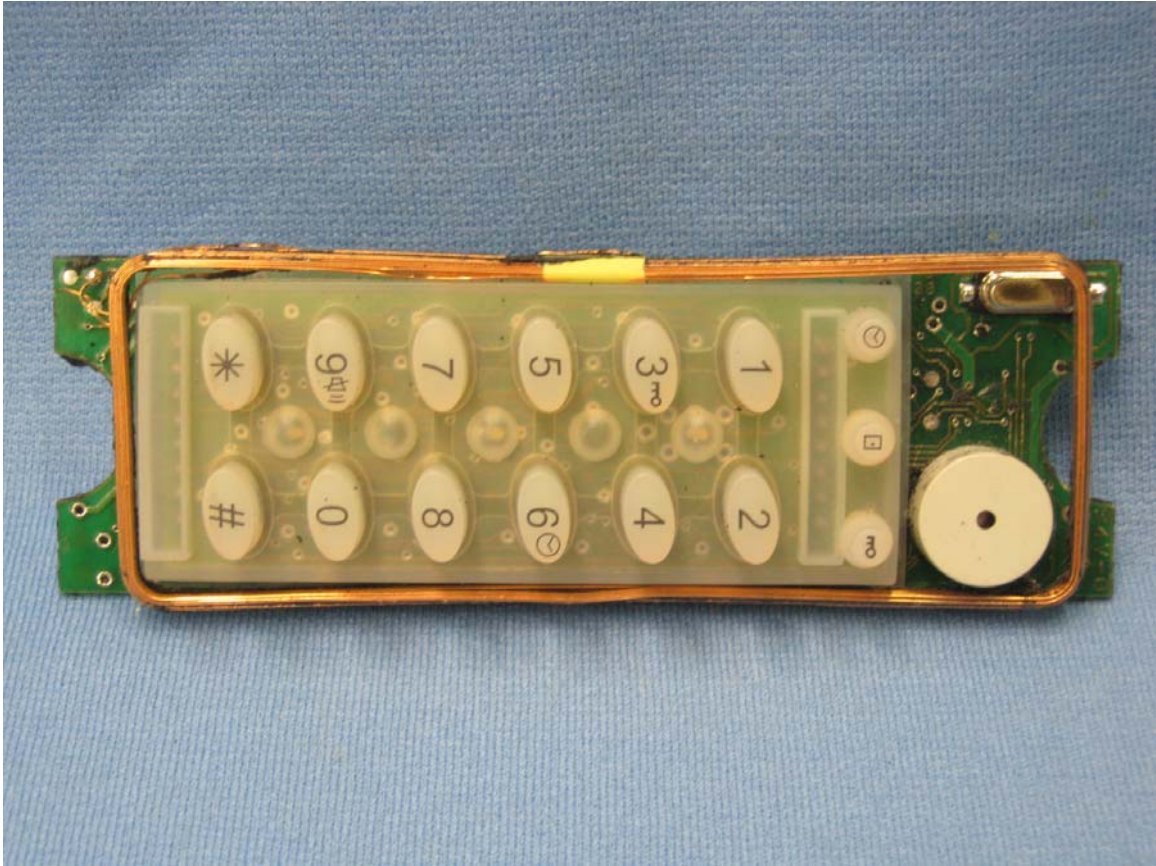
Assembly without housing or potting
