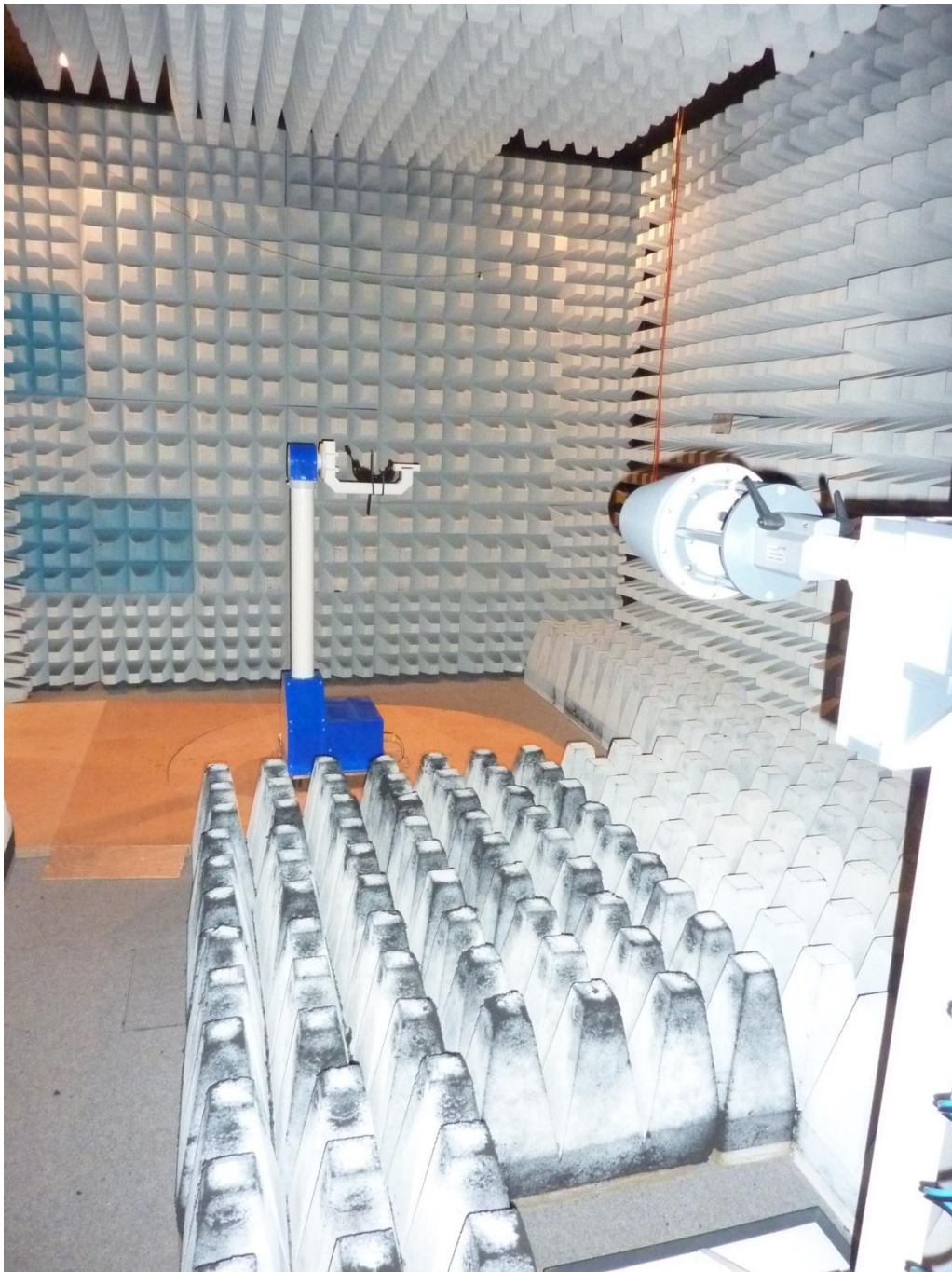
151497_n_e.JPG: FPS COM 7000, test set-up fully anechoic chamber
