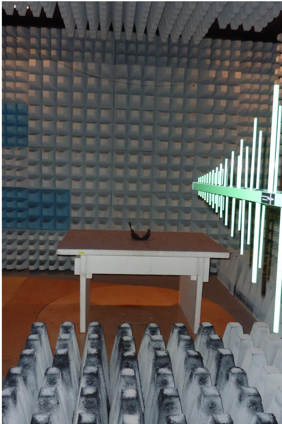
151497_n_b.JPG: FPS COM 7000, test set-up fully anechoic chamber
