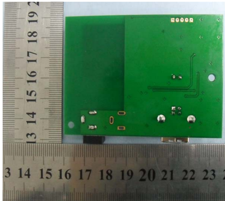
EUT - PCB View of TX part
