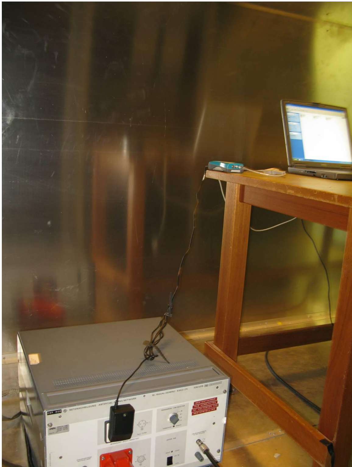
Photograph 5: - Conducted emissions test, photo 1
