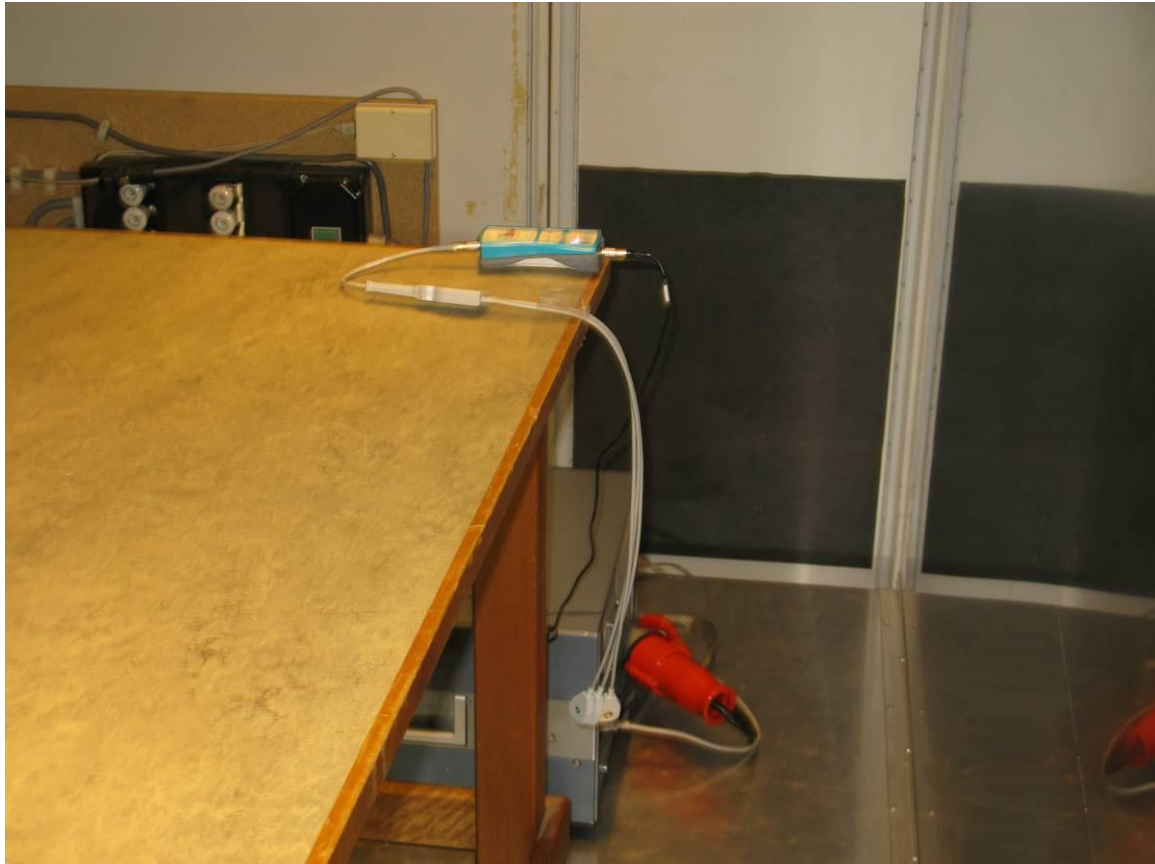
Photograph 8: - Conducted emissions test, photo 4
