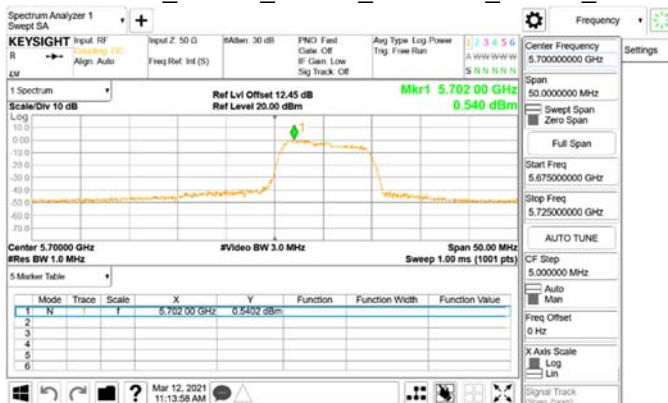
802.11ax_20MHz_Chain0_5700MHz_RU106_54
