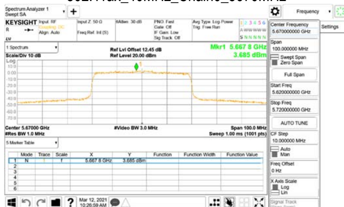
802.11ax_40MHz_Chain0_5670MHz_RU242_62
