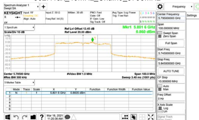
802.11ax_40MHz_Chain0_5795MHz
