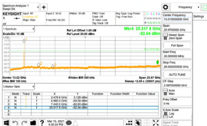
Spurious Emission_GFSK_1M_DH5_2480MHz
