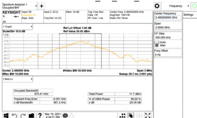
OBW 20DB GFSK_1M_DH5_2480MHz
