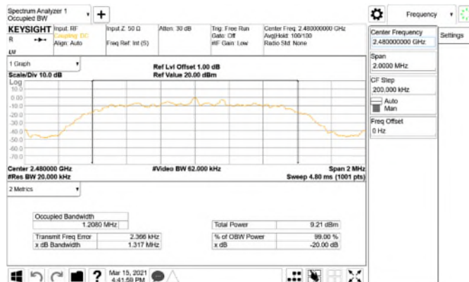
OBW 99%π/4DQPSK_2M_DH5_2480MHz
