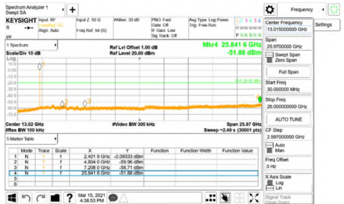
Spurious Emission_π/4DQPSK_2M_DH5_2441MHz
