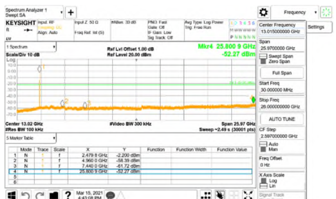
Spurious Emission_π/4DQPSK_2M_DH5_2480MHz
