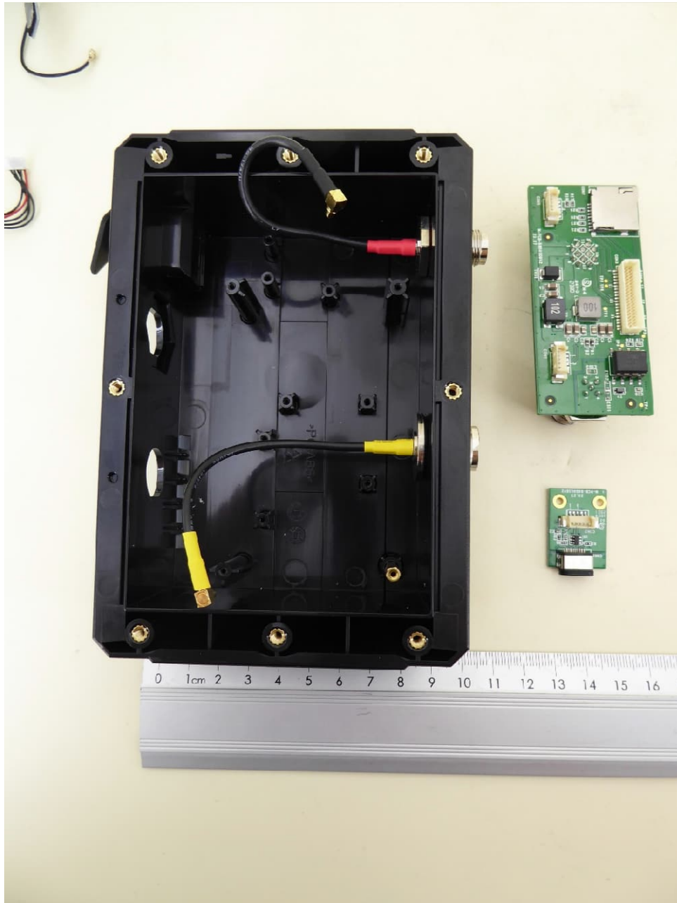
B620, internal view 3, all PCBs removed
