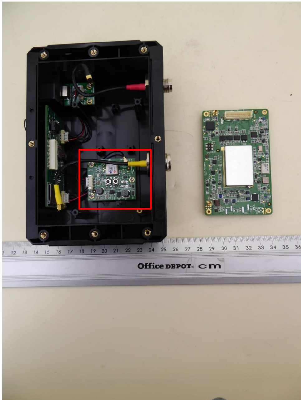
B620W (with certified Wifi Module FCC ID: WZ7-W151 / IC ID 9547A-W151), internal view 2, main PCB removed
