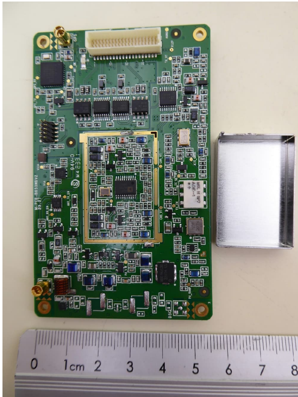
B620 / B620W, main PCB, top view, shielding removed
