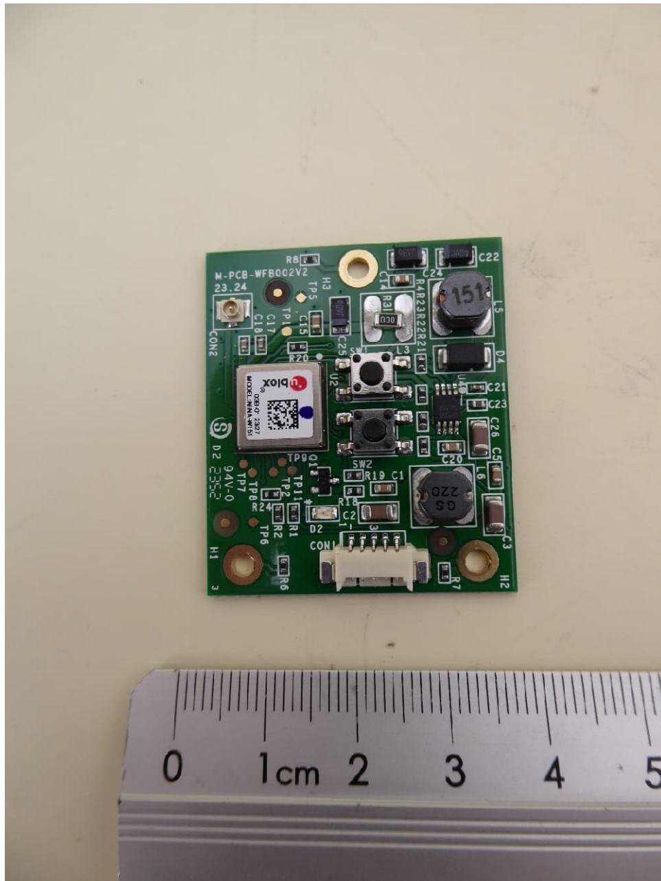
B620W, Wi-Fi module, top view
