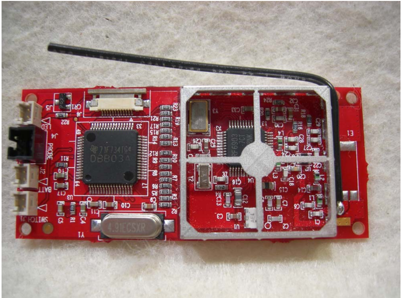
Figure 2: PCB Front without Shields
